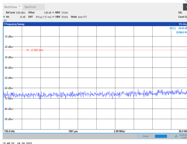
Band26-15MHz-QPSK-26865-1RB#0-Range2:0.15~30MHz
