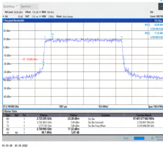
1-N78-3700-3800-30-50-M-6-CP-QPSK-Outer_Full I-33@0-Ant1-47.402-49.700-≤50-PASS
