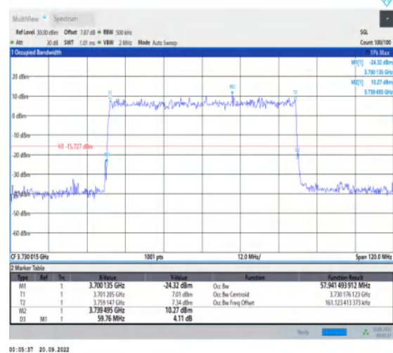
1-N78-3700-3800-30-60-L-5-DFT-256QAM-Outer_Full-162@0-Ant1-57.941-59.760-≤60-PASS
