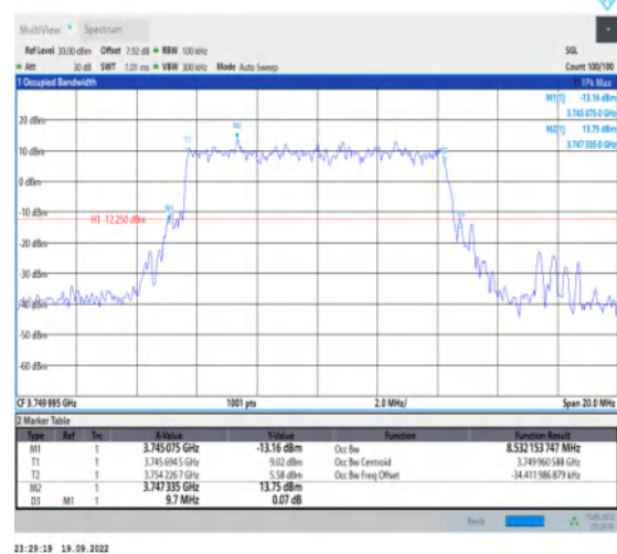
1-N78-3700-3800-30-10-M-3-DFT-16QAM-Outer_Ful l-24@0-Ant1-8.532-9.700-≤10-PASS
