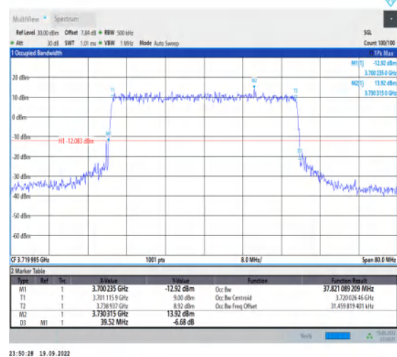
1-N78-3700-3800-30-40-L-7-CP-16QAM-Outer_Full- 106@0-Ant1-37.821-39.520-≤40-PASS
