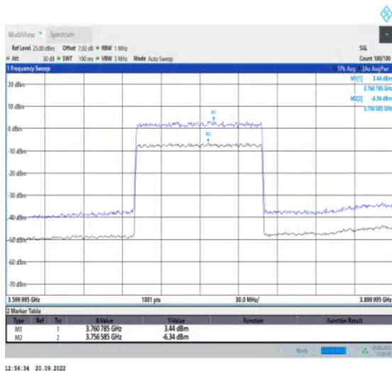
1-N78-3700-3800-30-100-M-1-DFT-256QAM-Outer_F ull-270@0-Ant1-9.78-19.56%-7.09-2.69-PASS-≤13
