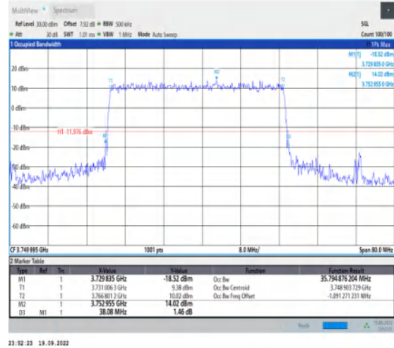
1-N78-3700-3800-30-40-M-4-DFT-64QAM-Outer_Ful I-100@0-Ant1-35.795-38.080-≤40-PASS
