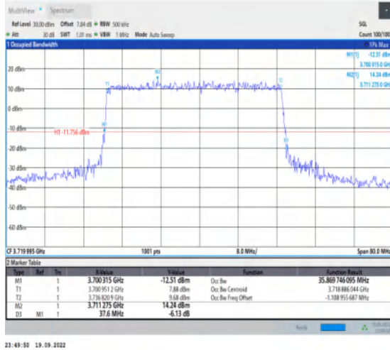
1-N78-3700-3800-30-40-L-4-DFT-64QAM-Outer_Full -100@0-Ant1-35.87-37.600-≤40-PASS
