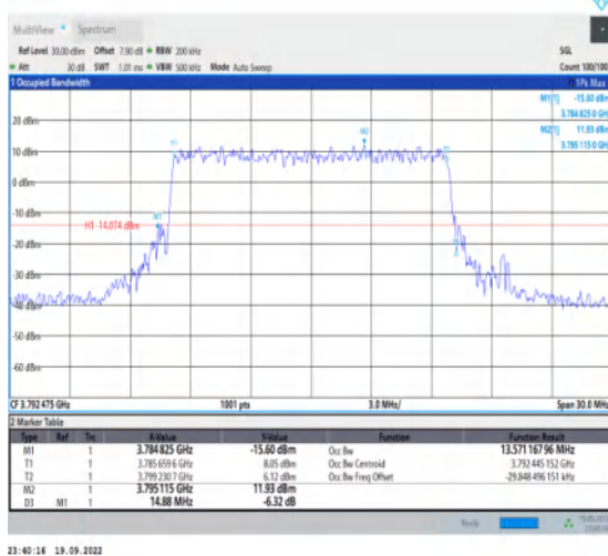
1-N78-3700-3800-30-15-H-6-CP-QPSK-Outer_Full-I-36@0-Ant1-13.571-14.880-≤15-PASS
