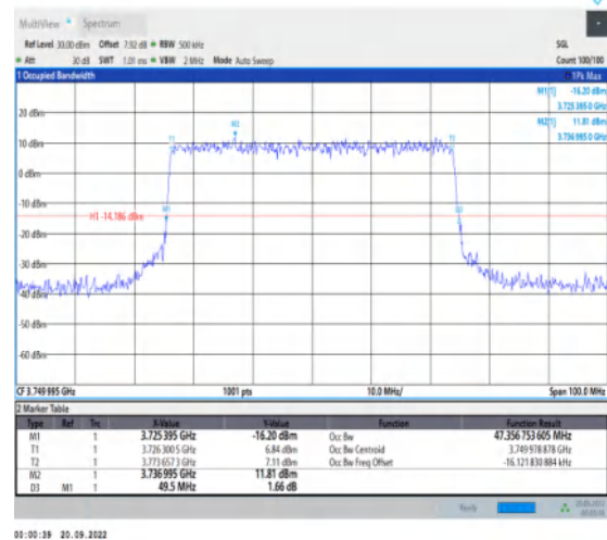
1-N78-3700-3800-30-50-M-7-CP-16QAM-Outer_Full I-133@0-Ant1-47.357-49.500-≤50-PASS
