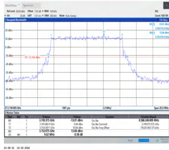
1-N78-3700-3800-30-10-M-1-DFT-QPSK-Outer_Full- 24@0-Ant1-8.586-9.620-≤10-PASS
