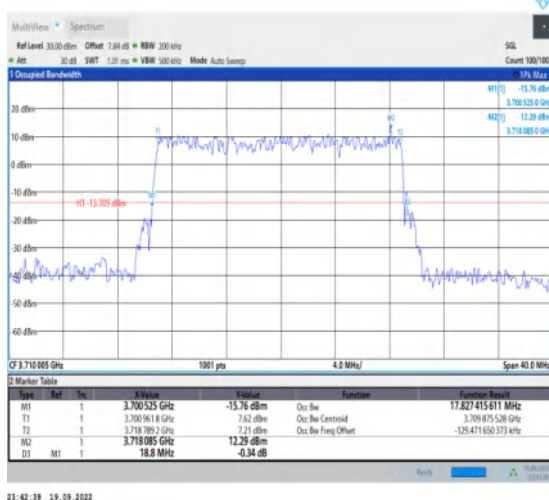
1-N78-3700-3800-30-20-L-5-DFT-256QAM-Outer_Fu II-50@0-Ant1-17.827-18.800-≤20-PASS
