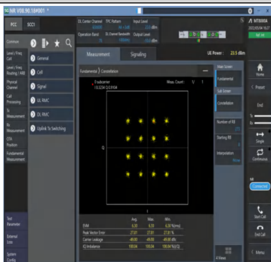
1-N78-3700-3800--30-100-M-7-CP-16QAM-Outer_Full-273@0-Ant1-see graph-PASS
