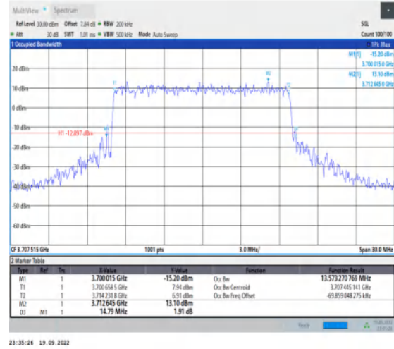
1-N78-3700-3800-30-15-L-7-CP-16QAM-Outer_Full-38@0-Ant1-13.573-14.790-≤15-PASS
