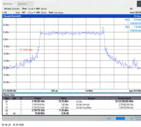
1-N78-3700-3800-30-20-M-6-CP-QPSK-Outer_Full-5 1@0-Ant1-18.136-19.480-≤20-PASS
