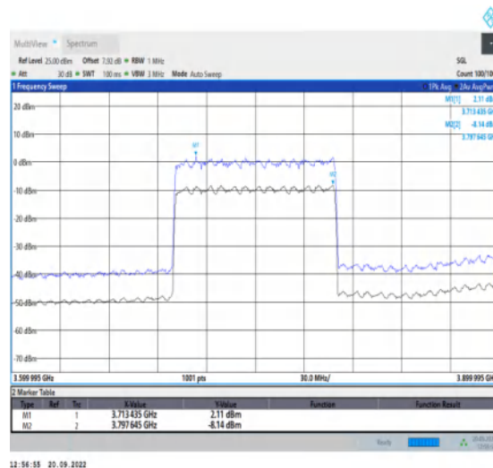
1-N78-3700-3800-30-100-M-2-CP-256QAM-Outer_F ull-273@0-Ant1-10.25-19.56%-7.09-3.16-PASS-≤13
