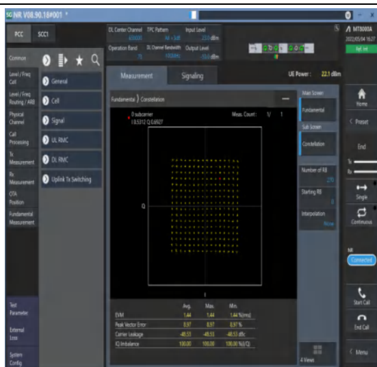
1-N78-3700-3800--30-100-M-5-DFT-256QAM-Outer_Full-270@0-Ant1-see graph-PASS
