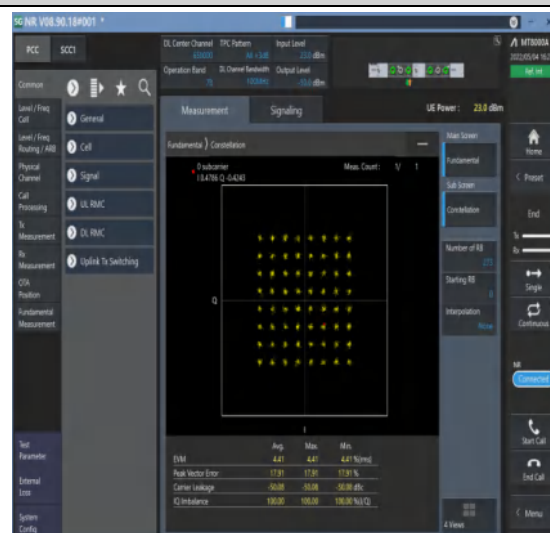
1-N78-3700-3800--30-100-M-8-CP-64QAM-Outer_Full-273@0-Ant1-see graph-PASS
