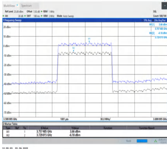
1-N78-3700-3800-30-100-L-1-DFT-256QAM-Outer_F ull-270@0-Ant1-9.84-19.56%-7.09-2.75-PASS-≤13
