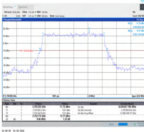
1-N78-3700-3800-30-10-M-2-DFT-PI2BPSK-Outer_F ull-24@0-Ant1-8.56-9.460-≤10-PASS
