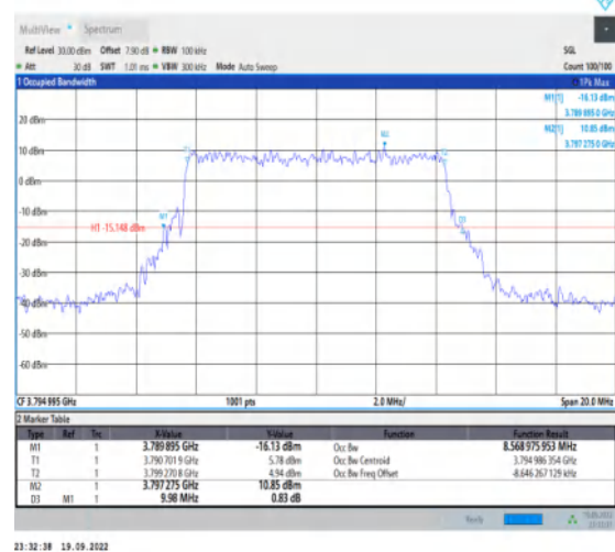
1-N78-3700-3800-30-10-H-6-CP-QPSK-Outer_Full-24@0-Ant1-8.569-9.980-≤10-PASS
