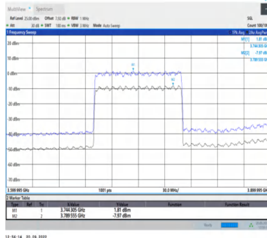
1-N78-3700-3800-30-100-L-2-CP-256QAM-Outer_F ull-273@0-Ant1-9.78-19.56%-7.09-2.69-PASS-≤13
