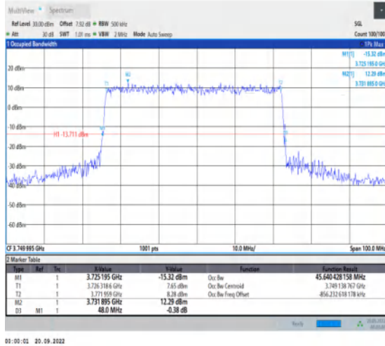
1-N78-3700-3800-30-50-M-4-DFT-64QAM-Outer_Full I-128@0-Ant1-45.64-48.000-≤50-PASS
