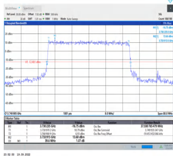
1-N78-3700-3800-30-40-M-6-CP-QPSK-Outer_Full-106@0-Ant1-37.931-39.600-≤40-PASS
