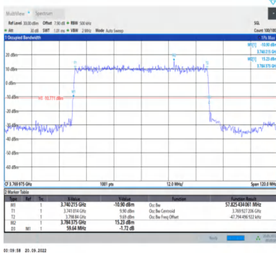
1-N78-3700-3800-30-60-H-2-DFT-PI2BPSK-Outer_Full-162@0-Ant1-57.825-59.640-≤60-PASS
