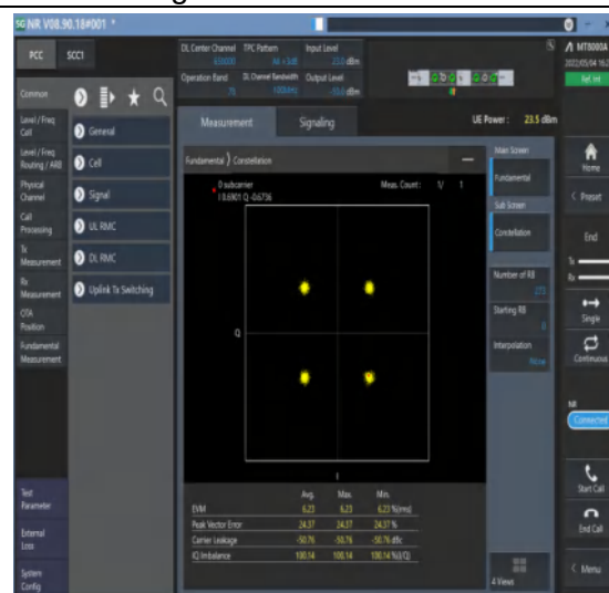
1-N78-3700-3800--30-100-M-6-CP-QPSK-Outer_Full-273@0-Ant1-see graph-PASS
