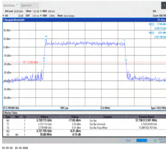
1-N78-3700-3800-30-60-M-9-CP-256QAM-Outer_Ful I-162@0-Ant1-57.797-59.880-≤60-PASS
