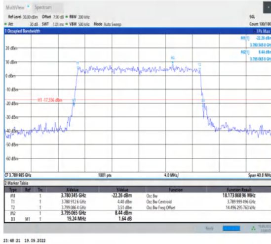
1-N78-3700-3800-30-20-H-9-CP-256QAM-Outer_Ful I-51@0-Ant1-18.174-19.240-≤20-PASS
