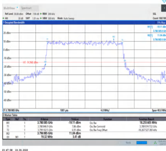
1-N78-3700-3800-30-20-H-7-CP-16QAM-Outer_Full-51@0-Ant1-18.256-19.320-≤20-PASS
