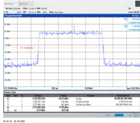
1-N78-3700-3800-30-50-M-5-DFT-256QAM-Outer_Full I-128@0-Ant1-45.693-47.900-≤50-PASS
