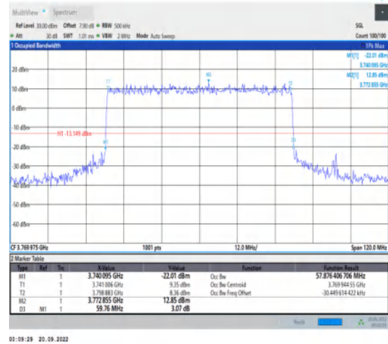
1-N78-3700-3800-30-60-H-1-DFT-QPSK-Outer_Full-162@0-Ant1-57.876-59.760-≤60-PASS
