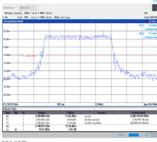
1-N78-3700-3800-30-15-H-2-DFT-PI2BPSK-Outer_Full-36@0-Ant1-12.802-14.310-≤15-PASS
