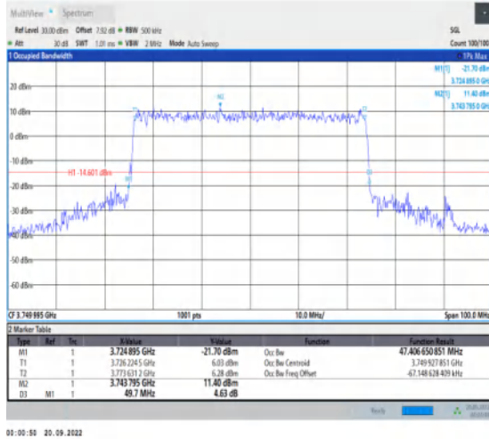
1-N78-3700-3800-30-50-M-8-CP-64QAM-Outer_Full-133@0-Ant1-47.407-49.700-≤50-PASS
