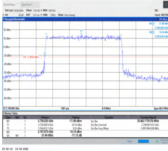
1-N78-3700-3800-30-40-M-3-DFT-16QAM-Outer_Ful I-100@0-Ant1-35.862-37.440-≤40-PASS
