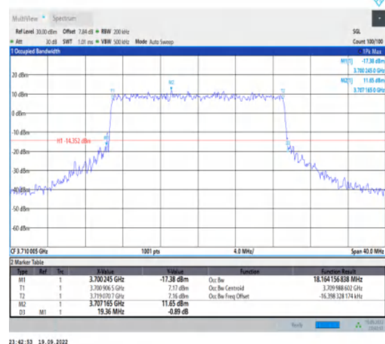
1-N78-3700-3800-30-20-L-6-CP-QPSK-Outer_Full-5 1@0-Ant1-18.164-19.360-≤20-PASS
