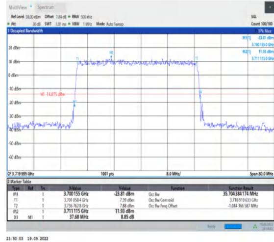
1-N78-3700-3800-30-40-L-5-DFT-256QAM-Outer_F ull-100@0-Ant1-35.704-37.680-≤40-PASS
