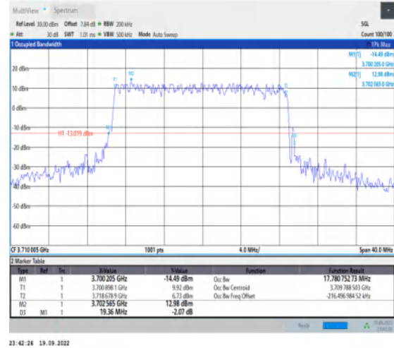
1-N78-3700-3800-30-20-L-4-DFT-64QAM-Outer_Full -50@0-Ant1-17.781-19.360-≤20-PASS
