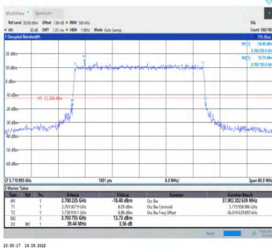
1-N78-3700-3800-30-40-L-6-CP-QPSK-Outer_Full-1 06@0-Ant1-37.902-39.440-≤40-PASS
