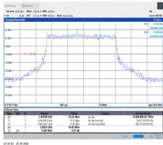
1-N78-3450-3550--30-15-L-1-DFT-QPSK-Outer_Full -36@0-Ant1-12.897-13.860≤15-PASS
