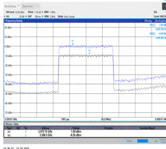
1-N78-3450-3550--30-100-L-2-CP-256QAM-Outer_Full-273@0-Ant1-10.26-100%-0.00-10.26-PASS-≤13
