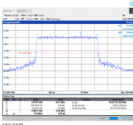
1-N78-3450-3550--30-50-M-3-DFT-16QAM-Outer_Full ull-128@0-Ant1-45.537-47.800-≤50-PASS
