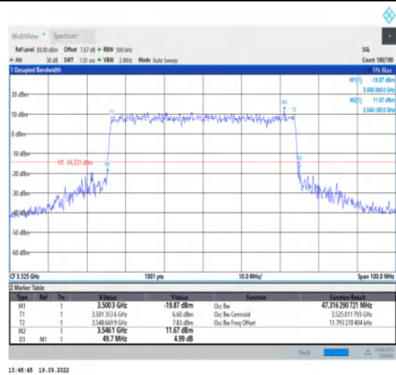
1-N78-3450-3550--30-50-H-8-CP-64QAM-Outer_Full -133@0-Ant1-47.316-49.700≤50-PASS
