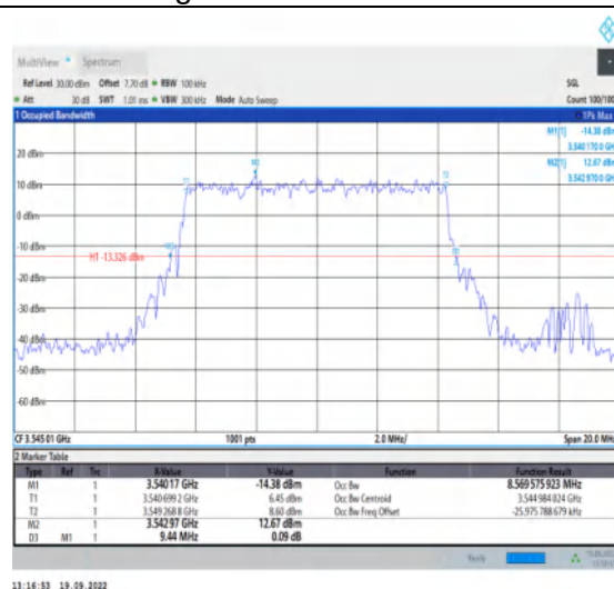
1-N78-3450-3550--30-10-H-4-DFT-64QAM-Outer_Fu II-24@0-Ant1-8.57-9.440-≤10-PASS
