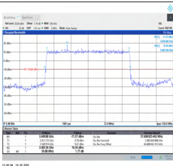
1-N78-3450-3550--30-60-L-2-DFT-PI2BPSK-Outer_Full-162@0-Ant1-57.699-59.880-≤60-PASS
