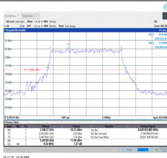
1-N78-3450-3550--30-10-H-6-CP-QPSK-Outer_Full-24@0-Ant1-8.61-9.540-≤10-PASS
