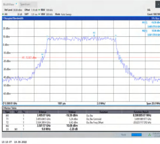
1-N78-3450-3550--30-10-M-8-CP-64QAM-Outer_Ful I-24@0-Ant1-8.599-9.800-≤10-PASS
