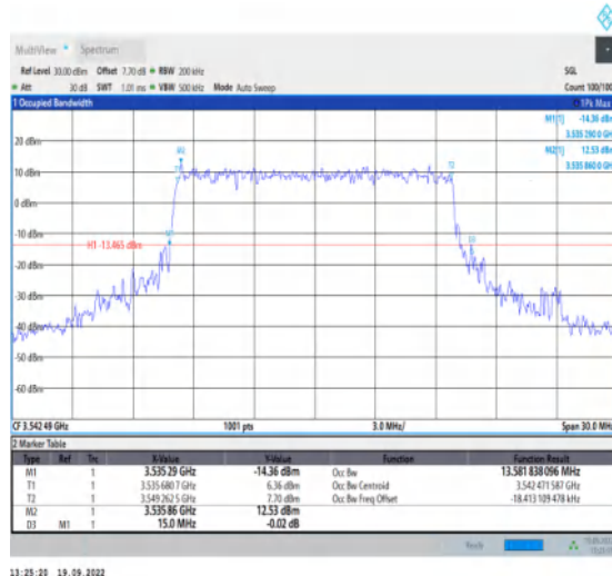
1-N78-3450-3550--30-15-H-7-CP-16QAM-Outer_Full-38@0-Ant1-13.582-15.000-≤15-PASS
