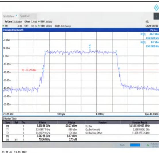
1-N78-3450-3550--30-20-H-9-CP-256QAM-Outer_Full-51@0-Ant1-18.181-19.360-≤20-PASS
