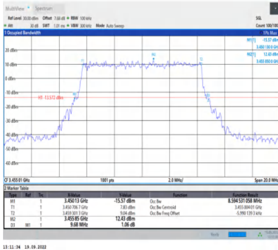
1-N78-3450-3550--30-10-L-3-DFT-16QAM-Outer_Full-24@0-Ant1-8.595-9.680-≤10-PASS
