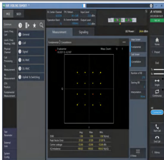
1-N78-3450-3550--30-100-M-3-DFT-16QAM-Outter_Full-270@0-Ant1-see graph-PASS
