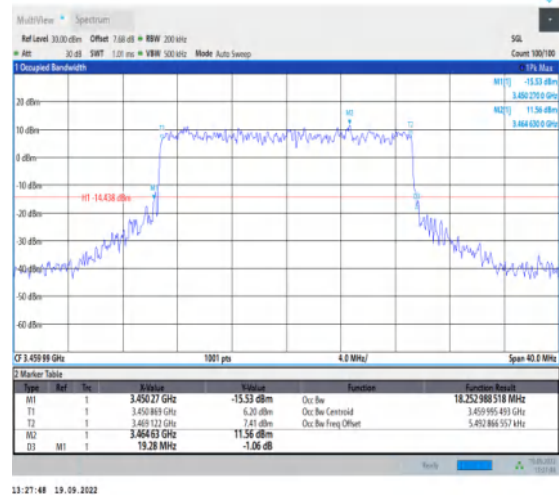
1-N78-3450-3550--30-20-L-6-CP-QPSK-Outer_Full-5 1@0-Ant1-18.253-19.280-<20-PASS
