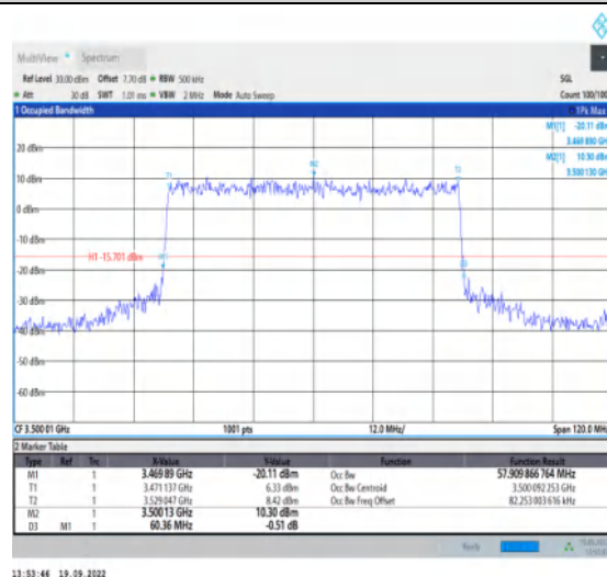
1-N78-3450-3550--30-60-M-8-CP-64QAM-Outer_Full-162@0-Ant1-57.91-60.360-≤60-PASS
