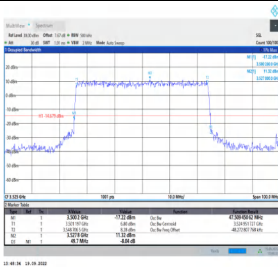
1-N78-3450-3550--30-50-H-7-CP-16QAM-Outer_Full -133@0-Ant1-47.509-49.700≤50-PASS
