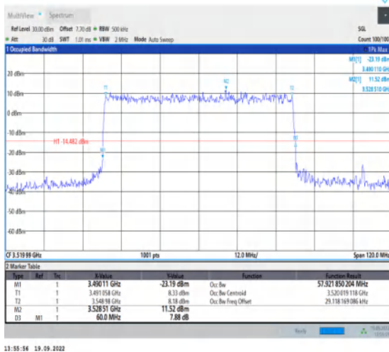
1-N78-3450-3550--30-60-H-6-CP-QPSK-Outer_Full-162@0-Ant1-57.922-60.000-≤60-PASS
