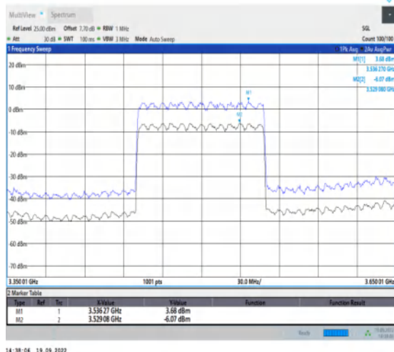
1-N78-3450-3550--30-100-L-1-DFT-256QAM-Outer_Full-270@0-Ant1-9.75-100%-0.00-9.75-PASS-≤13
