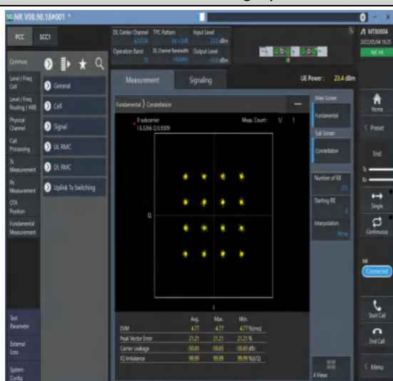
1-N78-3450-3550--30-100-M-7-CP-16QAM-Outer_Fu ll-273@0-Ant1-see graph-PASS
