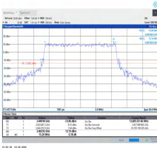
1-N78-3450-3550--30-15-L-8-CP-64QAM-Outet_Full-38@0-Ant1-13.605-15.240-≤15-PASS
