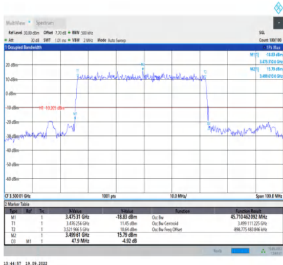
1-N78-3450-3550--30-50-M-2-DFT-PI2BPSK-Outer_Full Full-128@0-Ant1-45.71-47.900-≤50-PASS
