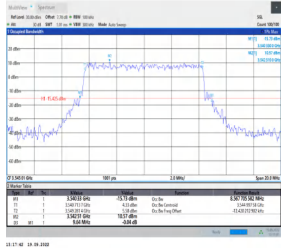
1-N78-3450-3550--30-10-H-8-CP-64QAM-Outer_Full -24@0-Ant1-8.568-9.640≤10-PASS
