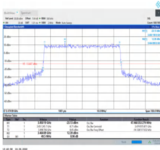
1-N78-3450-3550--30-50-L-8-CP-64QAM-Outer_Full-133@0-Ant1-47.46-49.500-≤50-PASS
