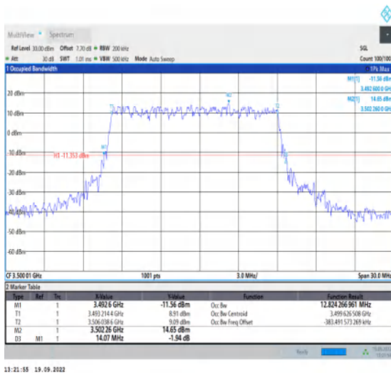
1-N78-3450-3550--30-15-M-3-DFT-16QAM-Outer_Full -36@0-Ant1-12.824-14.070≤15-PASS
