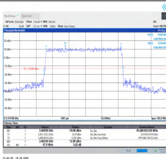
1-N78-3450-3550--30-50-L-4-DFT-64QAM-Outer_Full-128@0-Ant1-45.6-47.900-≤50-PASS
