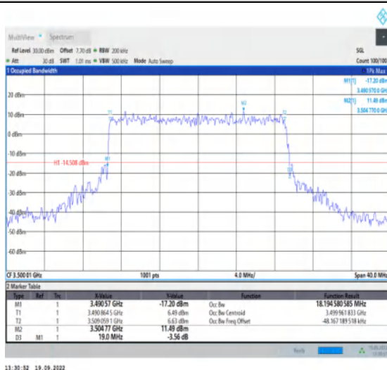
1-N78-3450-3550--30-20-M-8-CP-64QAM-Outer_Full-51@0-Ant1-18.195-19.000-≤20-PASS
