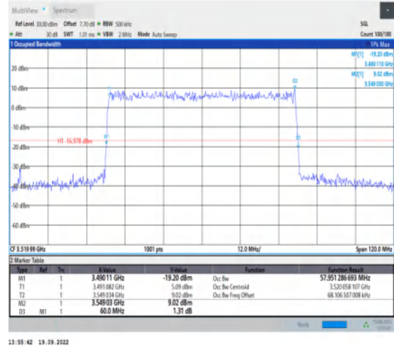
1-N78-3450-3550--30-60-H-5-DFT-256QAM-Outer_F ull-162@0-Ant1-57.951-60.000-≤60-PASS
