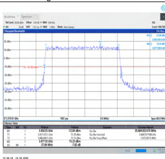
1-N78-3450-3550--30-40-L-1-DFT-QPSK-Outer_Full-100@0-Ant1-35.805-37.840-≤40-PASS
