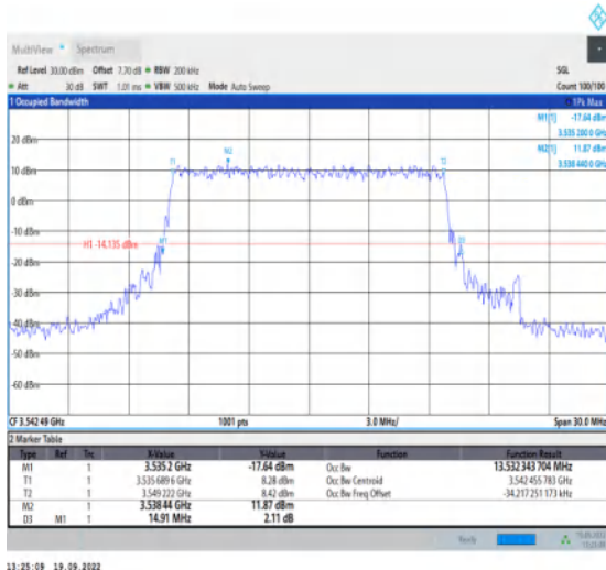
1-N78-3450-3550--30-15-H-6-CP-QPSK-Outer_Full-38@0-Ant1-13.532-14.910-≤15-PASS
