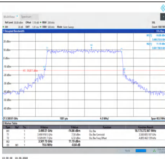
1-N78-3450-3550--30-20-M-6-CP-QPSK-Outer_Full-51@0-Ant1-18.173-19.600-≤20-PASS
