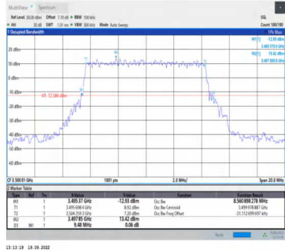
1-N78-3450-3550--30-10-M-1-DFT-QPSK-Outer_Full -24@0-Ant1-8.561-9.480-≤10-PASS
