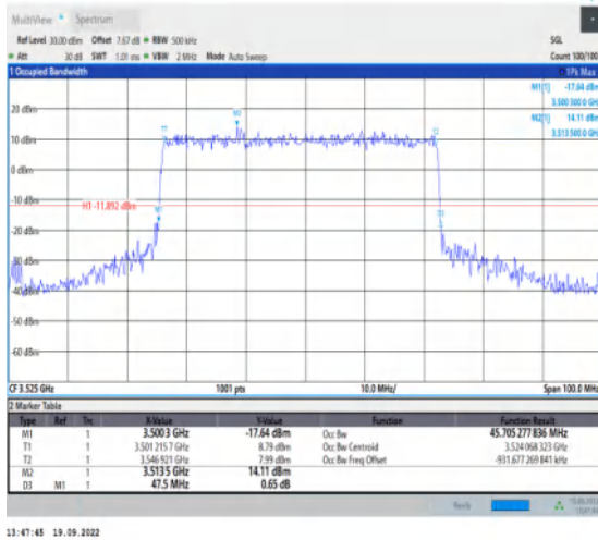
1-N78-3450-3550--30-50-H-3-DFT-16QAM-Outer_Fu II-128@0-Ant1-45.705-47.500-≤50-PASS
