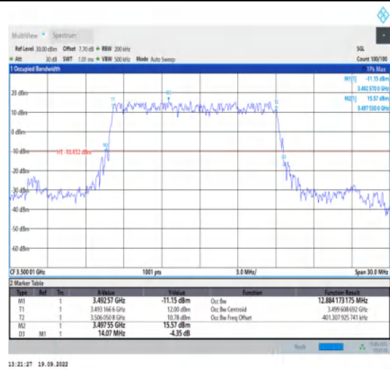
1-N78-3450-3550--30-15-M-2-DFT-PI2BPSK-Outer_Full -36@0-Ant1-12.884-14.070≤15-PASS
