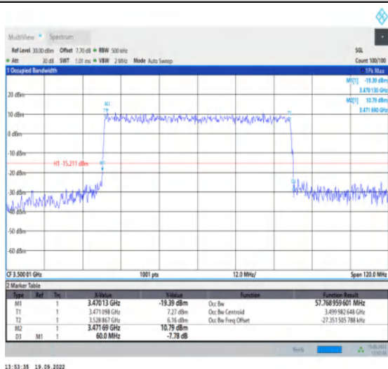
1-N78-3450-3550--30-60-M-7-CP-16QAM-Outer_Ful I-162@0-Ant1-57.769-60.000-≤60-PASS
