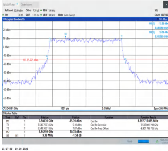
1-N78-3450-3550--30-10-H-7-CP-16QAM-Outer_Full -24@0-Ant1-8.598-9.380≤10-PASS
