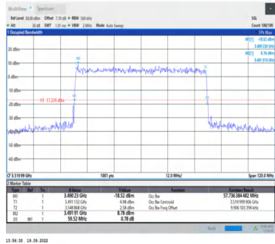
1-N78-3450-3550--30-60-H-9-CP-256QAM-Outer_Fu ll-162@0-Ant1-57.736-59.520-≤60-PASS
