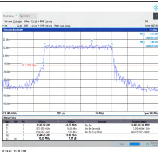
1-N78-3450-3550--30-15-H-4-DFT-64QAM-Outer_Fu ll-36@0-Ant1-12.864-13.650-≤15-PASS
