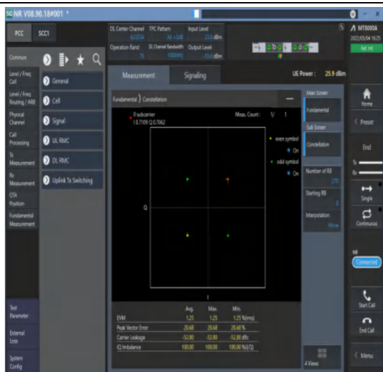
1-N78-3450-3550--30-100-M-1-DFT-PI2BPSK-Outter_Full-270@0-Ant1-see graph-PASS
