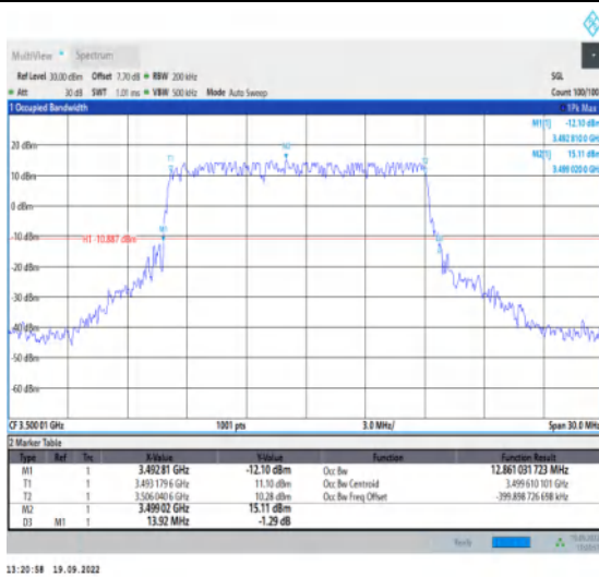
1-N78-3450-3550--30-15-M-1-DFT-QPSK-Outer_Full -36@0-Ant1-12.861-13.920≤15-PASS
