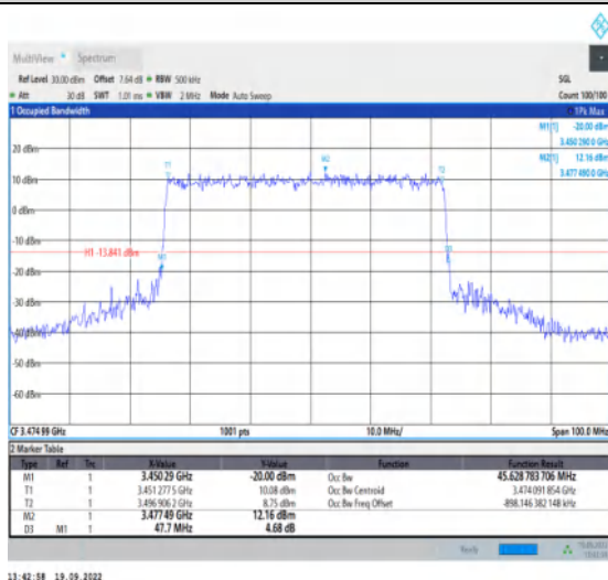
1-N78-3450-3550--30-50-L-3-DFT-16QAM-Outer_Full-128@0-Ant1-45.629-47.700-≤50-PASS
