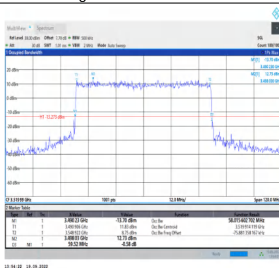
1-N78-3450-3550--30-60-H-1-DFT-QPSK-Outer_Full-162@0-Ant1-58.016-59.520-≤60-PASS
