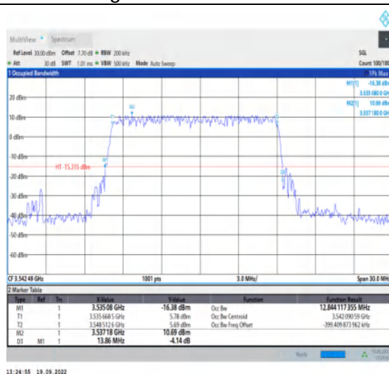
1-N78-3450-3550--30-15-H-5-DFT-256QAM-Outer_F ull-36@0-Ant1-12.844-13.860-≤15-PASS
