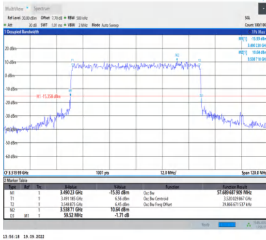
1-N78-3450-3550--30-60-H-8-CP-64QAM-Outer_Full -162@0-Ant1-57.69-59.520-≤60-PASS
