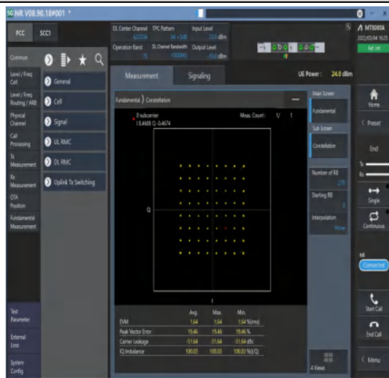
1-N78-3450-3550--30-100-M-4-DFT-64QAM-Outter_Full-270@0-Ant1-see graph-PASS
