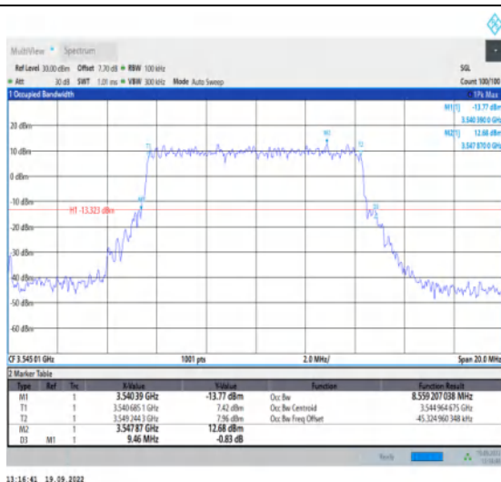
1-N78-3450-3550--30-10-H-3-DFT-16QAM-Outer_Fu II-24@0-Ant1-8.559-9.460-≤10-PASS
