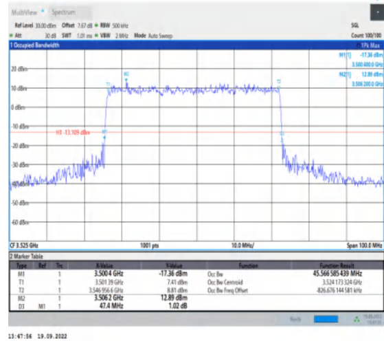
1-N78-3450-3550--30-50-H-4-DFT-64QAM-Outer_Fu II-128@0-Ant1-45.567-47.400-≤50-PASS
