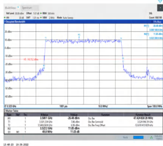
1-N78-3450-3550--30-50-H-6-CP-QPSK-Outer_Full- 133@0-Ant1-47.425-49.800-≤50-PASS
