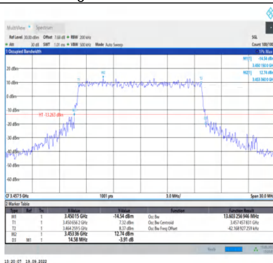
1-N78-3450-3550--30-15-L-7-CP-16QAM-Outet_Full-38@0-Ant1-13.603-14.580-≤15-PASS
