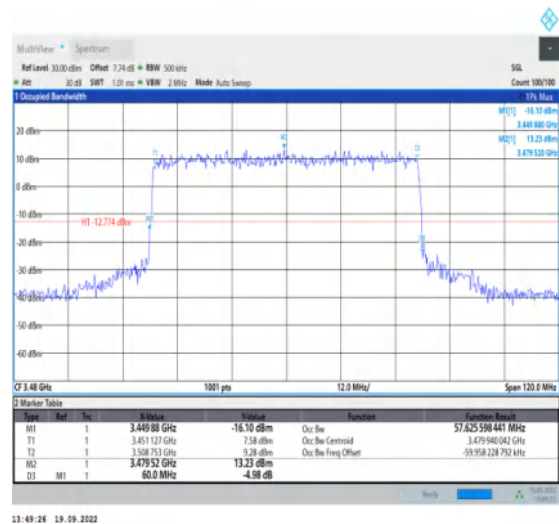
1-N78-3450-3550--30-60-L-1-DFT-QPSK-Outer_Full -162@0-Ant1-57.626-60.000≤60-PASS
