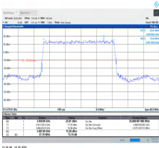
1-N78-3450-3550--30-40-L-2-DFT-PI2BPSK-Outer_Full-100@0-Ant1-35.808-37.760-≤40-PASS
