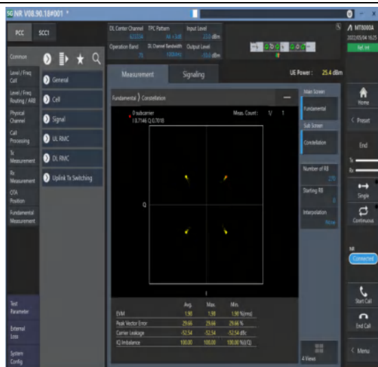
1-N78-3450-3550--30-100-M-2-DFT-QPSK-Outter_Full-270@0-Ant1-see graph-PASS
