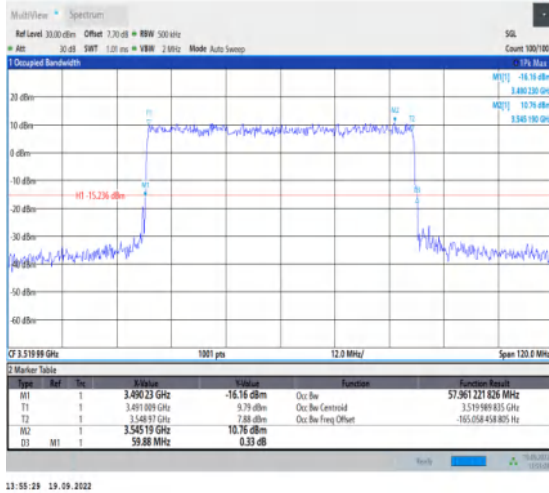
1-N78-3450-3550--30-60-H-4-DFT-64QAM-Outer_Fu II-162@0-Ant1-57.961-59.880-≤60-PASS
