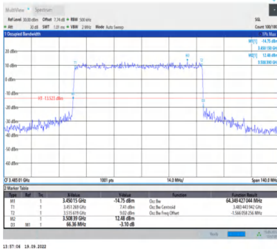
1-N78-3450-3550--30-70-L-1-DFT-QPSK-Outer_Full- 180@0-Ant1-64.349-66.360-≤70-PASS
