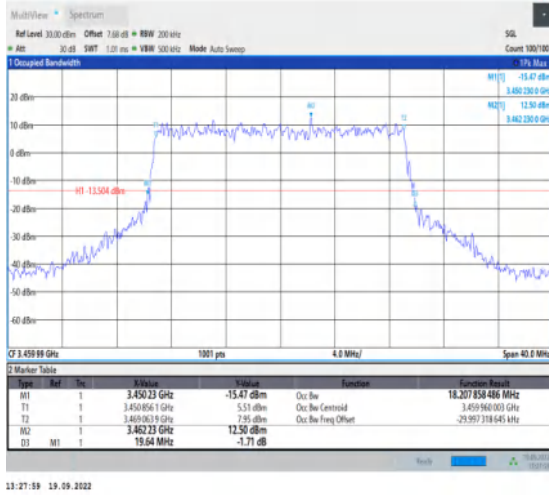
1-N78-3450-3550--30-20-L-7-CP-16QAM-Outer_Full -51@0-Ant1-18.208-19.640-≤20-PASS
