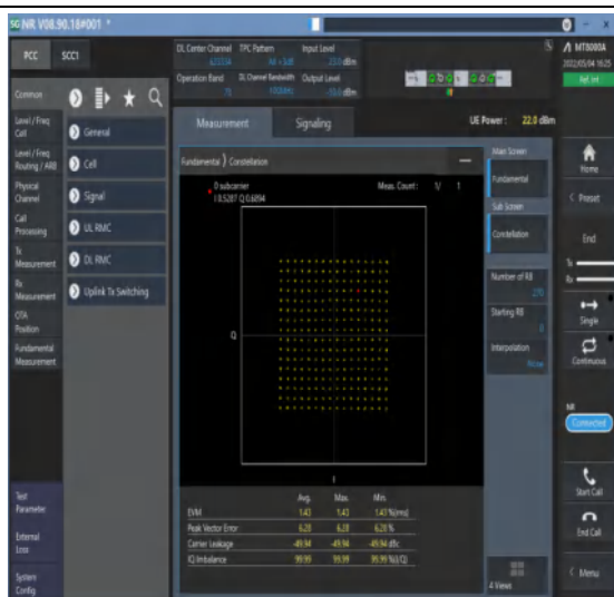
1-N78-3450-3550--30-100-M-5-DFT-256QAM-Outer_Fu Full-270@0-Ant1-see graph-PASS
