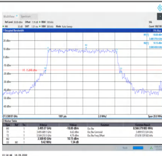
1-N78-3450-3550--30-10-M-6-CP-QPSK-Outer_Full-24@0-Ant1-8.566-9.420≤10-PASS
