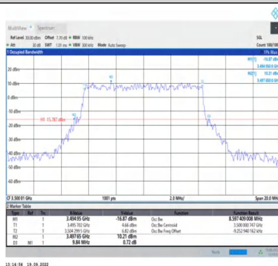
1-N78-3450-3550--30-10-M-7-CP-16QAM-Outer_Full-24@0-Ant1-8.597-9.840≤10-PASS
