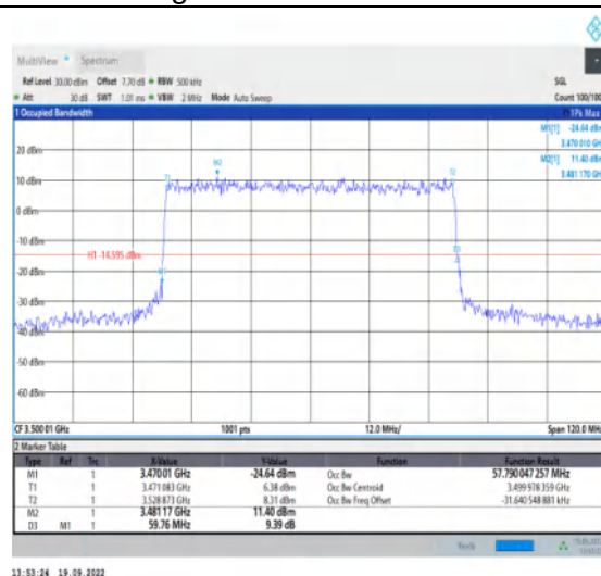
1-N78-3450-3550--30-60-M-6-CP-QPSK-Outer_Full-162@0-Ant1-57.79-59.760-≤60-PASS
