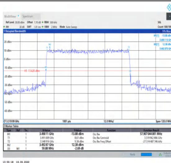
1-N78-3450-3550--30-60-H-3-DFT-16QAM-Outer_Full-162@0-Ant1-57.907-59.880-≤60-PASS
