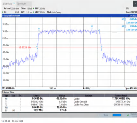
1-N78-3450-3550--30-20-L-3-DFT-16QAM-Outer_Fu ll-50@0-Ant1-17.785-18.920-<20-PASS
