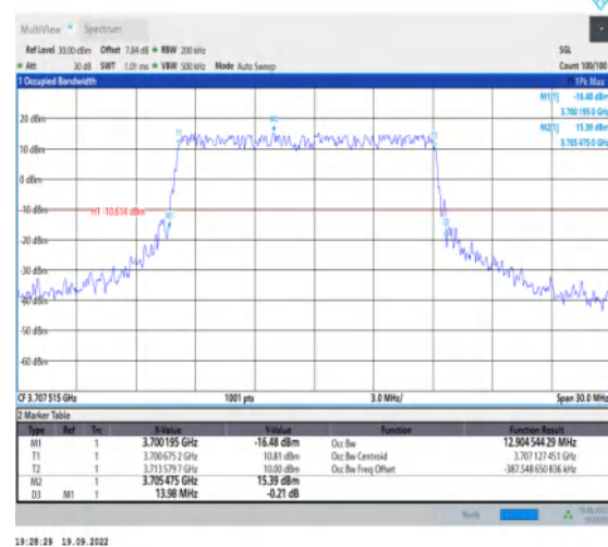
1-N77-3700-3980--30-15-L-1-DFT-QPSK-Outer_Full- 36@0-Ant1-12.905-13.980-≤15-PASS
