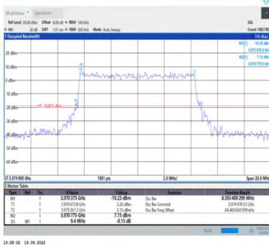
1-N77-3700-3980--30-10-H-9-CP-256QAM-Outer_F ull-24@0-Ant1-8.593-9.400-≤10-PASS
