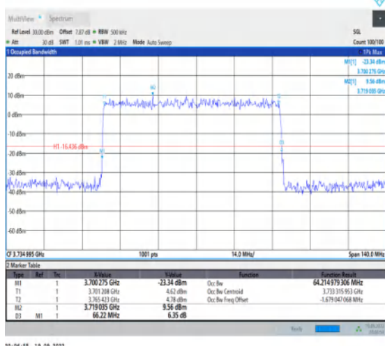
1-N77-3700-3980--30-70-L-5-DFT-256QAM-Outer_F ull-180@0-Ant1-64.215-66.220-≤70-PASS
