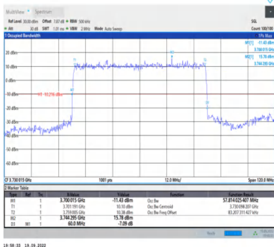
1-N77-3700-3980--30-60-L-2-DFT-PI2BPSK-Outer_Full-162@0-Ant1-57.814-60.000-≤60-PASS
