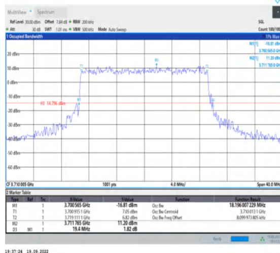
1-N77-3700-3980--30-20-L-8-CP-64QAM-Outer_Full- 51@0-Ant1-18.196-19.400-≤20-PASS
