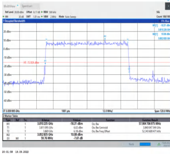
1-N77-3700-3980--30-60-M-5-DFT-256QAM-Outer_Full-162@0-Ant1-57.905-59.760-≤60-PASS
