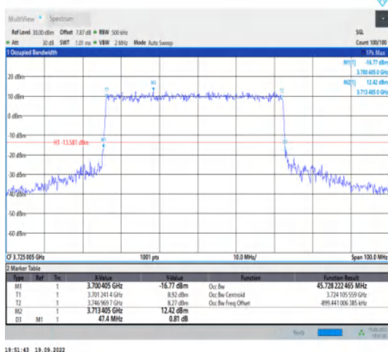
1-N77-3700-3980--30-50-L-3-DFT-16QAM-Outer_Fu ll-128@0-Ant1-45.728-47.400-≤50-PASS
