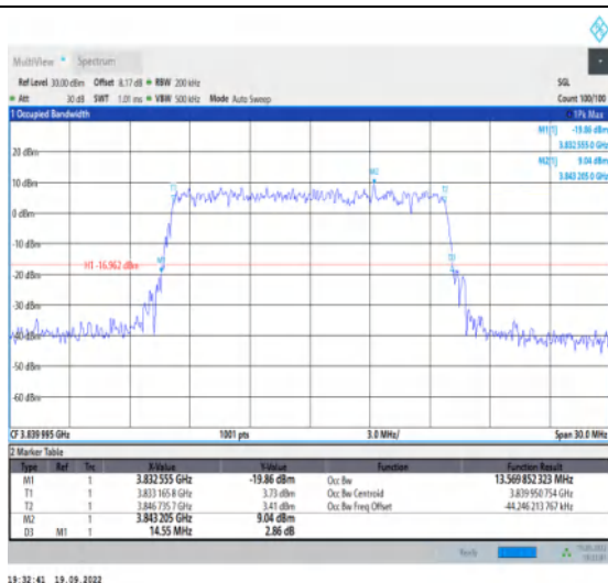
1-N77-3700-3980--30-15-M-9-CP-256QAM-Outer_Full-38@0-Ant1-13.57-14.550-≤15-PASS
