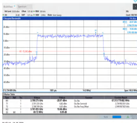
1-N77-3700-3980--30-70-L-6-CP-QPSK-Outer_Full-189@0-Ant1-67.514-69.720-≤70-PASS
