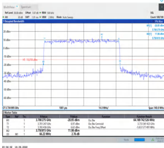
1-N77-3700-3980--30-70-L-3-DFT-16QAM-Outer_Fu ll-180@0-Ant1-64.19-66.220-≤70-PASS
