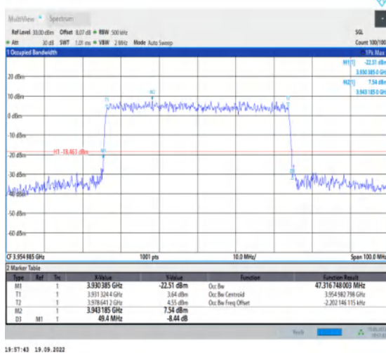
1-N77-3700-3980--30-50-H-9-CP-256QAM-Outer_Full -133@0-Ant1-47.317-49.400-≤50-PASS
