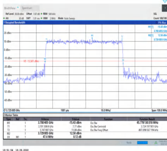
1-N77-3700-3980--30-50-L-4-DFT-64QAM-Outer_Ful l-128@0-Ant1-45.778-47.400-≤50-PASS
