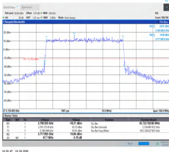
1-N77-3700-3980--30-50-L-1-DFT-QPSK-Outer_Full -128@0-Ant1-45.732-47.700-≤50-PASS
