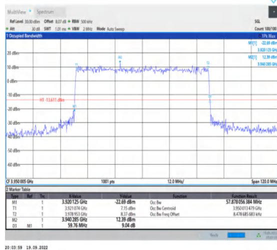
1-N77-3700-3980--30-60-H-3-DFT-16QAM-Outer_Full-162@0-Ant1-57.878-59.760-≤60-PASS
