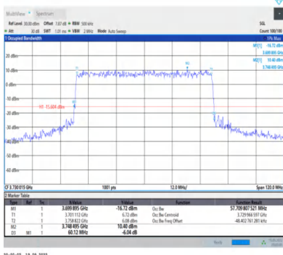
1-N77-3700-3980--30-60-L-8-CP-64QAM-Outer_Full-162@0-Ant1-57.71-60.120-≤60-PASS
