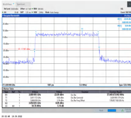
1-N77-3700-3980--30-60-M-9-CP-256QAM-Outer_Full-162@0-Ant1-57.646-59.760-≤60-PASS
