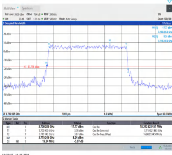
1-N77-3700-3980--30-20-L-9-CP-256QAM-Outer_F ull-51@0-Ant1-18.243-19.240-≤20-PASS
