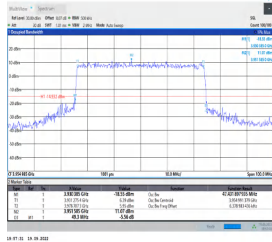
1-N77-3700-3980--30-50-H-8-CP-64QAM-Outer_Full -133@0-Ant1-47.432-49.300-≤50-PASS
