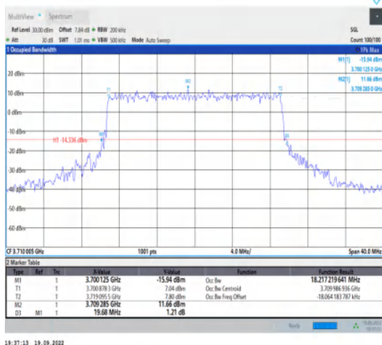
1-N77-3700-3980--30-20-L-7-CP-16QAM-Outer_Full -51@0-Ant1-18.217-19.680-≤20-PASS
