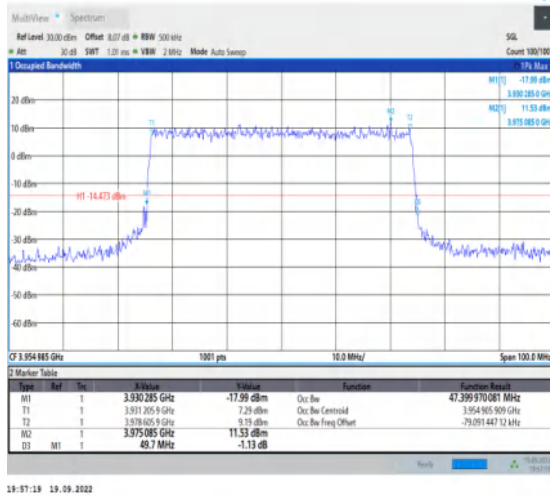
1-N77-3700-3980--30-50-H-7-CP-16QAM-Outer_Full I-133@0-Ant1-47.4-49.700-≤50-PASS
