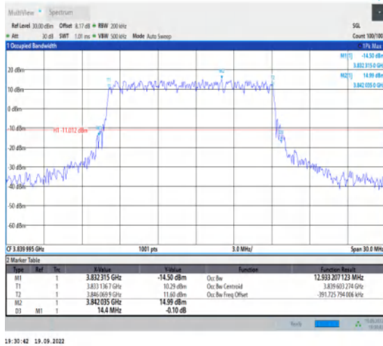
1-N77-3700-3980--30-15-M-1-DFT-QPSK-Outer_Ful I-36@0-Ant1-12.933-14.400-≤15-PASS
