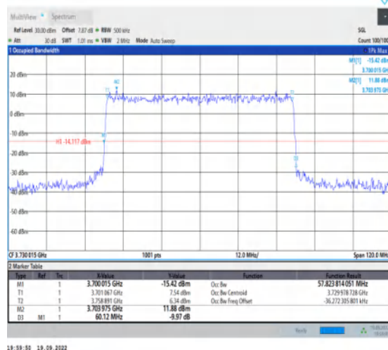
1-N77-3700-3980--30-60-L-7-CP-16QAM-Outer_Full-162@0-Ant1-57.824-60.120-≤60-PASS
