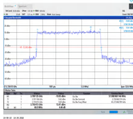
1-N77-3700-3980--30-60-L-1-DFT-QPSK-Outer_Full -162@0-Ant1-57.909-60.000-≤60-PASS
