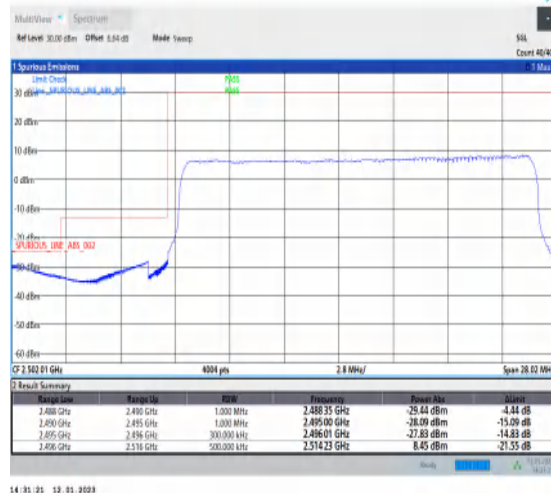
1-N41-PC3-30-20-L-3-DFT-PI2BPSK-Outer_Full-50@0-Ant1-1--PASS-see graph
