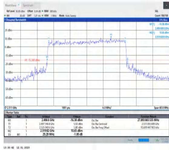
1-N41-PC3-30-30-L-7-CP-16QAM-Outer_Full-78@0- Ant1-27.894-29.280-≤30-PASS
