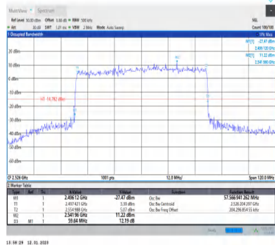
1-N41-PC3-30-60-L-4-DFT-64QAM-Outer_Full-162 @0-Ant1-57.567-59.640-≤60-PASS
