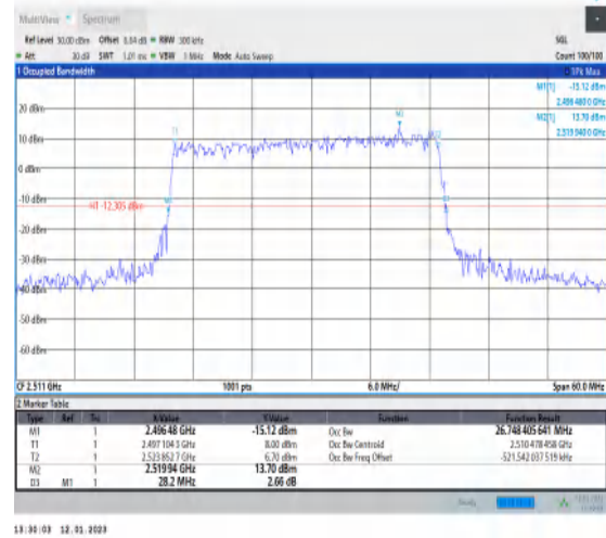
1-N41-PC3-30-30-L-3-DFT-16QAM-Outer_Full-75@ 0-Ant1-26.748-28.200-≤30-PASS
