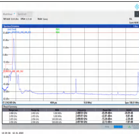
1-N41-PC3-30-100-L-1-DFT-PI2BPSK-Edge_1RB_Left-1@0-Ant1-1--PASS-see graph
