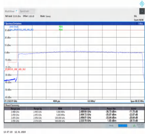
1-N41-PC3-30-80-L-3-DFT-PI2BPSK-Outer_Full-216@0-Ant1-1--PASS-see graph
