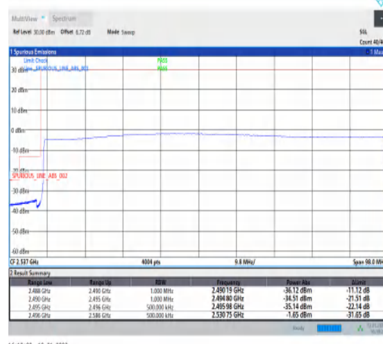
1-N41-PC3-30-90-L-6-CP-QPSK-Outer_Full-245@0-Ant1-1--PASS-see graph
