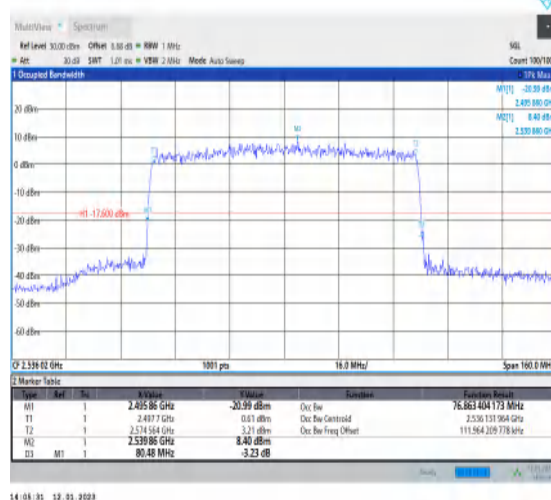
1-N41-PC3-30-80-L-9-CP-256QAM-Outer_Full-217@0-Ant1-76.863-80.480-≤80-PASS
