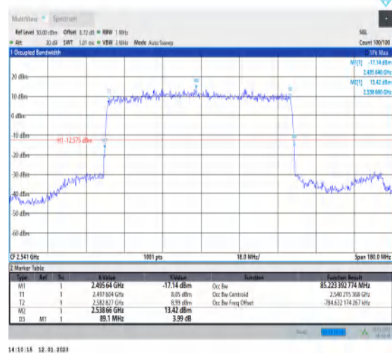
1-N41-PC3-30-90-L-2-DFT-PI2BPSK-Outer_Full-240 @0-Ant1-85.223-89.100-≤90-PASS
