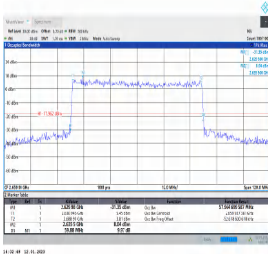
1-N41-PC3-30-60-H-5-DFT-256QAM-Outer_Full-162 @0-Ant1-57.965-59.880-≤60-PASS
