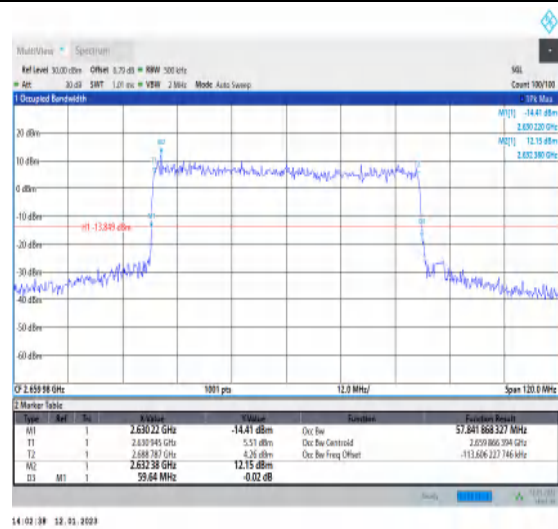
1-N41-PC3-30-60-H-4-DFT-64QAM-Outer_Full-162 @0-Ant1-57.842-59.640-≤60-PASS
