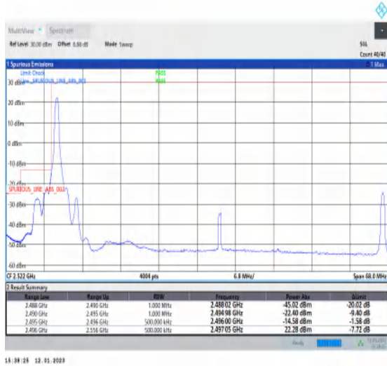
1-N41-PC3-30-60-L-1-DFT-PI2BPSK-Edge_1RB_Left-1@0-Ant1-1--PASS-see graph
