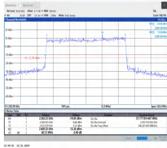
1-N41-PC3-30-60-M-1-DFT-QPSK-Outer_Full-162@ 0-Ant1-57.778-60.120-≤60-PASS
