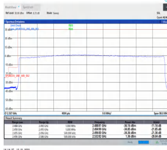
1-N41-PC3-30-90-L-3-DFT-PI2BPSK-Outer_Full-240@0-Ant1-1--PASS-see graph
