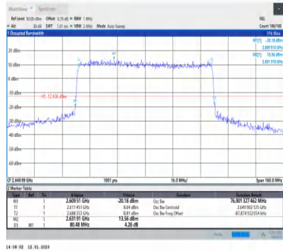
1-N41-PC3-30-80-H-1-DFT-QPSK-Outer_Full-216@ 0-Ant1-76.901-80.480-≤80-PASS
