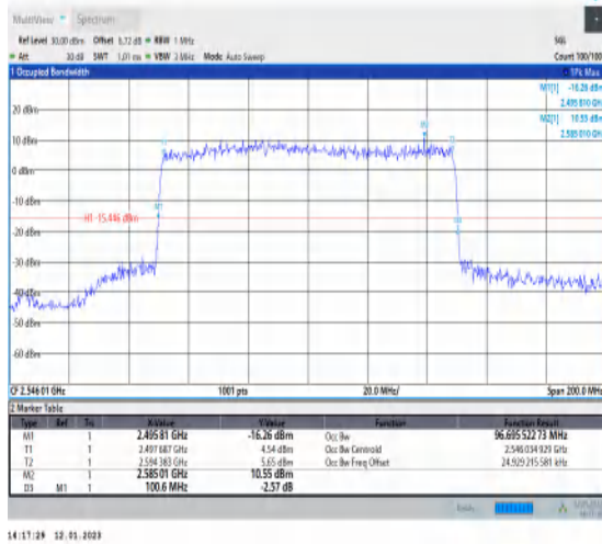
1-N41-PC3-30-100-L-8-CP-64QAM-Outer_Full-273 @0-Ant1-96.696-100.600-≤100-PASS
