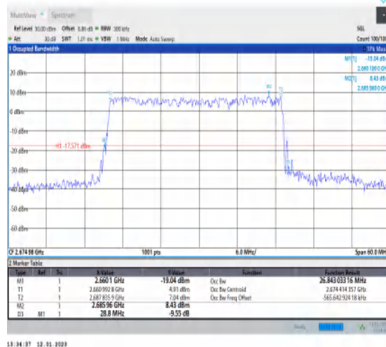
1-N41-PC3-30-30-H-5-DFT-256QAM-Outer_Full-75@ 0-Ant1-26.843-28.800-≤30-PASS
