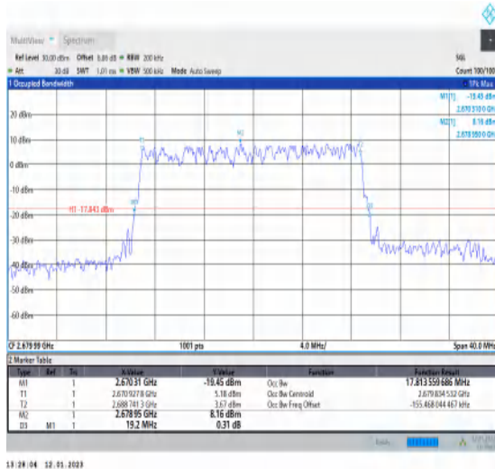
1-N41-PC3-30-20-H-5-DFT-256QAM-Outer_Full-50 @0-Ant1-17.814-19.200-≤20-PASS
