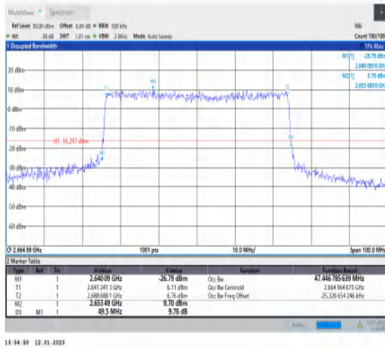
1-N41-PC3-30-50-H-6-CP-QPSK-Outet_Full-133@0-Ant1-47.447-49.500-≤50-PASS
