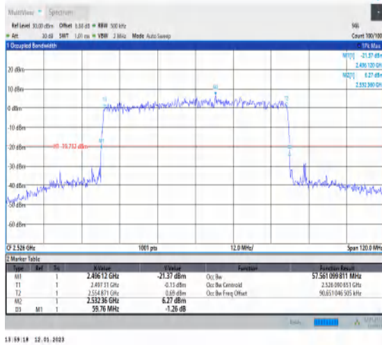
1-N41-PC3-30-60-L-9-CP-256QAM-Outer_Full-162 @0-Ant1-57.561-59.760-≤60-PASS
