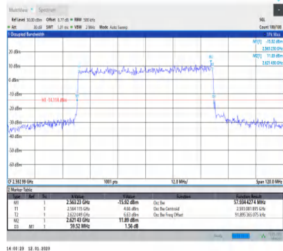
1-N41-PC3-30-60-M-3-DFT-16QAM-Outer_Full-162 @0-Ant1-57.934-59.520-≤60-PASS
