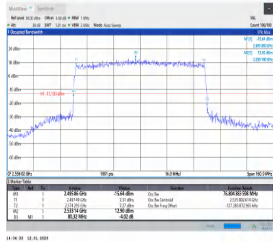
1-N41-PC3-30-80-L-3-DFT-16QAM-Outer_Full-216 @0-Ant1-76.804-80.320-≤80-PASS
