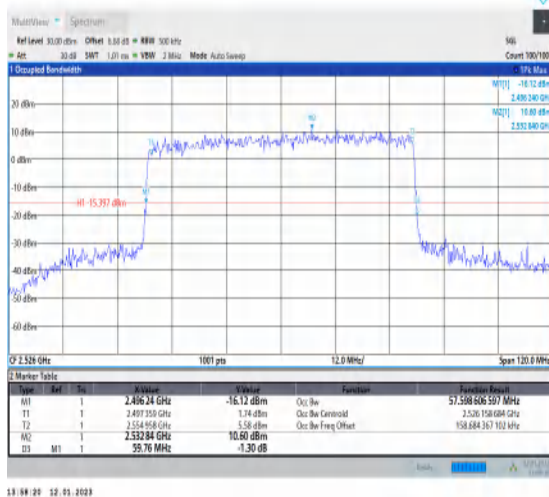
1-N41-PC3-30-60-L-3-DFT-16QAM-Outer_Full-162 @0-Ant1-57.599-59.760-≤60-PASS
