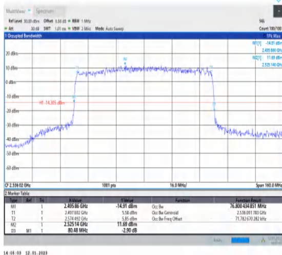
1-N41-PC3-30-80-L-6-CP-QPSK-Outer_Full-217@0-Ant1-76.8-80.480-≤80-PASS
