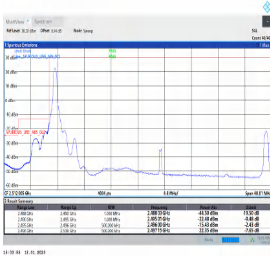
1-N41-PC3-30-40-L-1-DFT-PI2BPSK-Edge_1RB_Left-1@0-Ant1-1--PASS-see graph
