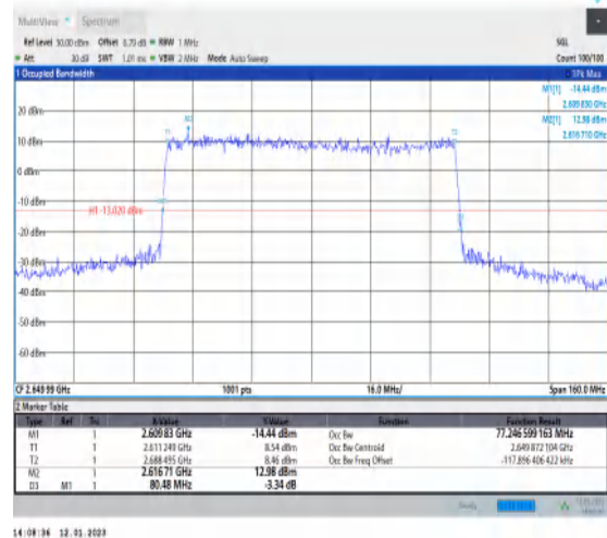
1-N41-PC3-30-80-H-3-DFT-16QAM-Outer_Full-216 @0-Ant1-77.247-80.480-≤80-PASS
