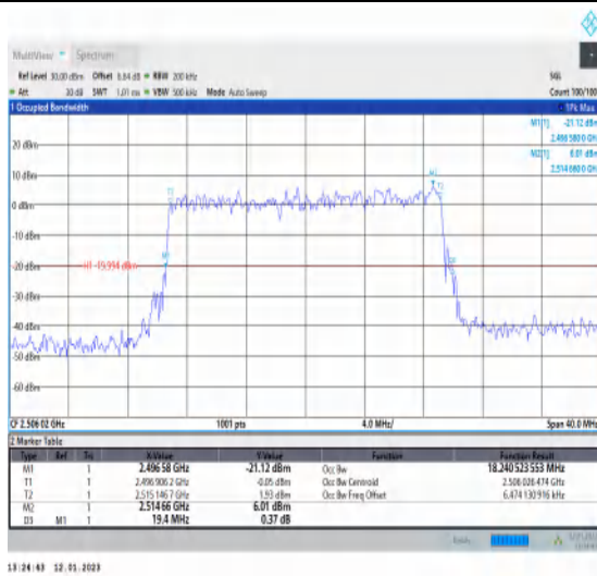
1-N41-PC3-30-20-L-9-CP-256QAM-Outer_Full-51@ 0-Ant1-18.241-19.400-≤20-PASS
