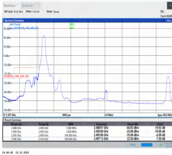
1-N41-PC3-30-30-L-1-DFT-PI2BPSK-Edge_1RB_Left-1@0-Ant1-1--PASS-see graph
