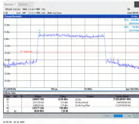
1-N41-PC3-30-80-H-9-CP-256QAM-Outer_Full-217 @0-Ant1-77.435-80.640-≤80-PASS
