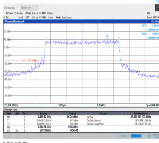
1-N41-PC3-30-30-H-7-CP-16QAM-Outer_Full-78@0- Ant1-27.93-30.180-≤30-PASS
