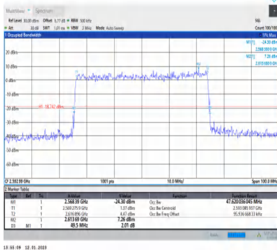
1-N41-PC3-30-50-M-9-CP-256QAM-Outer_Full-133 @0-Ant1-47.62-49.500-≤50-PASS
