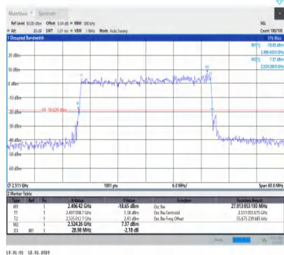
1-N41-PC3-30-30-L-9-CP-256QAM-Outer_Full-78@0- Ant1-27.914-28.980-≤30-PASS
