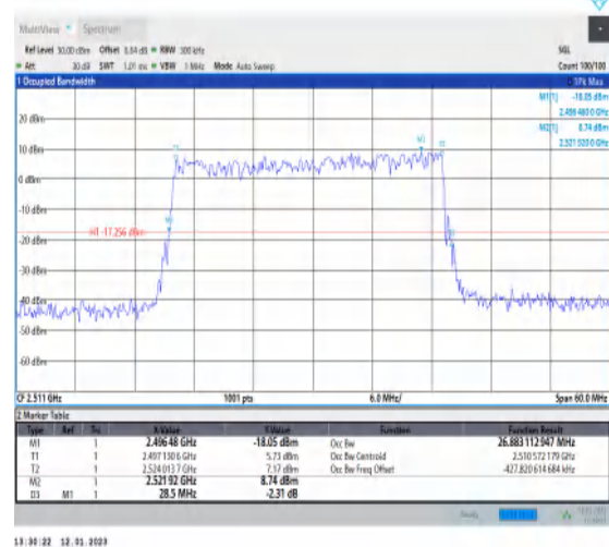
1-N41-PC3-30-30-L-5-DFT-256QAM-Outer_Full-75 @0-Ant1-26.883-28.500-≤30-PASS
