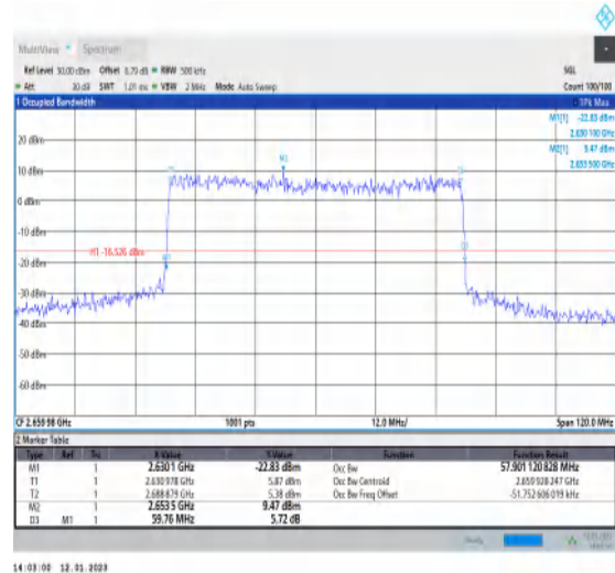
1-N41-PC3-30-60-H-6-CP-QPSK-Outer_Full-162@0 -Ant1-57.901-59.760-≤60-PASS
