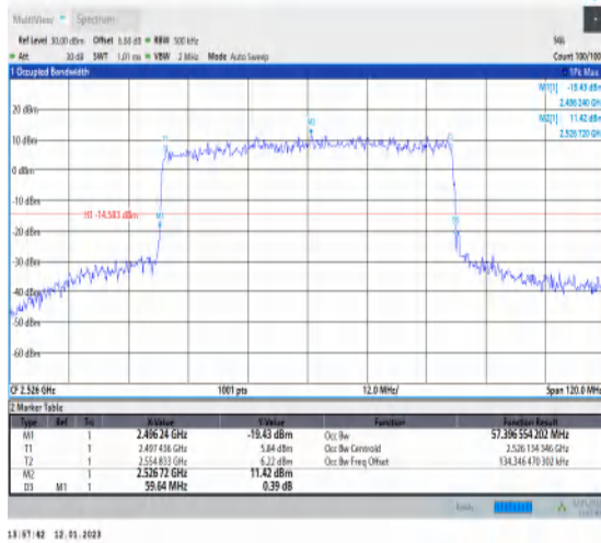
1-N41-PC3-30-60-L-1-DFT-QPSK-Outer_Full-162@0 -Ant1-57.397-59.640-≤60-PASS
