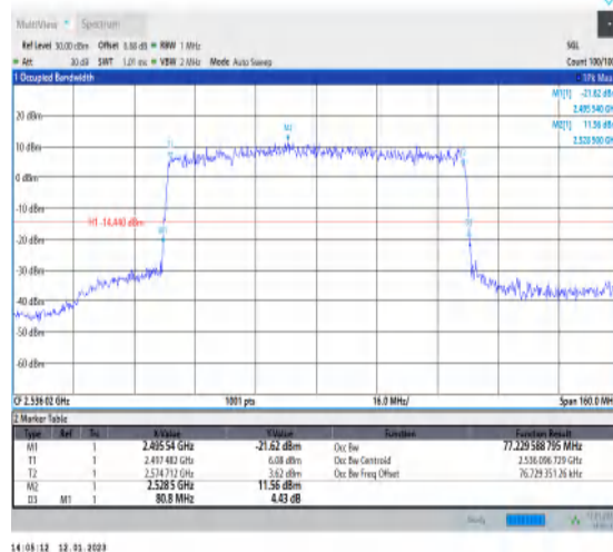
1-N41-PC3-30-80-L-7-CP-16QAM-Outer_Full-217@0-Ant1-77.23-80.800-≤80-PASS
