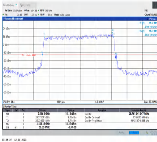
1-N41-PC3-30-30-L-2-DFT-PI2BPSK-Outer_Full-75 @0-Ant1-26.762-28.380-≤30-PASS
