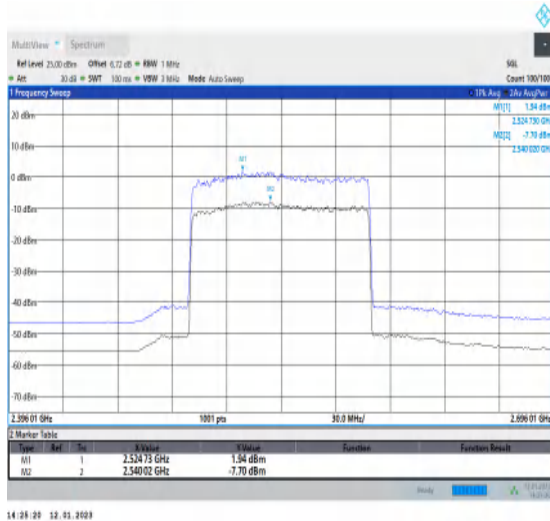
1-N41-PC3-30-100-L-1-DFT-256QAM-Outet_Full-270 @0-Ant1-9.64-100%-0.00-9.64-PASS-≤13
