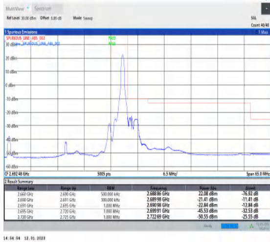
1-N41-PC3-30-30-H-2-DFT-PI2BPSK-Edge_1RB_Right-t-1@77-Ant1-1--PASS-see graph
