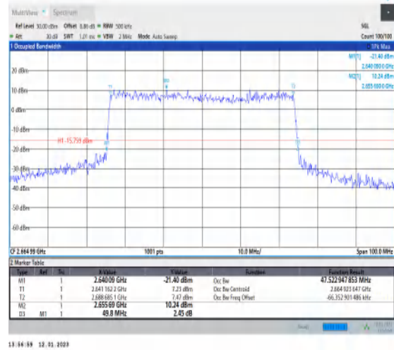
1-N41-PC3-30-50-H-7-CP-16QAM-Outet_Full-133@0-Ant1-47.523-49.800-≤50-PASS
