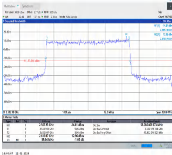
1-N41-PC3-30-60-M-2-DFT-PI2BPSK-Outer_Full-16 2@0-Ant1-58.086-59.640-≤60-PASS
