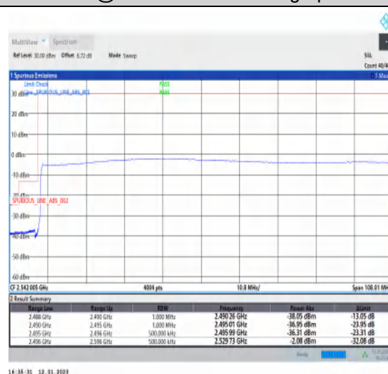
1-N41-PC3-30-100-L-6-CP-QPSK-Outer_Full-273@0-Ant1-1--PASS-see graph
