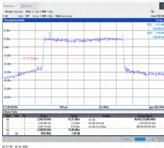
1-N41-PC3-30-100-M-1-DFT-QPSK-Outer_Full-270 @0-Ant1-96.432-99.800-≤100-PASS
