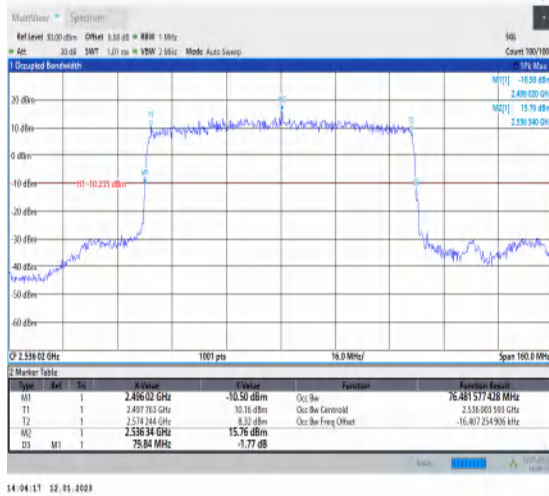
1-N41-PC3-30-80-L-2-DFT-PI2BPSK-Outer_Full-216 @0-Ant1-76.482-79.840-≤80-PASS
