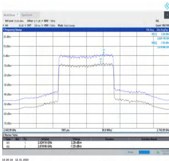
1-N41-PC3-30-100-M-1-DFT-256QAM-Outet_Full-27 0@0-Ant1-9.61-100%-0.00-9.61-PASS-≤13
