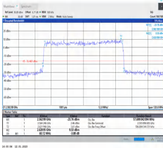
1-N41-PC3-30-60-M-6-CP-QPSK-Outer_Full-162@0 -Ant1-57.699-60.120-≤60-PASS
