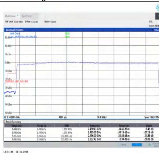
1-N41-PC3-30-100-L-3-DFT-PI2BPSK-Outer_Full-270@0-Ant1-1--PASS-see graph
