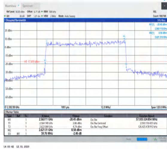
1-N41-PC3-30-60-M-5-DFT-256QAM-Outer_Full-162 @0-Ant1-57.935-59.760-≤60-PASS
