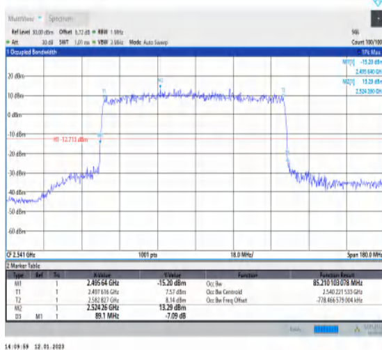
1-N41-PC3-30-90-L-1-DFT-QPSK-Outer_Full-240@0 -Ant1-85.21-89.100-≤90-PASS
