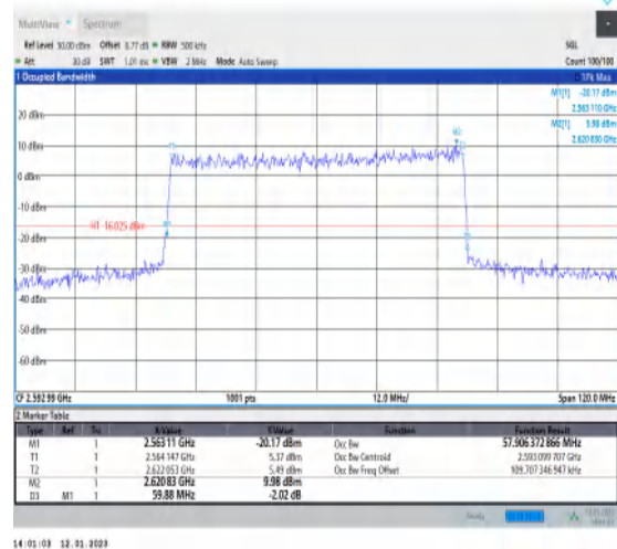
1-N41-PC3-30-60-M-7-CP-16QAM-Outer_Full-162@0 0-Ant1-57.906-59.880-≤60-PASS
