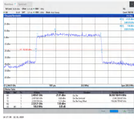
1-N41-PC3-30-100-L-9-CP-256QAM-Outer_Full-273 @0-Ant1-96.931-100.800-≤100-PASS
