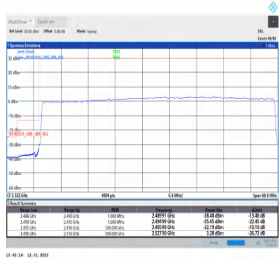
1-N41-PC3-30-60-L-3-DFT-PI2BPSK-Outer_Full-162@0-Ant1-1--PASS-see graph
