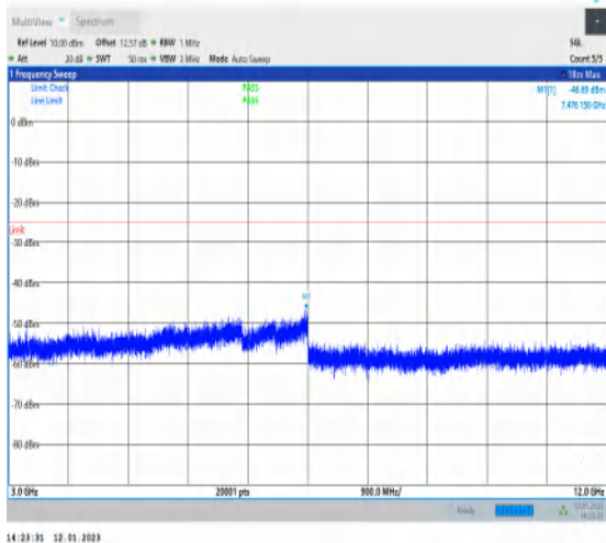
1-N41-PC3-30-100-M-1-DFT-PI2BPSK-Inner_1RB_Left-1@1-3000-12000-Ant1-7478.85--46.69--25-PASS SS
