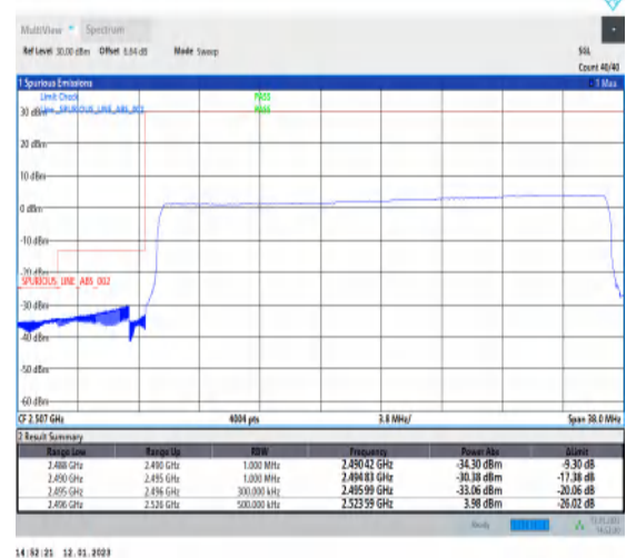
1-N41-PC3-30-30-L-6-CP-QPSK-Outer_Full-78@0-Ant1-1--PASS-see graph
