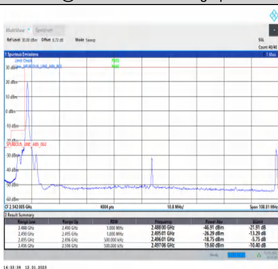
1-N41-PC3-30-100-L-4-CP-QPSK-Edge_1RB_Left-1@0-Ant1-1--PASS-see graph
