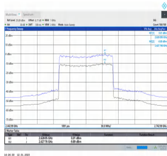
1-N41-PC3-30-100-M-2-CP-256QAM-Outet_Full-27 3@0-Ant1-9.90-100%-0.00-9.90-PASS-≤13
