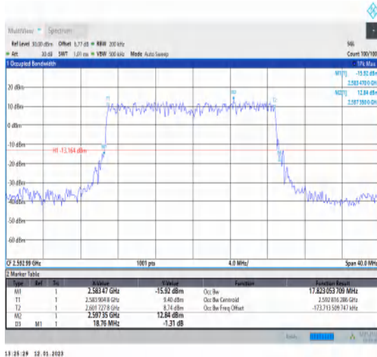
1-N41-PC3-30-20-M-2-DFT-PI2BPSK-Outer_Full-50 @0-Ant1-17.823-18.760-≤20-PASS
