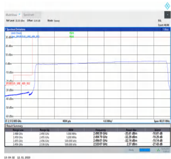
1-N41-PC3-30-40-L-6-CP-QPSK-Outer_Full-106@0-Ant1-1--PASS-see graph
