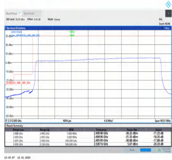
1-N41-PC3-30-40-L-3-DFT-PI2BPSK-Outer_Full-100@0-Ant1-1--PASS-see graph
