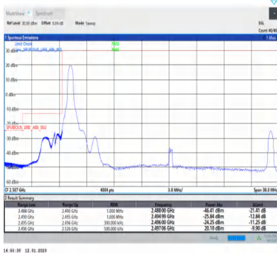
1-N41-PC3-30-30-L-4-CP-QPSK-Edge_1RB_Left-1@0-Ant1-1--PASS-see graph
