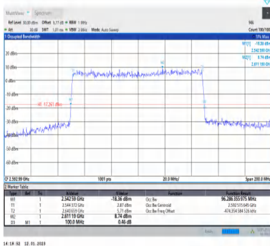
1-N41-PC3-30-100-M-5-DFT-256QAM-Outer_Full-270 @0-Ant1-96.286-100.000-≤100-PASS
