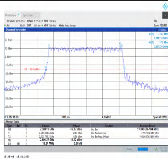
1-N41-PC3-30-20-M-1-DFT-QPSK-Outer_Full-50@0 -Ant1-17.841-19.240-≤20-PASS
