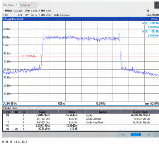
1-N41-PC3-30-80-H-4-DFT-64QAM-Outer_Full-216 @0-Ant1-76.98-80.320-≤80-PASS
