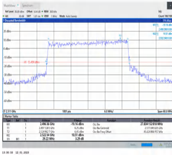
1-N41-PC3-30-30-L-6-CP-QPSK-Outer_Full-78@0-A Ant1-27.834-29.220-≤30-PASS
