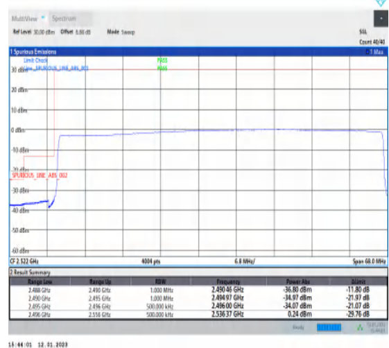
1-N41-PC3-30-60-L-6-CP-QPSK-Outer_Full-162@0-Ant1-1--PASS-see graph
