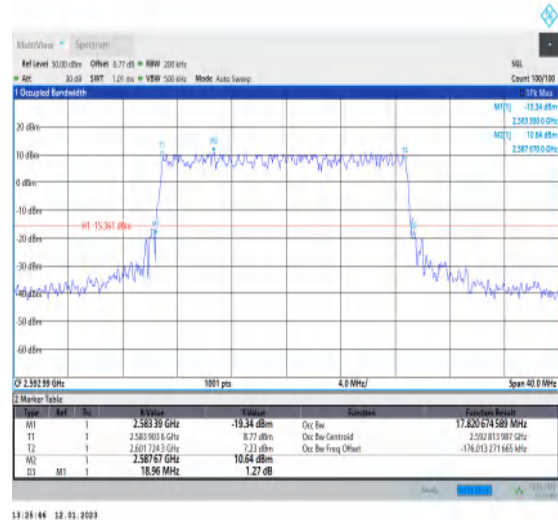
1-N41-PC3-30-20-M-3-DFT-16QAM-Outer_Full-50@ 0-Ant1-17.821-18.960-≤20-PASS
