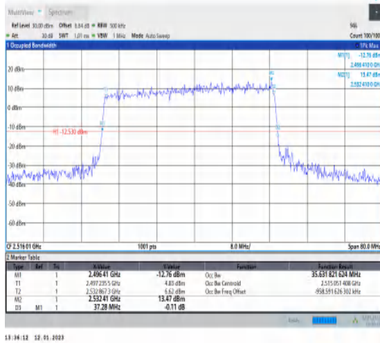
1-N41-PC3-30-40-L-3-DFT-16QAM-Outer_Full-100 @0-Ant1-35.632-37.280-≤40-PASS
