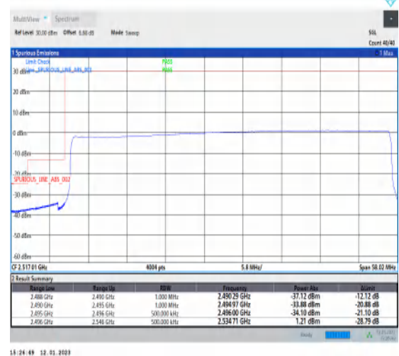
1-N41-PC3-30-50-L-6-CP-QPSK-Outer_Full-133@0-Ant1-1--PASS-see graph
