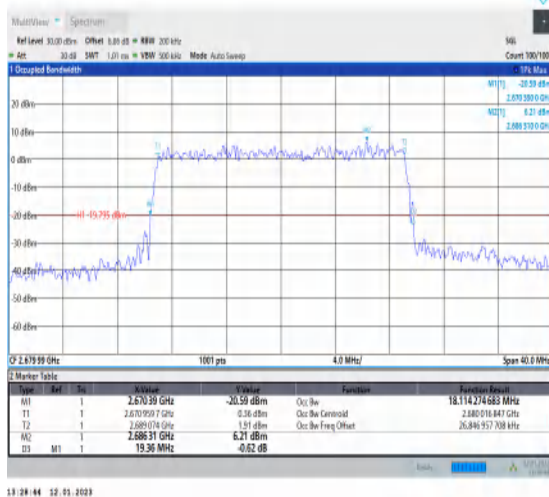
1-N41-PC3-30-20-H-9-CP-256QAM-Outer_Full-51@0 -Ant1-18.114-19.360-≤20-PASS
