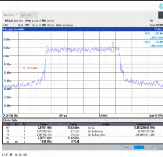
1-N41-PC3-30-20-H-3-DFT-16QAM-Outer_Full-50@ 0-Ant1-17.853-18.920-≤20-PASS
