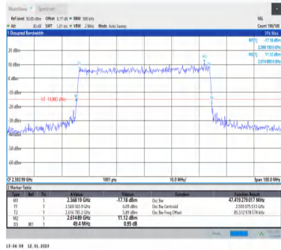
1-N41-PC3-30-50-M-8-CP-64QAM-Outer_Full-133@ 0-Ant1-47.419-49.400-≤50-PASS
