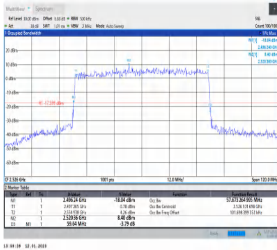
1-N41-PC3-30-60-L-5-DFT-256QAM-Outer_Full-162@0-Ant1-57.673-59.640-≤60-PASS
