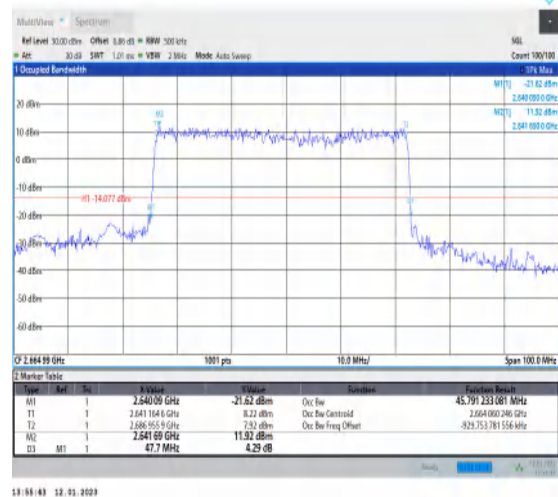
1-N41-PC3-30-50-H-1-DFT-QPSK-Outer_Full-128@ 0-Ant1-45.791-47.700-≤50-PASS
