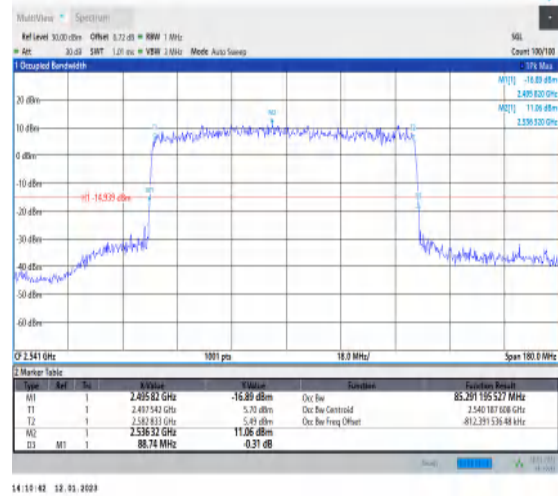
1-N41-PC3-30-90-L-4-DFT-64QAM-Outer_Full-240 @0-Ant1-85.291-88.740-≤90-PASS
