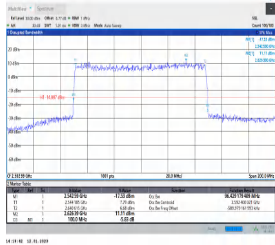
1-N41-PC3-30-100-M-4-DFT-64QAM-Outer_Full-270 @0-Ant1-96.429-100.000-≤100-PASS
