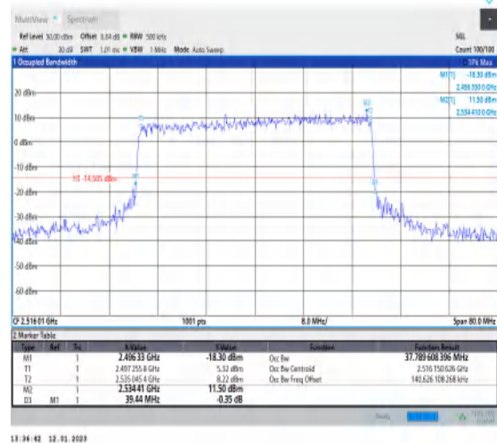
1-N41-PC3-30-40-L-6-CP-QPSK-Outer_Full-106@0-Ant1-37.79-39.440-≤40-PASS
