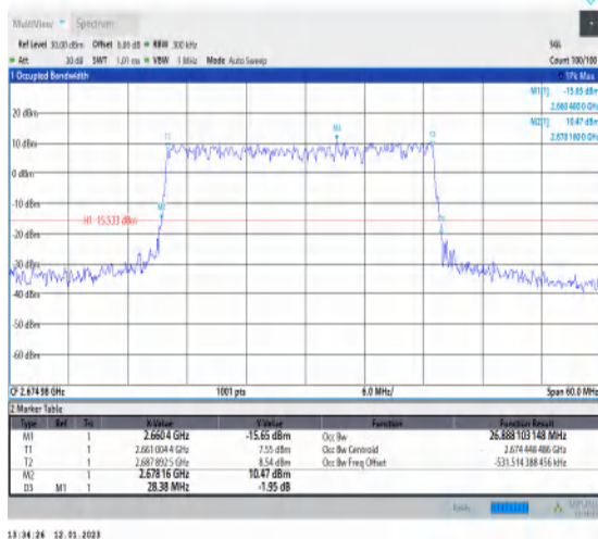
1-N41-PC3-30-30-H-4-DFT-64QAM-Outer_Full-75@ 0-Ant1-26.888-28.380-≤30-PASS
