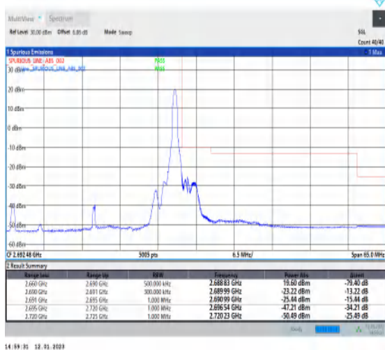
1-N41-PC3-30-30-H-5-CP-QPSK-Edge_1RB_Right-1@77-Ant1-1--PASS-see graph
