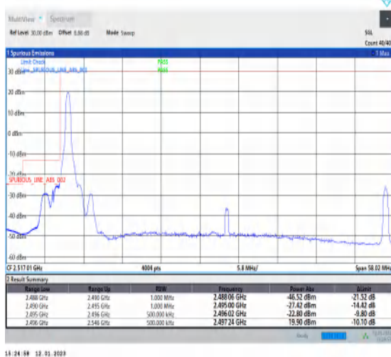
1-N41-PC3-30-50-L-4-CP-QPSK-Edge_1RB_Left-1@0-Ant1-1--PASS-see graph
