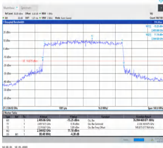
1-N41-PC3-30-80-L-8-CP-64QAM-Outer_Full-217@0-Ant1-76.994-80.480-≤80-PASS
