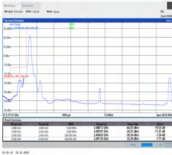
1-N41-PC3-30-50-L-1-DFT-PI2BPSK-Edge_1RB_Left-1@0-Ant1-1--PASS-see graph
