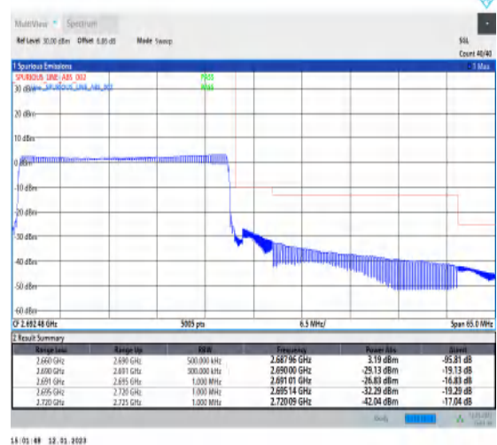
1-N41-PC3-30-30-H-6-CP-QPSK-Outer_Full-78@0-Ant1-1--PASS-see graph
