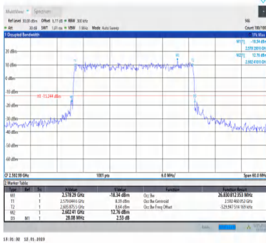
1-N41-PC3-30-30-M-1-DFT-QPSK-Outer_Full-75@0 -Ant1-26.831-28.080-≤30-PASS
