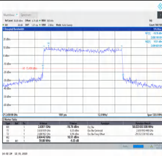
1-N41-PC3-30-60-H-3-DFT-16QAM-Outer_Full-162 @0-Ant1-58.023-59.880-≤60-PASS
