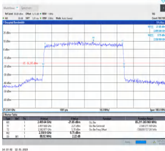
1-N41-PC3-30-90-L-5-DFT-256QAM-Outer_Full-240 @0-Ant1-85.211-88.920-≤90-PASS
