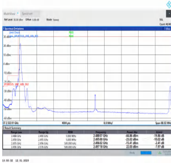
1-N41-PC3-30-80-L-1-DFT-PI2BPSK-Edge_1RB_Left-1@0-Ant1-1--PASS-see graph
