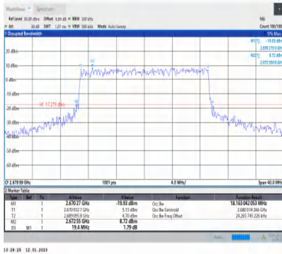
1-N41-PC3-30-20-H-7-CP-16QAM-Outer_Full-51@0 -Ant1-18.163-19.400-≤20-PASS
