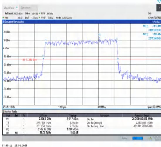
1-N41-PC3-30-30-L-4-DFT-64QAM-Outer_Full-75@ 0-Ant1-26.764-28.080-≤30-PASS
