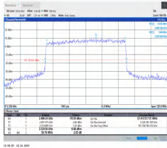
1-N41-PC3-30-60-L-6-CP-QPSK-Outer_Full-162@0-Ant1-57.414-59.760-≤60-PASS
