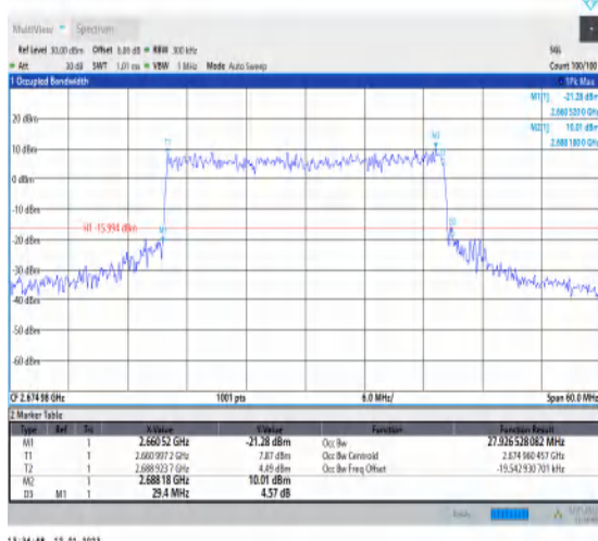
1-N41-PC3-30-30-H-6-CP-QPSK-Outer_Full-78@0- Ant1-27.927-29.400-≤30-PASS
