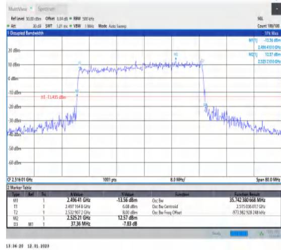
1-N41-PC3-30-40-L-4-DFT-64QAM-Outer_Full-100 @0-Ant1-35.742-37.360-≤40-PASS
