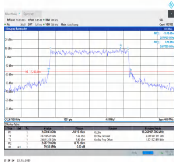
1-N41-PC3-30-20-H-6-CP-QPSK-Outer_Full-51@0- Ant1-18.269-19.360-≤20-PASS
