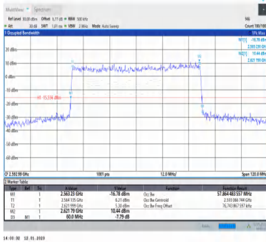
1-N41-PC3-30-60-M-4-DFT-64QAM-Outer_Full-162 @0-Ant1-57.864-60.000-≤60-PASS
