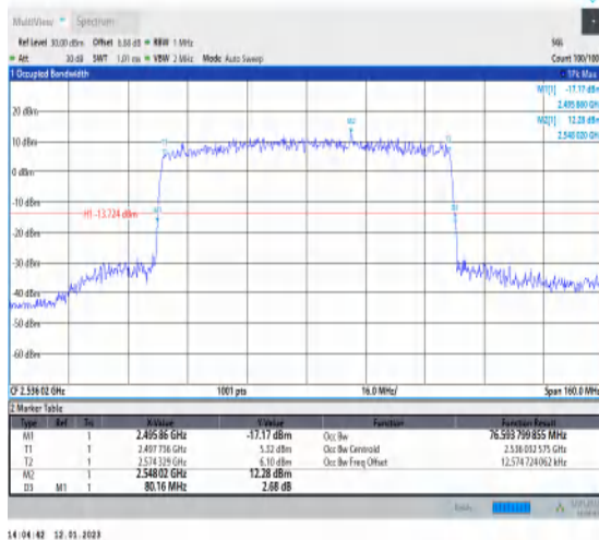
1-N41-PC3-30-80-L-4-DFT-64QAM-Outer_Full-216 @0-Ant1-76.594-80.160-≤80-PASS
