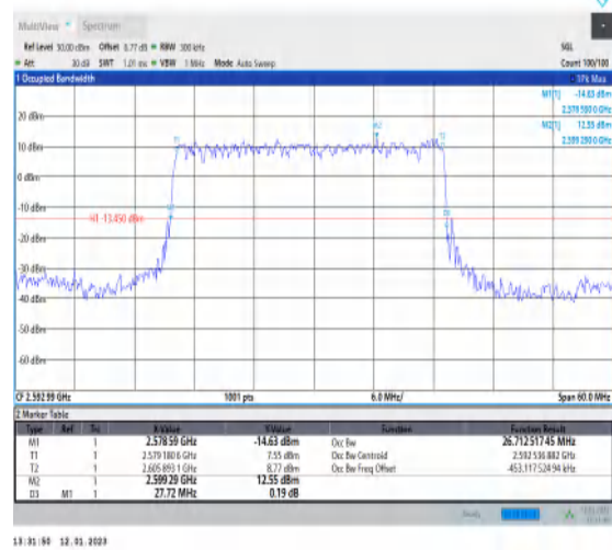
1-N41-PC3-30-30-M-2-DFT-PI2BPSK-Outer_Full-75 @0-Ant1-26.713-27.720-≤30-PASS
