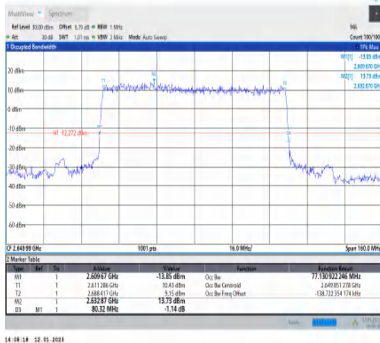
1-N41-PC3-30-80-H-2-DFT-PI2BPSK-Outer_Full-216 @0-Ant1-77.131-80.320-≤80-PASS
