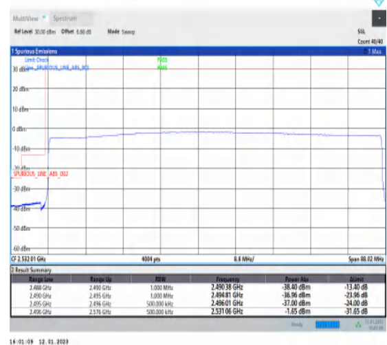
1-N41-PC3-30-80-L-6-CP-QPSK-Outer_Full-217@0-Ant1-1--PASS-see graph
