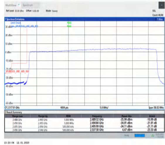
1-N41-PC3-30-50-L-3-DFT-PI2BPSK-Outer_Full-128@0-Ant1-1--PASS-see graph
