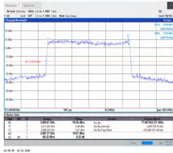
1-N41-PC3-30-80-H-5-DFT-256QAM-Outer_Full-216 @0-Ant1-77.098-80.320-≤80-PASS
