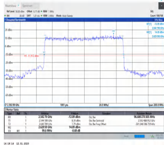
1-N41-PC3-30-100-M-2-DFT-PI2BPSK-Outer_Full-270 @0-Ant1-96.6-99.600-≤100-PASS
