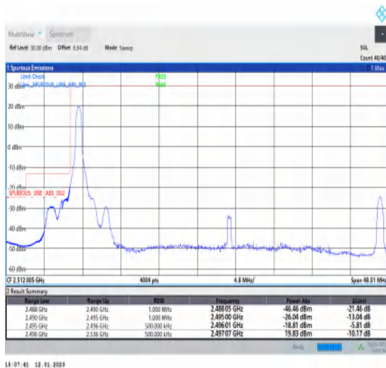
1-N41-PC3-30-40-L-4-CP-QPSK-Edge_1RB_Left-1@0-Ant1-1--PASS-see graph
