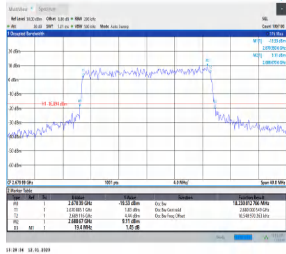
1-N41-PC3-30-20-H-8-CP-64QAM-Outer_Full-51@0 -Ant1-18.231-19.400-≤20-PASS
