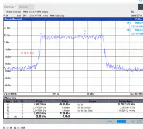
1-N41-PC3-30-30-M-4-DFT-64QAM-Outer_Full-75@0-Ant1-26.736-28.380-≤30-PASS
