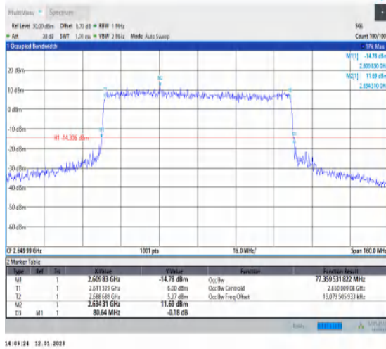
1-N41-PC3-30-80-H-8-CP-64QAM-Outer_Full-217@ 0-Ant1-77.36-80.640-≤80-PASS
