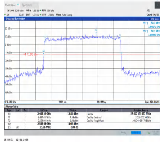
1-N41-PC3-30-60-L-2-DFT-PI2BPSK-Outer_Full-162 @0-Ant1-57.407-59.760-≤60-PASS
