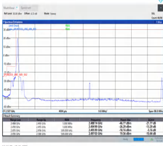
1-N41-PC3-30-90-L-4-CP-QPSK-Edge_1RB_Left-1@0-Ant1-1--PASS-see graph
