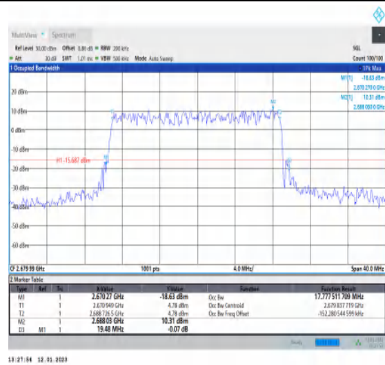
1-N41-PC3-30-20-H-4-DFT-64QAM-Outer_Full-50@ 0-Ant1-17.778-19.480-≤20-PASS
