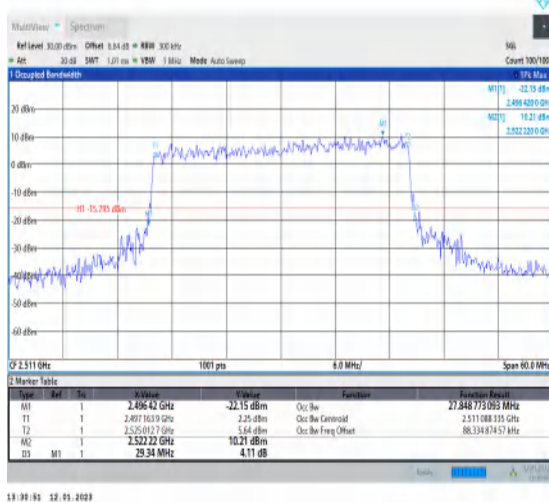
1-N41-PC3-30-30-L-8-CP-64QAM-Outer_Full-78@0- Ant1-27.849-29.340-≤30-PASS
