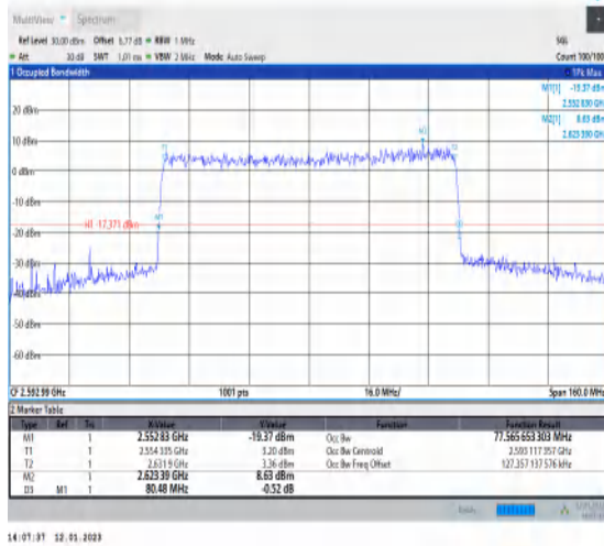
1-N41-PC3-30-80-M-9-CP-256QAM-Outer_Full-217 @0-Ant1-77.566-80.480-≤80-PASS
