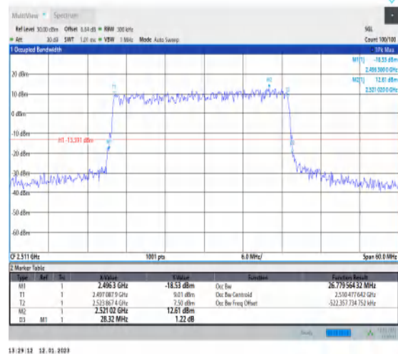
1-N41-PC3-30-30-L-1-DFT-QPSK-Outer_Full-75@0- Ant1-26.78-28.320-≤30-PASS
