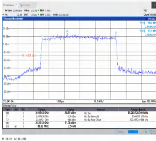
1-N41-PC3-90-90-L-3-DFT-16QAM-Outer_Full-240 @0-Ant1-85.283-88.920-≤90-PASS
