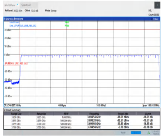
1-N78-3700-3800-PC2-30-90-L-6-CP-QPSK-Outer _Full-245@0-Ant1-1--PASS-see graph
