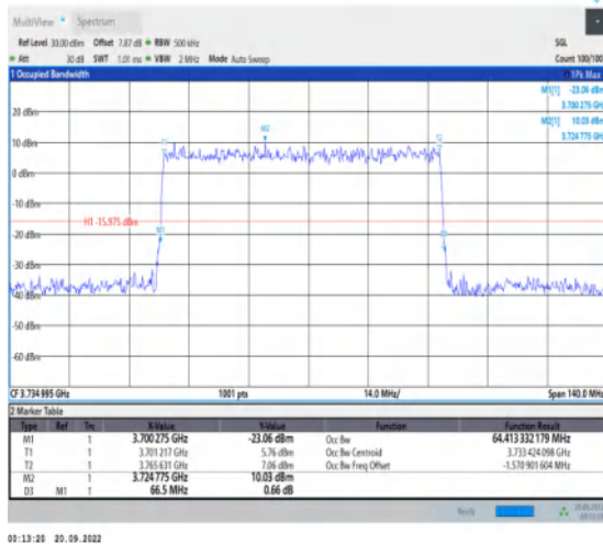
1-N78-3700-3800-30-70-L-5-DFT-256QAM-Outer_Fu II-180@0-Ant1-64.413-66.500-≤70-PASS
