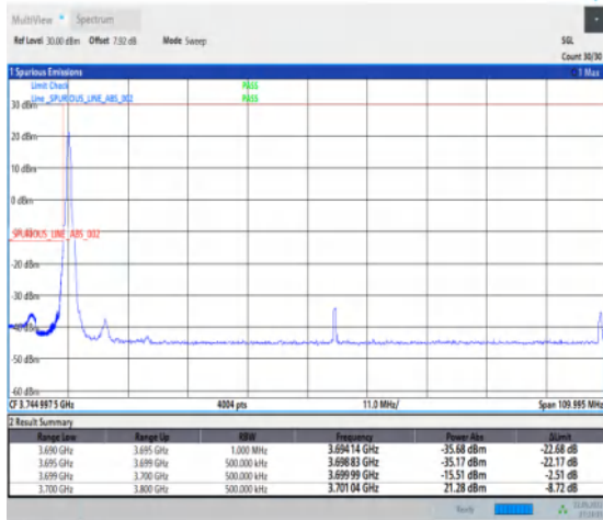
1-N78-3700-3800-30-100-L-1-DFT-PI2BPSK-Edge_1R_B_Left-1@0-Ant1-1--PASS-see graph
