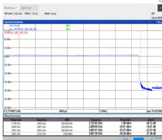
1-N78-3700-3800-30-60-H-6-CP-QPSK-Outer_Full -162@0-Ant1-1--PASS-see graph
