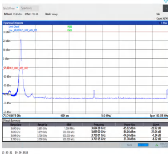
1-N78-3700-3800-30-90-L-4-CP-QPSK-Edge_1RB_Lef t-1@0-Ant1-1--PASS-see graph
