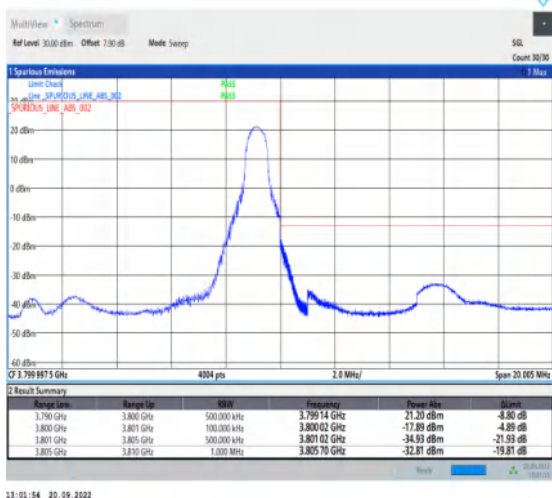
1-N78-3700-3800-30-10-H-2-DFT-PI2BPSK-Edge_1R_B_Right-1@23-Ant1-1--PASS-see graph
