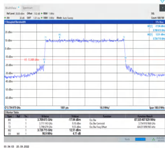
1-N78-3700-3800-30-90-H-6-CP-QPSK-Outer_Full-2 45@0-Ant1-87.535-90.900-≤90-PASS
