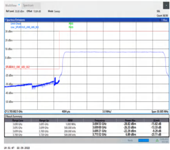
1-N78-3700-3800-PC2-30-20-L-6-CP-QPSK-Outer _Full-51@0-Ant1-1--PASS-see graph
