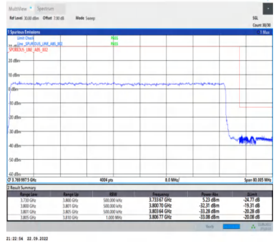
1-N78-3700-3800-30-70-H-3-DFT-PI2BPSK-Outer _Full-180@0-Ant1-1--PASS-see graph
