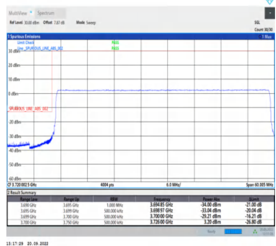
1-N78-3700-3800-30-50-L-6-CP-QPSK-Outer_Full -133@0-Ant1-1--PASS-see graph
