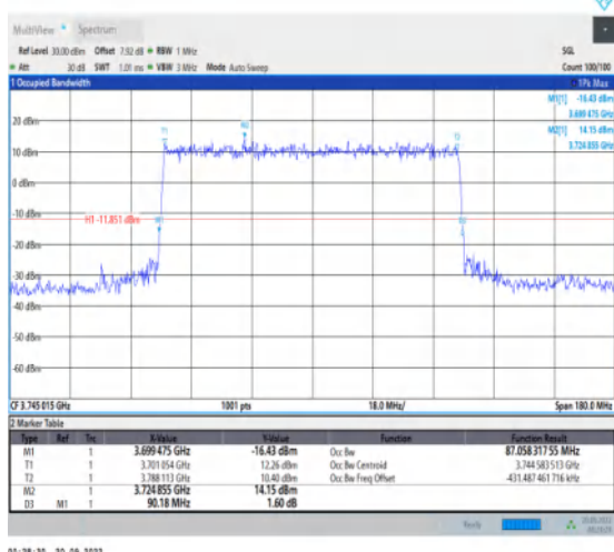
1-N78-3700-3800-30-90-L-3-DFT-16QAM-Outer_Full-243@0-Ant1-87.058-90.180-≤90-PASS
