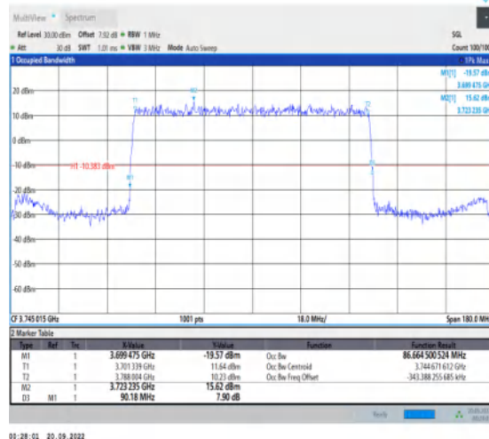
1-N78-3700-3800-30-90-L-2-DFT-PI2BPSK-Outer_Full-243@0-Ant1-86.665-90.180-≤90-PASS
