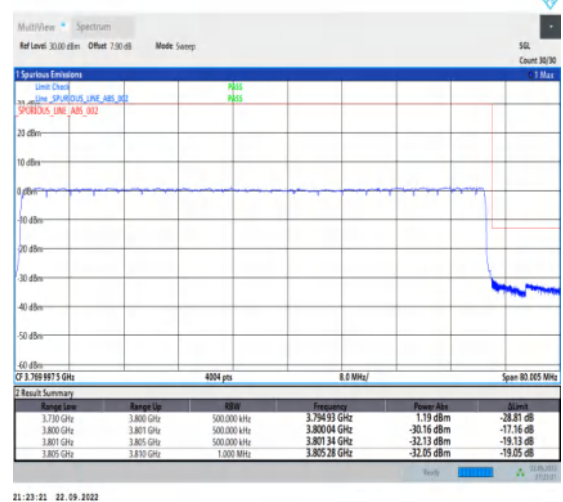
1-N78-3700-3800-30-70-H-6-CP-QPSK-Outer_Full -189@0-Ant1-1--PASS-see graph
