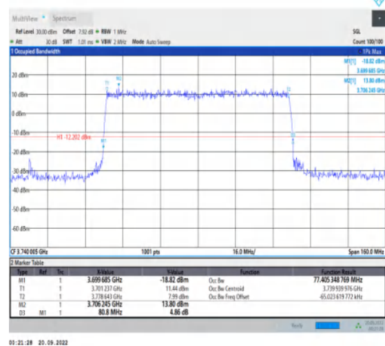
1-N78-3700-3800-30-80-L-7-CP-16QAM-Outer_Full- 217@0-Ant1-77.405-80.800-≤80-PASS
