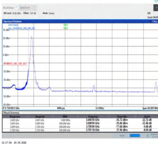
1-N78-3700-3800-30-50-L-4-CP-QPSK-Edge_1RB_Lef t-1@0-Ant1-1--PASS-see graph
