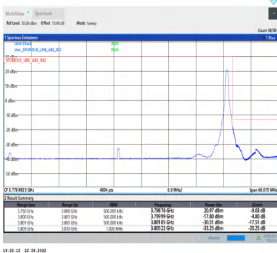
1-N78-3700-3800-PC2-30-50-H-5-CP-QPSK-Edge_1R B_Right-1@132-Ant1-1--PASS-see graph
