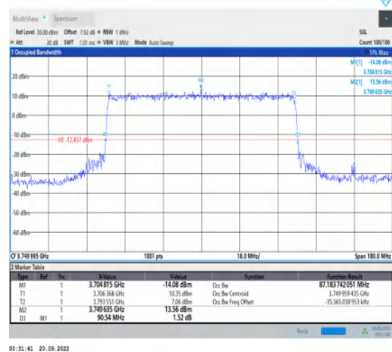
1-N78-3700-3800-30-90-M-7-CP-16QAM-Outer_Full -245@0-Ant1-87.184-90.540≤90-PASS
