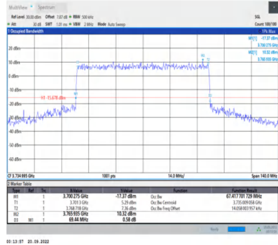
1-N78-3700-3800-30-70-L-8-CP-64QAM-Outer_Full-189@0-Ant1-67.418-69.440-≤70-PASS
