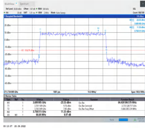
1-N78-3700-3800-30-70-L-4-DFT-64QAM-Outer_Full -180@0-Ant1-64.44-66.640-≤70-PASS
