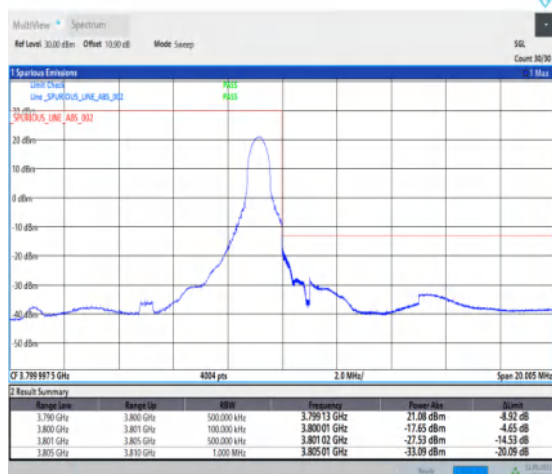
1-N78-3700-3800-PC2-30-10-H-5-CP-QPSK-Edge_1R B_Right-1@23-Ant1-1--PASS-see graph
