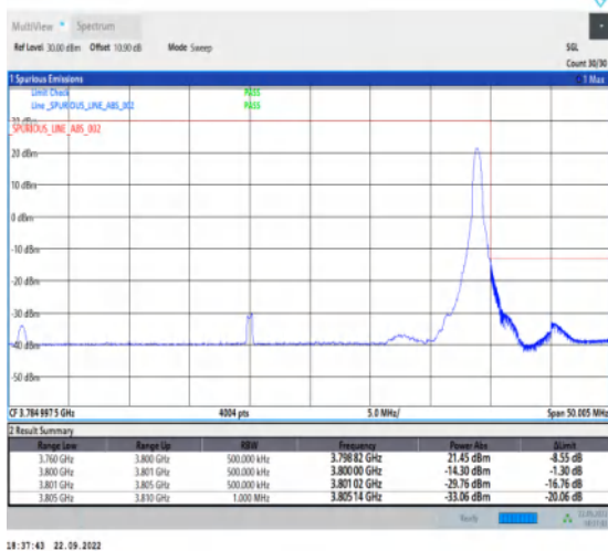
1-N78-3700-3800-PC2-30-40-H-5-CP-QPSK-Edge_1R B_Right-1@105-Ant1-1--PASS-see graph
