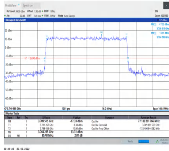
1-N78-3700-3800-30-80-M-4-DFT-64QAM-Outer_Ful I-216@0-Ant1-77.189-80.480-≤80-PASS
