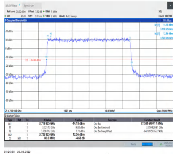
1-N78-3700-3800-30-80-H-7-CP-16QAM-Outter_Full-217@0-Ant1-77.582-80.800-≤80-PASS
