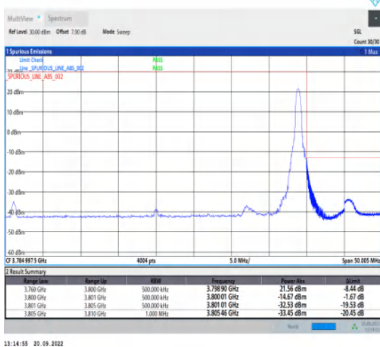
1-N78-3700-3800-30-40-H-5-CP-QPSK-Edge_1RB_Ri ght-1@105-Ant1-1--PASS-see graph
