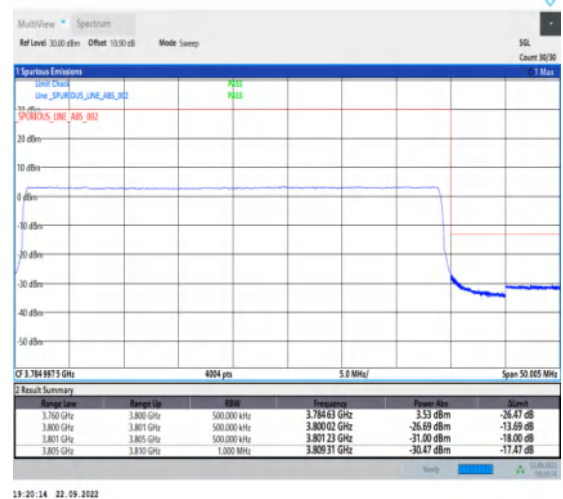
1-N78-3700-3800-PC2-30-40-H-6-CP-QPSK-Outer _Full-106@0-Ant1-1--PASS-see graph
