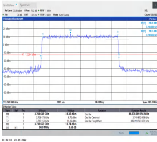
1-N78-3700-3800-30-90-M-4-DFT-64QAM-Outer_Full I-243@0-Ant1-86.678-90.000≤90-PASS
