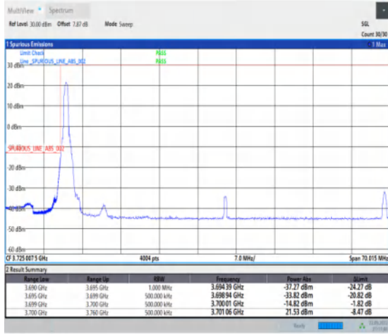
1-N78-3700-3800-30-60-L-1-DFT-PI2BPSK-Edge_1RB_Left-1@0-Ant1-1--PASS-see graph
