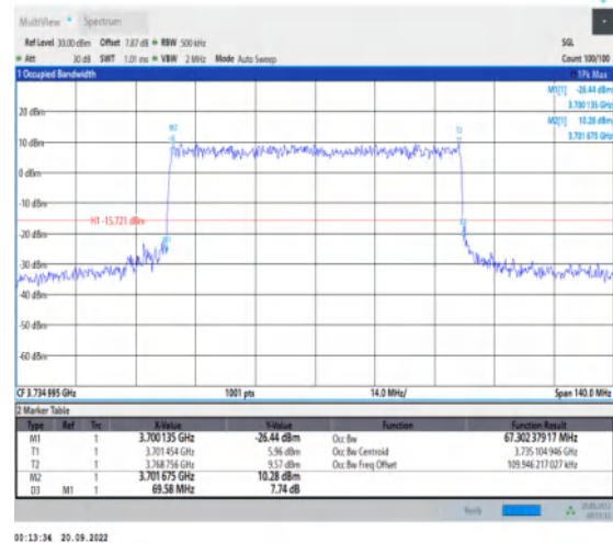
1-N78-3700-3800-30-70-L-6-CP-QPSK-Outer_Full-1 89@0-Ant1-67.302-69.580-≤70-PASS
