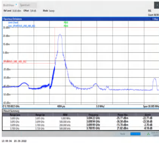
1-N78-3700-3800-30-20-L-1-DFT-PI2BPSK-Edge_1RB_Left-1@0-Ant1-1--PASS-see graph
