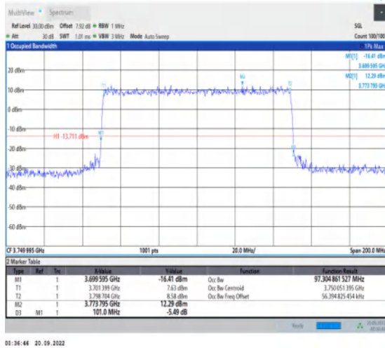
1-N78-3700-3800-30-100-L-6-CP-QPSK-Outter_Full-273@0-Ant1-97.305-101.000-≤100-PASS
