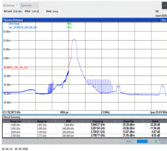
1-N78-3700-3800-PC2-30-15-L-4-CP-QPSK-Edge_1R B_Left-1@0-Ant1-1--PASS-see graph
