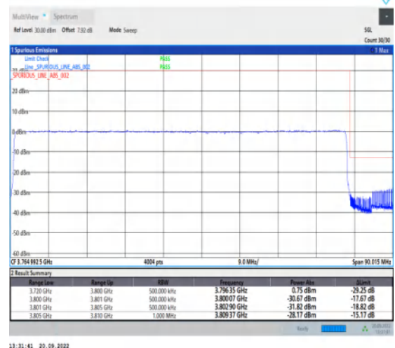
1-N78-3700-3800-30-80-H-6-CP-QPSK-Outer_Full -217@0-Ant1-1--PASS-see graph
