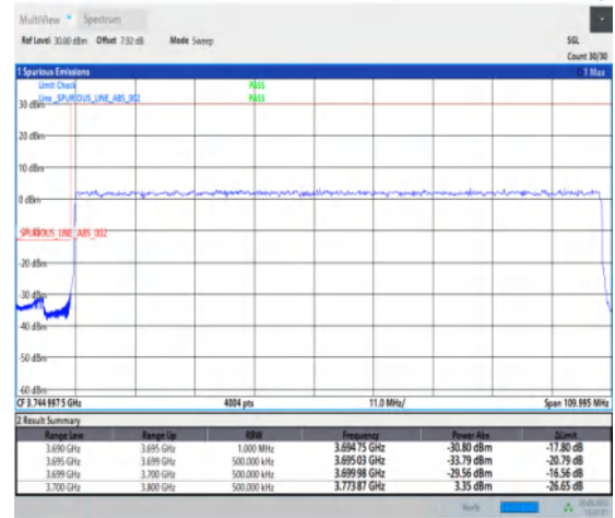
1-N78-3700-3800-30-100-L-3-DFT-PI2BPSK-Outer_Full-270@0-Ant1-1--PASS-see graph
