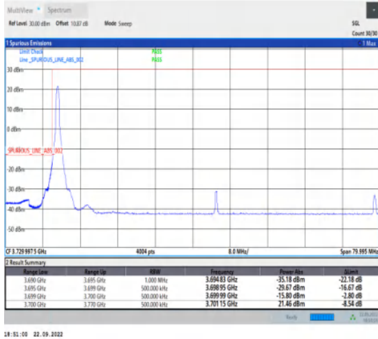
1-N78-3700-3800-PC2-30-70-L-4-CP-QPSK-Edge_1R B_Left-1@0-Ant1-1--PASS-see graph
