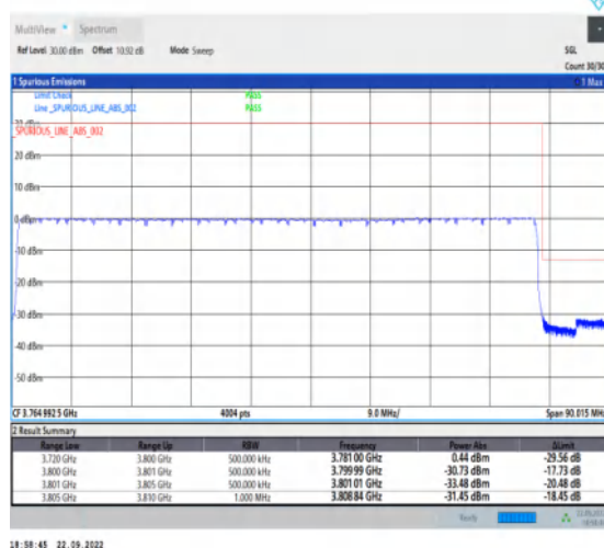
1-N78-3700-3800-PC2-30-80-H-6-CP-QPSK-Outer _Full-217@0-Ant1-1--PASS-see graph
