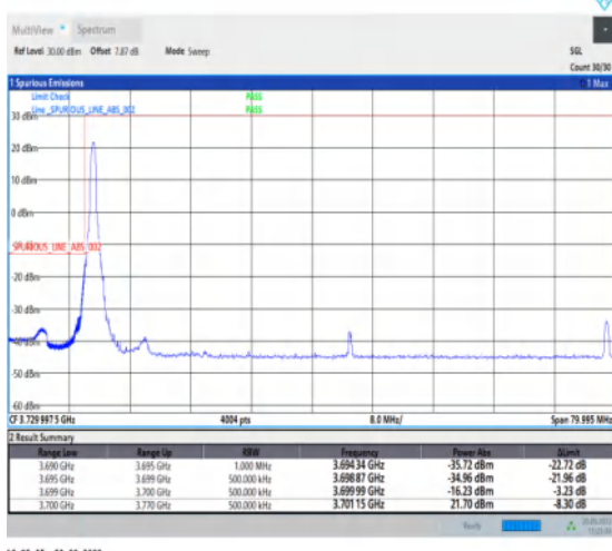
1-N78-3700-3800-30-70-L-4-CP-QPSK-Edge_1RB_Lef t-1@0-Ant1-1--PASS-see graph
