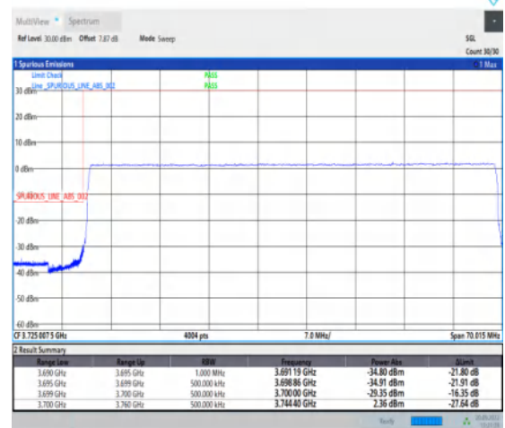
1-N78-3700-3800-30-60-L-6-CP-QPSK-Outer_Full_-162@0-Ant1-1--PASS-see graph
