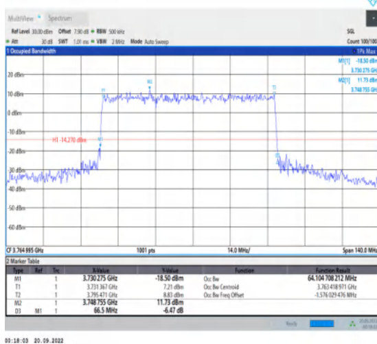
1-N78-3700-3800-30-70-H-3-DFT-16QAM-Outer_Full-180@0-Ant1-64.105-66.500-≤70-PASS
