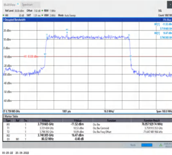
1-N78-3700-3800-30-80-H-2-DFT-PI2BPSK-Outer_F ull-216@0-Ant1-76.958-80.320-≤80-PASS
