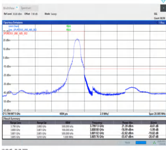
1-N78-3700-3800-30-10-H-5-CP-QPSK-Edge_1RB_Right-1@23-Ant1-1--PASS-see graph
