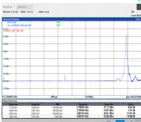
1-N78-3700-3800-PC2-30-90-H-5-CP-QPSK-Edge_1R B_Right-1@244-Ant1-1--PASS-see graph
