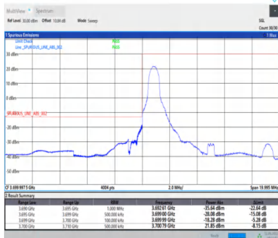
1-N78-3700-3800-PC2-30-10-L-4-CP-QPSK-Edge_1R B_Left-1@0-Ant1-1--PASS-see graph
