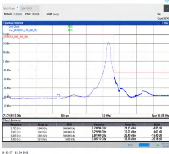
1-N78-3700-3800-PC2-30-20-H-5-CP-QPSK-Edge_1R B_Right-1@50-Ant1-1--PASS-see graph
