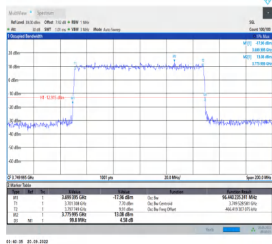
1-N78-3700-3800-30-100-H-3-DFT-16QAM-Outer_F ull-270@0-Ant1-96.44-99.800-≤100-PASS
