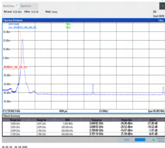
1-N78-3700-3800-PC2-30-80-L-4-CP-QPSK-Edge_1R B_Left-1@0-Ant1-1--PASS-see graph
