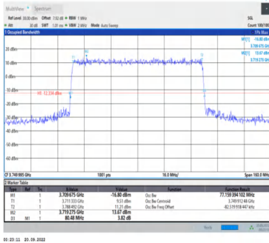
1-N78-3700-3800-30-80-M-3-DFT-16QAM-Outer_Ful I-216@0-Ant1-77.159-80.480-≤80-PASS
