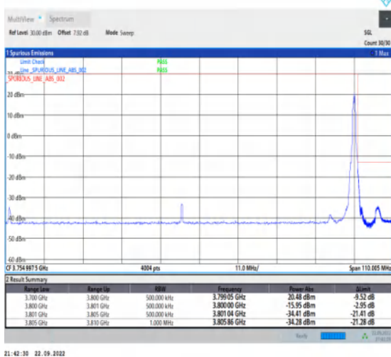
1-N78-3700-3800-30-100-H-5-CP-QPSK-Edge_1RB_Right-1@272-Ant1-1--PASS-see graph
