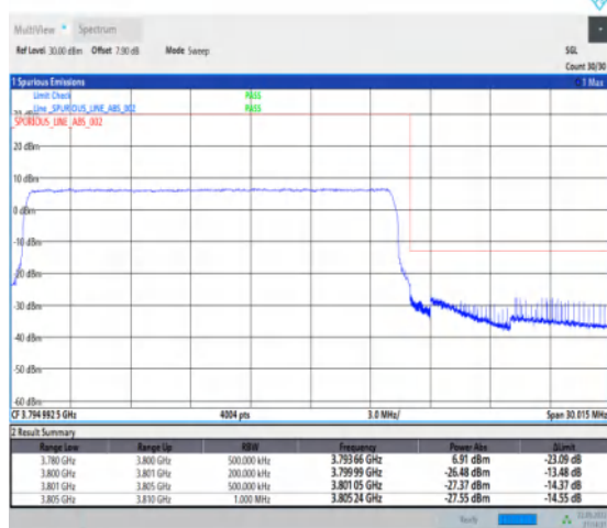
1-N78-3700-3800-30-20-H-6-CP-QPSK-Outer_Full-51@0-Ant1-1--PASS-see graph
