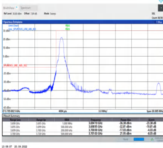
1-N78-3700-3800-30-20-L-4-CP-QPSK-Edge_1RB_Lef t-1@0-Ant1-1--PASS-see graph
