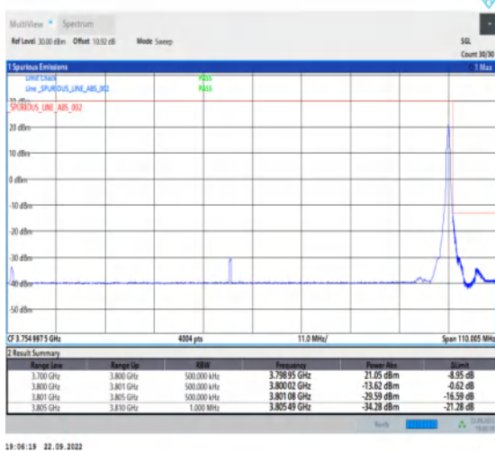
1-N78-3700-3800-PC2-30-100-H-5-CP-QPSK-Edge_1 RB_Right-1@272-Ant1-1--PASS-see graph
