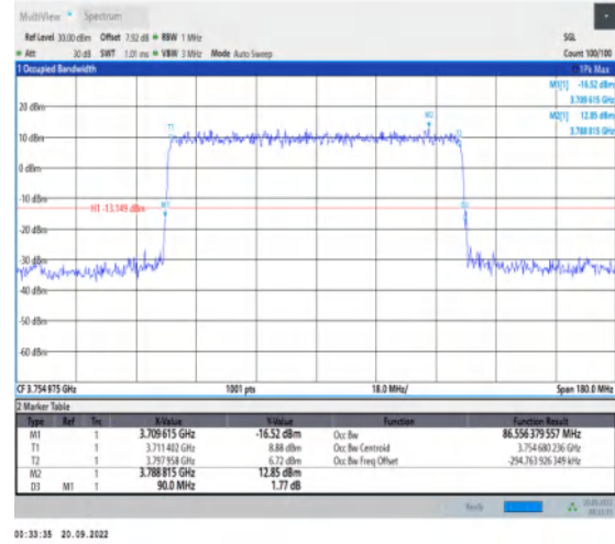
1-N78-3700-3800-30-90-H-4-DFT-64QAM-Outer_Ful I-243@0-Ant1-86.556-90.000-≤90-PASS
