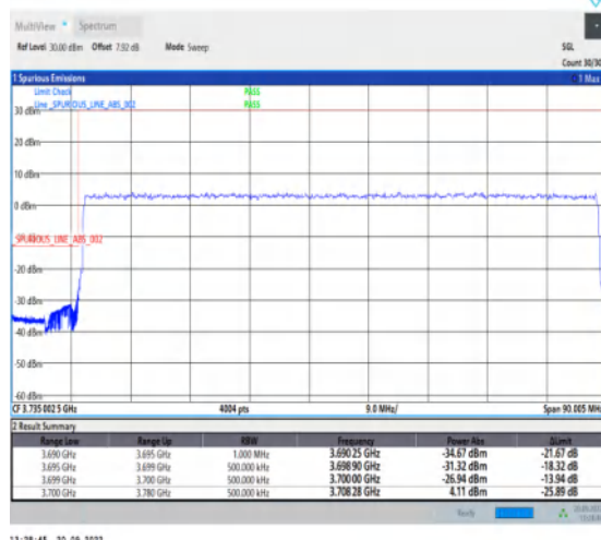
1-N78-3700-3800-30-80-L-3-DFT-PI2BPSK-Outer_Full-216@0-Ant1-1--PASS-see graph
