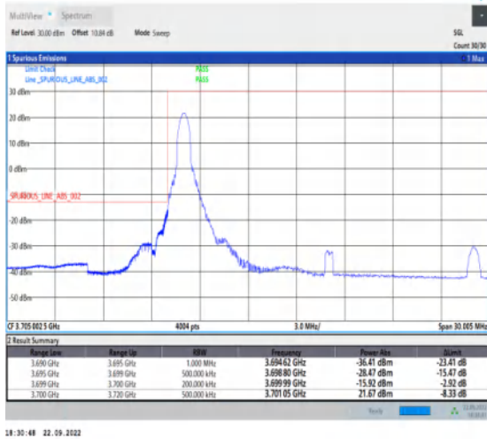
1-N78-3700-3800-PC2-30-20-L-4-CP-QPSK-Edge_1R B_Left-1@0-Ant1-1--PASS-see graph
