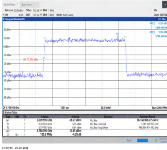
1-N78-3700-3800-30-100-M-5-DFT-256QAM-Outer_Full-270@0-Ant1-96.161-100.000-≤100-PASS
