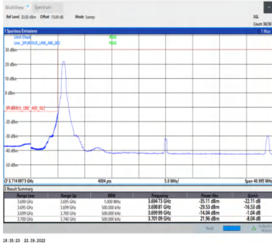
1-N78-3700-3800-PC2-30-40-L-4-CP-QPSK-Edge_1R B_Left-1@0-Ant1-1--PASS-see graph
