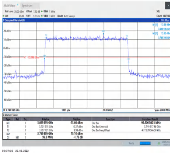
1-N78-3700-3800-30-100-M-1-DFT-QPSK-Outer_Full-I-270@0-Ant1-96.406-99.800-≤100-PASS
