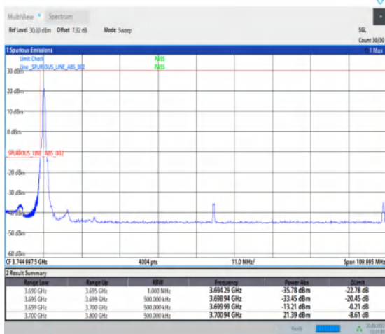
1-N78-3700-3800-30-100-L-4-CP-QPSK-Edge_1RB_Left-1@0-Ant1-1--PASS-see graph
