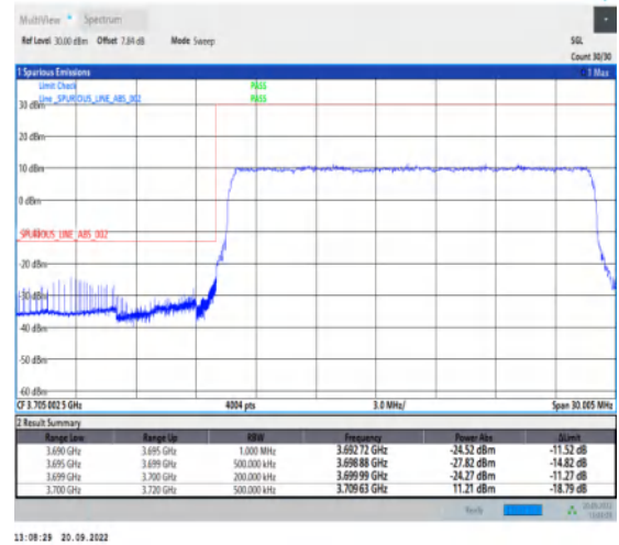
1-N78-3700-3800-30-20-L-3-DFT-PI2BPSK-Outer_Full-50@0-Ant1-1--PASS-see graph
