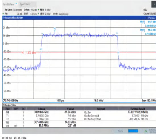
1-N78-3700-3800-30-80-L-4-DFT-64QAM-Outer_Full -216@0-Ant1-77.037-80.000-≤80-PASS
