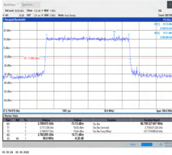
1-N78-3700-3800-30-90-H-3-DFT-16QAM-Outer_Ful I-243@0-Ant1-86.799-90.000-≤90-PASS
