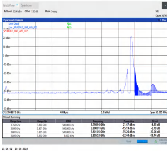
1-N78-3700-3800-30-40-H-2-DFT-PI2BPSK-Edge_1R B_Right-1@105-Ant1-1--PASS-see graph
