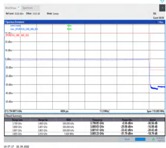
1-N78-3700-3800-PC2-30-100-H-6-CP-QPSK-Out er_Full-273@0-Ant1-1--PASS-see graph
