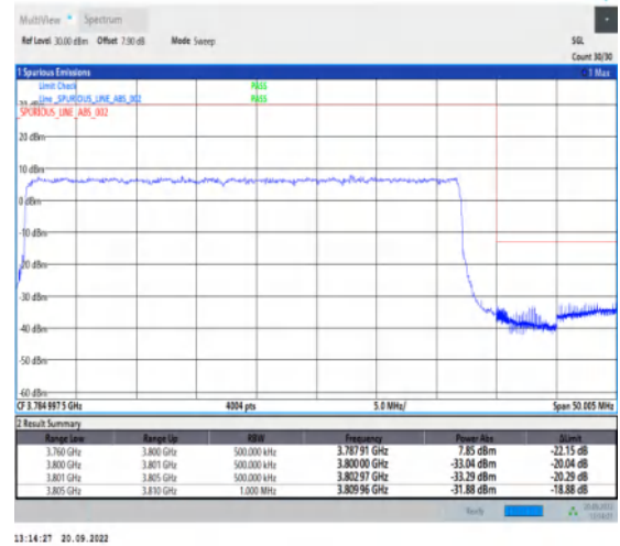
1-N78-3700-3800-30-40-H-3-DFT-PI2BPSK-Outer _Full-100@0-Ant1-1--PASS-see graph
