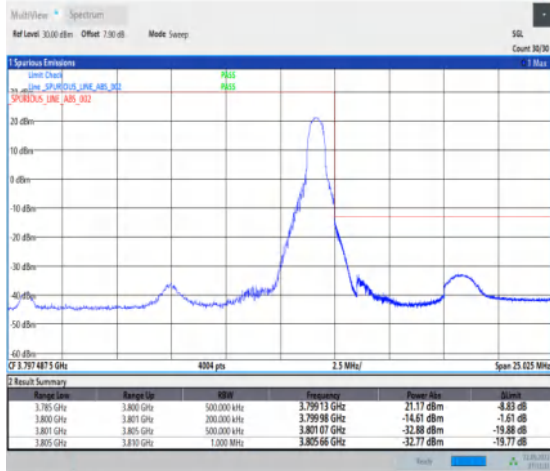
1-N78-3700-3800-30-15-H-2-DFT-PI2BPSK-Edge_1R_B_Right-1@37-Ant1-1--PASS-see graph
