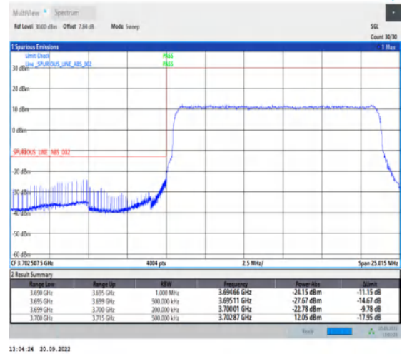
1-N78-3700-3800-30-15-L-3-DFT-PI2BPSK-Outer_Full-36@0-Ant1-1--PASS-see graph
