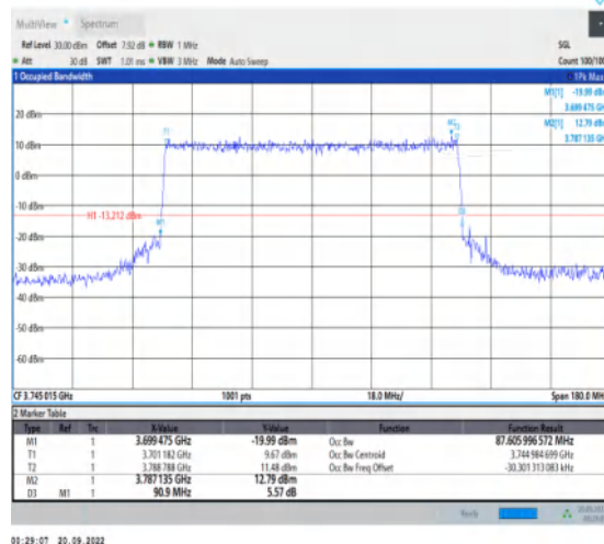
1-N78-3700-3800-30-90-L-6-CP-QPSK-Outter_Full-2 45@0-Ant1-87.606-90.900-≤90-PASS
