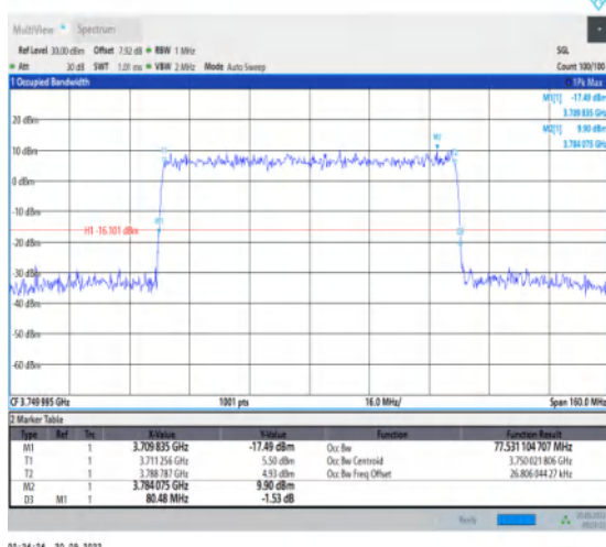
1-N78-3700-3800-30-80-M-9-CP-256QAM-Outer_Ful-I-217@0-Ant1-77.531-80.480-≤80-PASS
