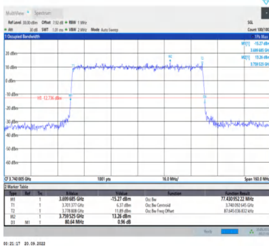
1-N78-3700-3800-30-80-L-6-CP-QPSK-Outer_Full-2 17@0-Ant1-77.431-80.640-≤80-PASS
