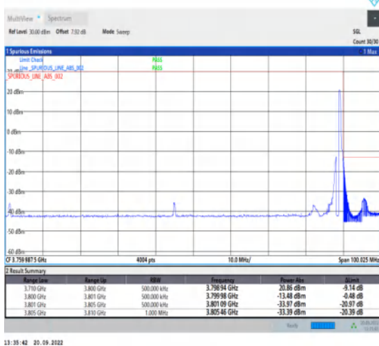
1-N78-3700-3800-30-90-H-5-CP-QPSK-Edge_1RB_Ri ght-1@244-Ant1-1--PASS-see graph
