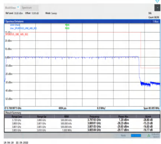
1-N78-3700-3800-PC2-30-70-H-6-CP-QPSK-Outer _Full-189@0-Ant1-1--PASS-see graph
