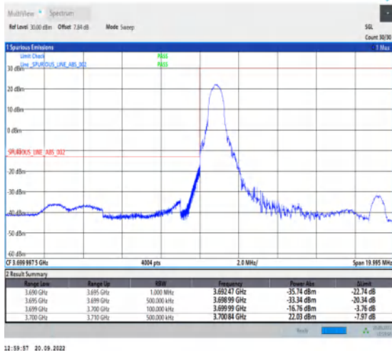
1-N78-3700-3800-30-10-L-4-CP-QPSK-Edge_1RB_Lef t-1@0-Ant1-1--PASS-see graph
