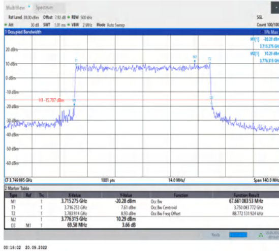
1-N78-3700-3800-30-70-M-6-CP-QPSK-Outer_Full-189@0-Ant1-67.661-69.580-≤70-PASS
