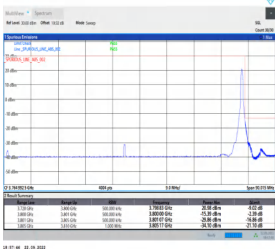
1-N78-3700-3800-PC2-30-80-H-5-CP-QPSK-Edge_1R B_Right-1@216-Ant1-1--PASS-see graph
