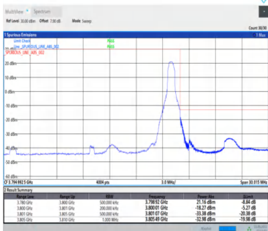
1-N78-3700-3800-30-20-H-2-DFT-PI2BPSK-Edge_1R_B_Right-1@50-Ant1-1--PASS-see graph
