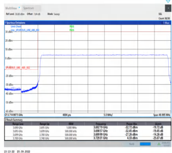
1-N78-3700-3800-30-40-L-6-CP-QPSK-Outer_Full -106@0-Ant1-1--PASS-see graph
