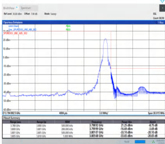
1-N78-3700-3800-30-20-H-5-CP-QPSK-Edge_1RB_Right-1@50-Ant1-1--PASS-see graph
