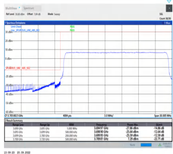
1-N78-3700-3800-30-20-L-6-CP-QPSK-Outer_Full -51@0-Ant1-1--PASS-see graph
