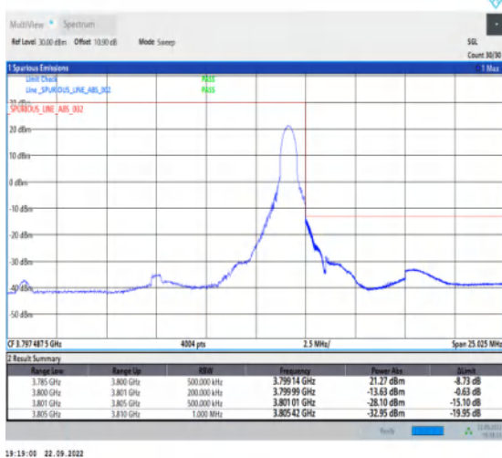
1-N78-3700-3800-PC2-30-15-H-5-CP-QPSK-Edge_1R B_Right-1@37-Ant1-1--PASS-see graph
