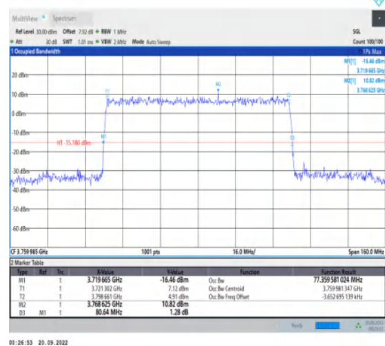
1-N78-3700-3800-30-80-H-9-CP-256QAM-Outter_Full-217@0-Ant1-77.36-80.640-≤80-PASS
