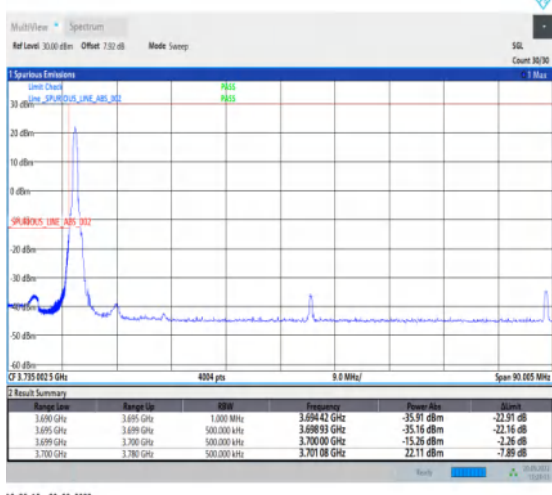
1-N78-3700-3800-30-80-L-4-CP-QPSK-Edge_1RB_Lef t-1@0-Ant1-1--PASS-see graph
