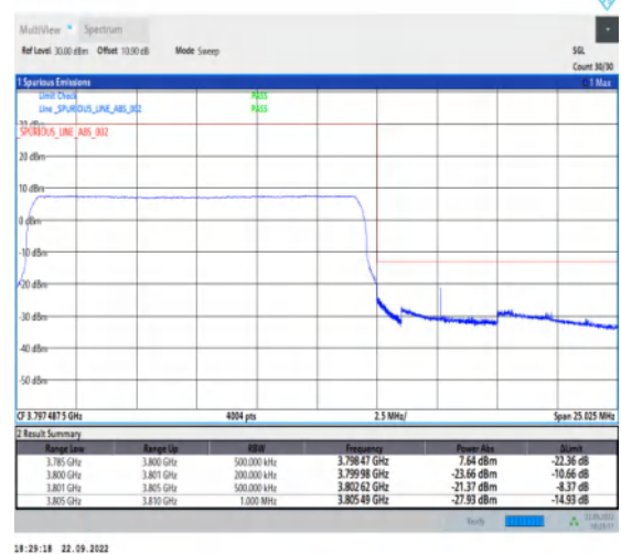
1-N78-3700-3800-PC2-30-15-H-6-CP-QPSK-Outer _Full-38@0-Ant1-1--PASS-see graph
