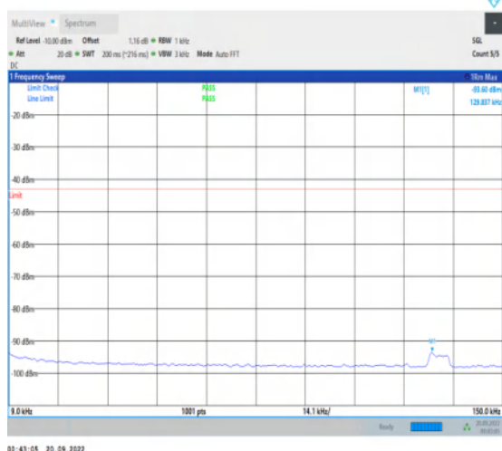
1-N78-3700-3800-30-100-M-1-DFT-PI2BPSK-Inner_1RB_Left-1@1-0.009-0.15-Ant1-0.13--93.60--43-PA SS
