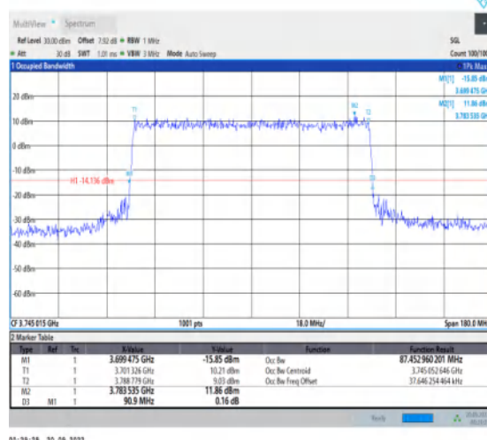
1-N78-3700-3800-30-90-L-8-CP-64QAM-Outter_Full-245@0-Ant1-87.453-90.900-≤90-PASS
