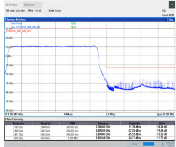
1-N78-3700-3800-30-15-H-3-DFT-PI2BPSK-Outer_Full-36@0-Ant1-1--PASS-see graph
