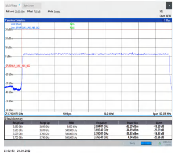
1-N78-3700-3800-30-90-L-3-DFT-PI2BPSK-Outer_Full-243@0-Ant1-1--PASS-see graph
