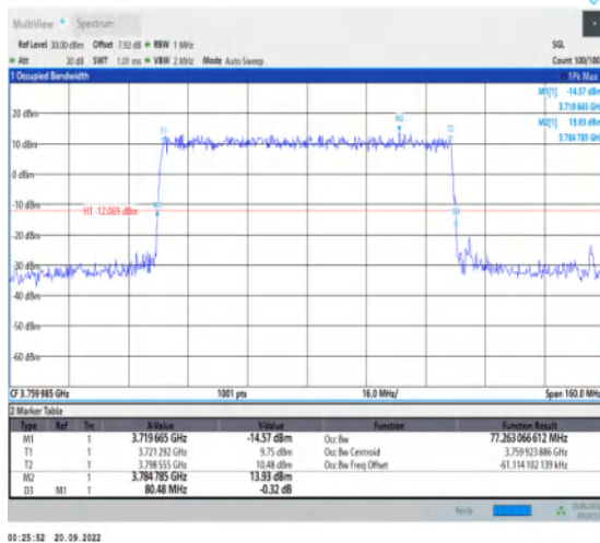
1-N78-3700-3800-30-80-H-4-DFT-64QAM-Outer_Ful I-216@0-Ant1-77.263-80.480-≤80-PASS
