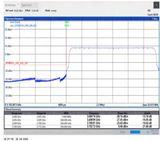
1-N78-3700-3800-PC2-30-15-L-6-CP-QPSK-Outer _Full-38@0-Ant1-1--PASS-see graph
