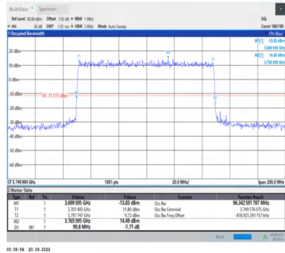
1-N78-3700-3800-30-100-H-1-DFT-QPSK-Outer_Ful l-270@0-Ant1-96.343-99.800-≤100-PASS
