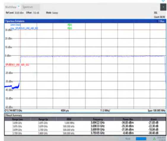
1-N78-3700-3800-30-100-L-6-CP-QPSK-Outer_Full-273@0-Ant1-1--PASS-see graph
