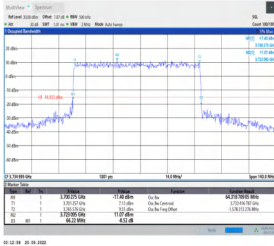
1-N78-3700-3800-30-70-L-3-DFT-16QAM-Outer_Full -180@0-Ant1-64.319-66.220-≤70-PASS
