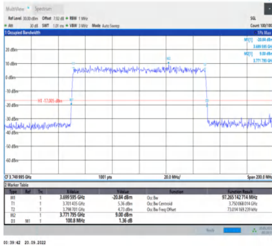
1-N78-3700-3800-30-100-M-9-CP-256QAM-Outer_F ull-273@0-Ant1-97.265-100.800-≤100-PASS
