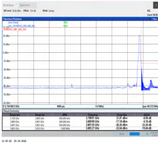
1-N78-3700-3800-30-80-H-2-DFT-PI2BPSK-Edge_1R B_Right-1@216-Ant1-1--PASS-see graph
