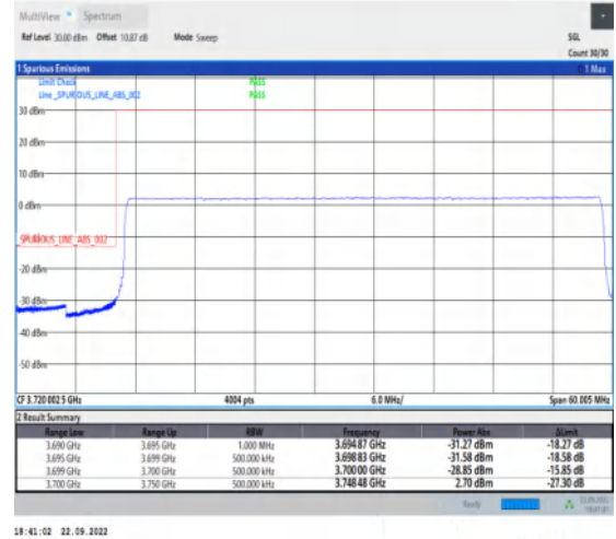
1-N78-3700-3800-PC2-30-50-L-6-CP-QPSK-Outer _Full-133@0-Ant1-1--PASS-see graph
