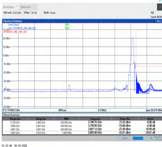
1-N78-3700-3800-30-50-H-5-CP-QPSK-Edge_1RB_Ri ght-1@132-Ant1-1--PASS-see graph
