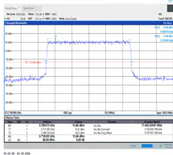
1-N78-3700-3800-30-80-M-6-CP-QPSK-Outer_Full-2 17@0-Ant1-77.443-80.640-≤80-PASS
