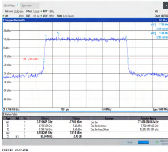
1-N78-3700-3800-30-80-H-6-CP-QPSK-Outter_Full-17@0-Ant1-77.454-80.640-≤80-PASS
