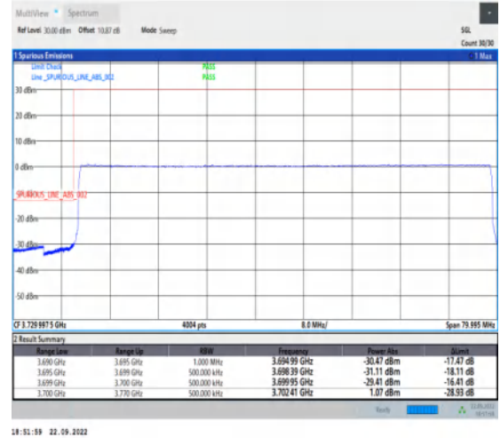
1-N78-3700-3800-PC2-30-70-L-6-CP-QPSK-Outer _Full-189@0-Ant1-1--PASS-see graph
