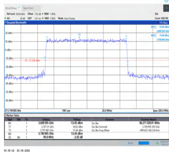
1-N78-3700-3800-30-100-L-1-DFT-QPSK-Outer_Full-270@0-Ant1-96.371-99.800-≤100-PASS
