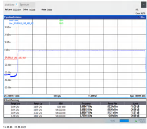
1-N78-3700-3800-PC2-30-100-L-6-CP-QPSK-Out er_Full-273@0-Ant1-1--PASS-see graph
