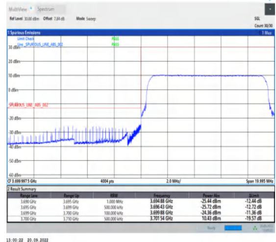
1-N78-3700-3800-30-10-L-6-CP-QPSK-Outer_Full -24@0-Ant1-1--PASS-see graph
