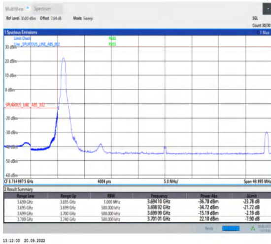
1-N78-3700-3800-30-40-L-1-DFT-PI2BPSK-Edge_1RB_Left-1@0-Ant1-1--PASS-see graph
