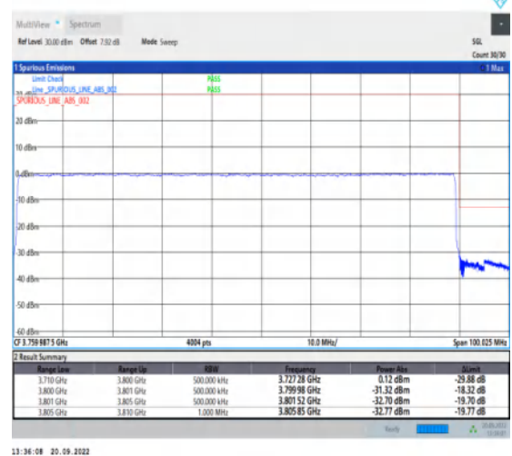
1-N78-3700-3800-30-90-H-6-CP-QPSK-Outer_Full -245@0-Ant1-1--PASS-see graph
