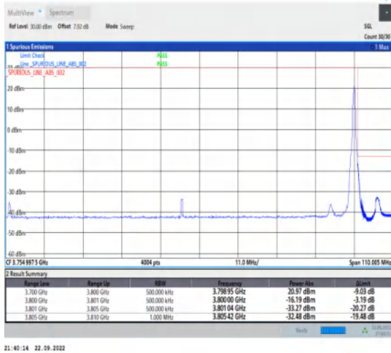
1-N78-3700-3800-30-100-H-2-DFT-PI2BPSK-Edge_1R_B_Right-1@272-Ant1-1--PASS-see graph
