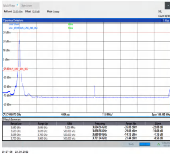
1-N78-3700-3800-PC2-30-100-L-4-CP-QPSK-Edge_1 RB_Left-1@0-Ant1-1--PASS-see graph
