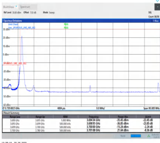
1-N78-3700-3800-30-80-L-1-DFT-PI2BPSK-Edge_1RB_Left-1@0-Ant1-1--PASS-see graph
