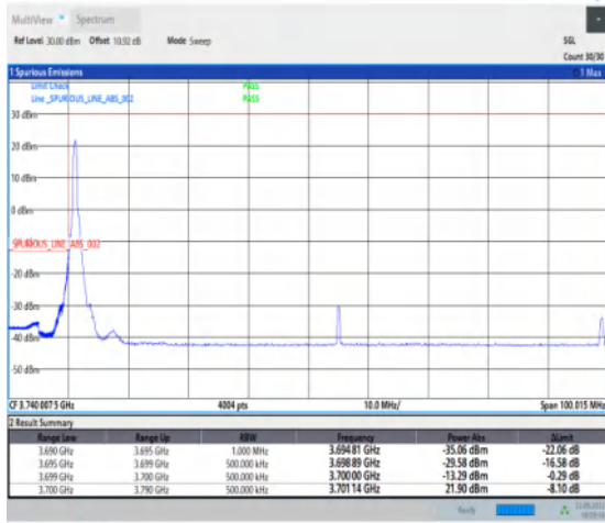
1-N78-3700-3800-PC2-30-90-L-4-CP-QPSK-Edge_1R B_Left-1@0-Ant1-1--PASS-see graph
