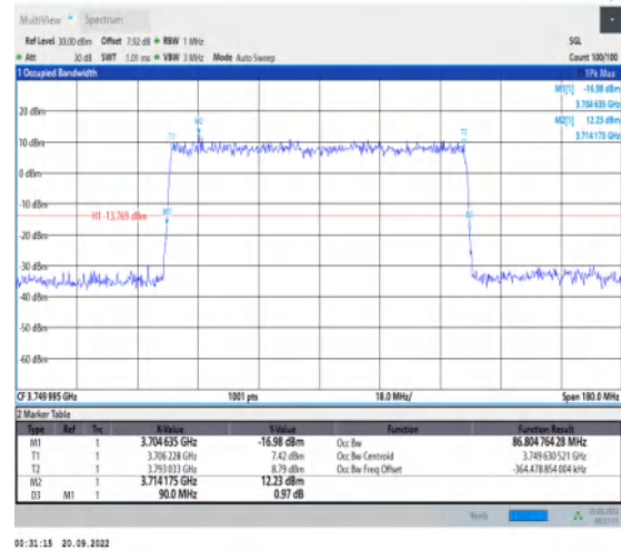
1-N78-3700-3800-30-90-M-5-DFT-256QAM-Outer_Full I-243@0-Ant1-86.805-90.000≤90-PASS
