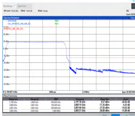
1-N78-3700-3800-PC2-30-10-H-6-CP-QPSK-Outer _Full-24@0-Ant1-1--PASS-see graph
