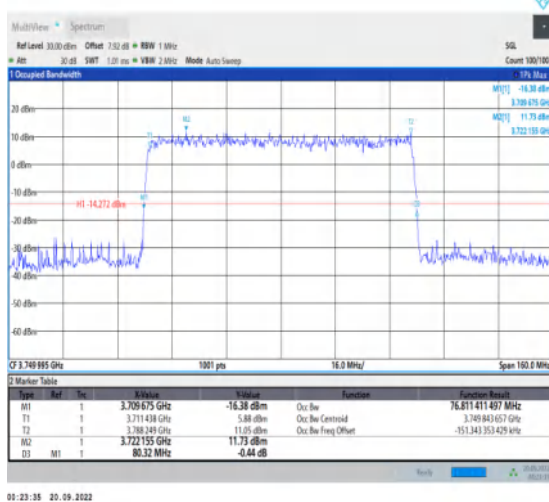
1-N78-3700-3800-30-80-M-5-DFT-256QAM-Outer_F ull-216@0-Ant1-76.811-80.320-≤80-PASS
