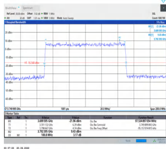
1-N78-3700-3800-30-100-L-9-CP-256QAM-Outter_Full-273@0-Ant1-97.535-100.800-≤100-PASS
