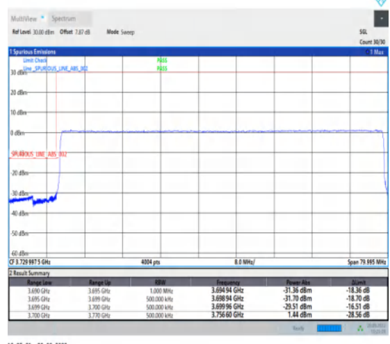
1-N78-3700-3800-30-70-L-6-CP-QPSK-Outer_Full -189@0-Ant1-1--PASS-see graph
