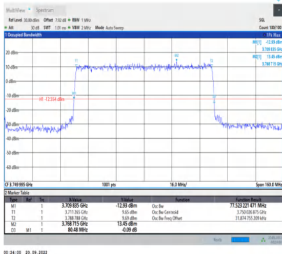
1-N78-3700-3800-30-80-M-7-CP-16QAM-Outer_Full-217@0-Ant1-77.523-80.480-≤80-PASS
