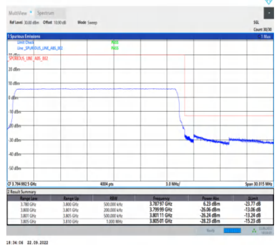
1-N78-3700-3800-PC2-30-20-H-6-CP-QPSK-Outer _Full-51@0-Ant1-1--PASS-see graph
