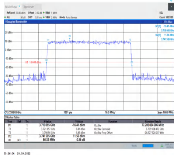
1-N78-3700-3800-30-80-H-5-DFT-256QAM-Outer_F ull-216@0-Ant1-77.203-80.320-≤80-PASS
