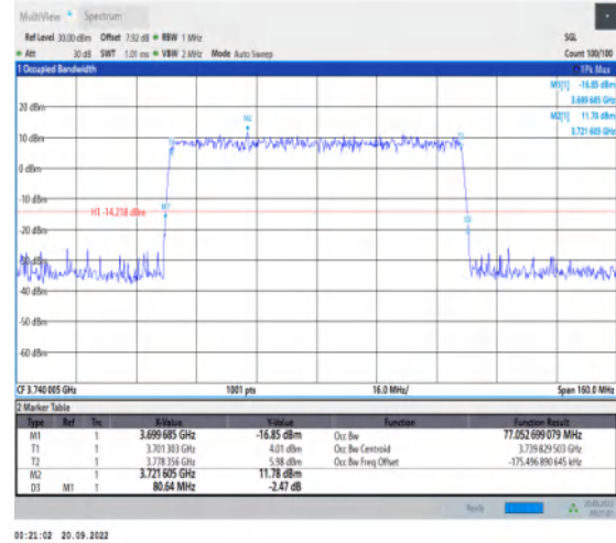
1-N78-3700-3800-30-80-L-5-DFT-256QAM-Outer_F ull-216@0-Ant1-77.053-80.640-≤80-PASS
