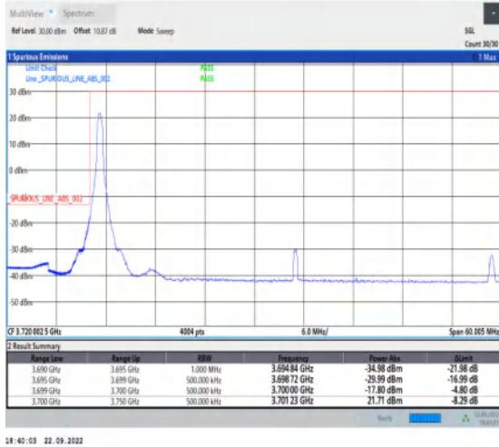
1-N78-3700-3800-PC2-30-50-L-4-CP-QPSK-Edge_1R B_Left-1@0-Ant1-1--PASS-see graph
