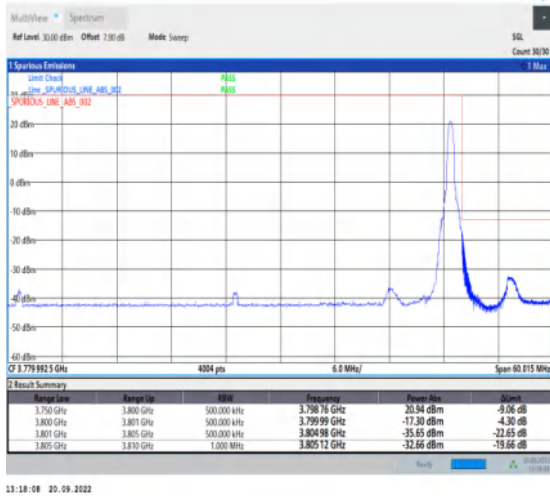
1-N78-3700-3800-30-50-H-2-DFT-PI2BPSK-Edge_1R B_Right-1@132-Ant1-1--PASS-see graph
