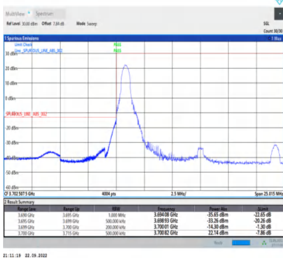
1-N78-3700-3800-30-15-L-4-CP-QPSK-Edge_1RB_Lef t-1@0-Ant1-1--PASS-see graph
