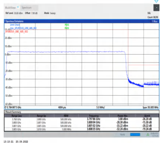
1-N78-3700-3800-30-40-H-6-CP-QPSK-Outer_Full -106@0-Ant1-1--PASS-see graph
