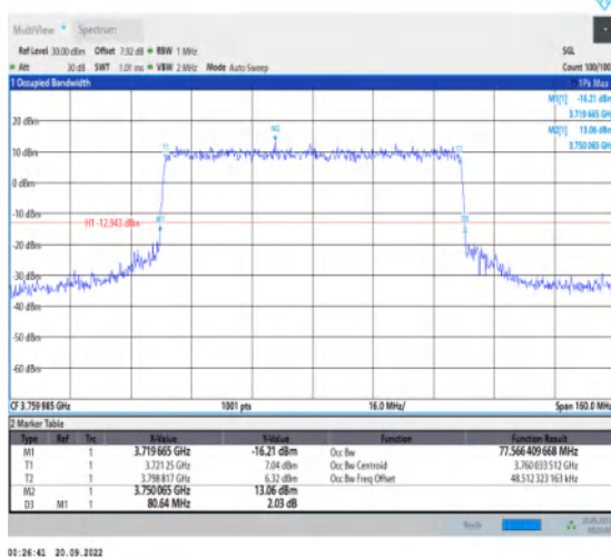
1-N78-3700-3800-30-80-H-8-CP-64QAM-Outter_Full-217@0-Ant1-77.566-80.640-≤80-PASS
