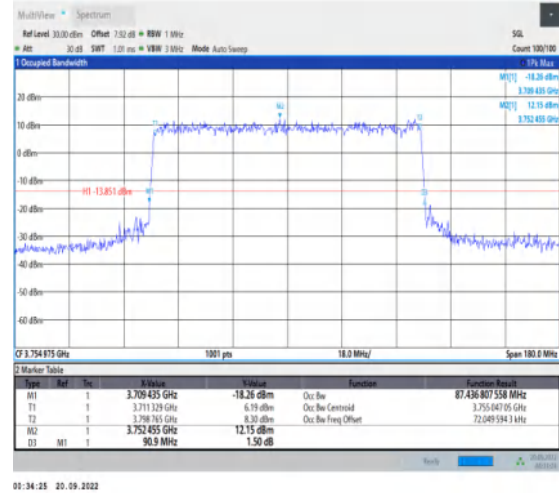
1-N78-3700-3800-30-90-H-8-CP-64QAM-Outer_Full-245@0-Ant1-87.437-90.900-≤90-PASS
