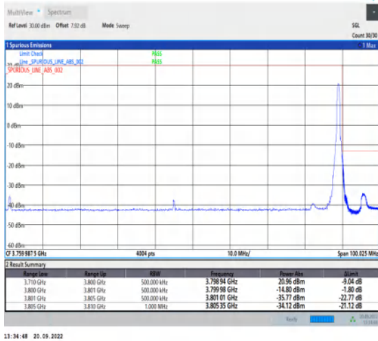
1-N78-3700-3800-30-90-H-2-DFT-PI2BPSK-Edge_1R B_Right-1@244-Ant1-1--PASS-see graph
