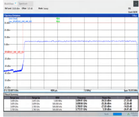
1-N78-3700-3800-30-60-L-3-DFT-PI2BPSK-Outer_Full-162@0-Ant1-1--PASS-see graph
