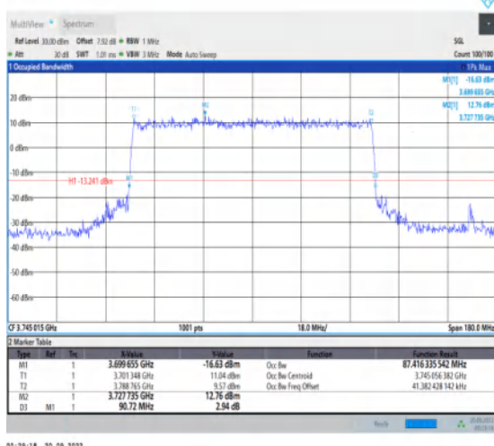
1-N78-3700-3800-30-90-L-7-CP-16QAM-Outter_Full-245@0-Ant1-87.416-90.720-≤90-PASS
