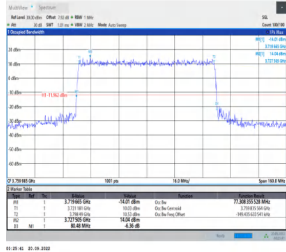
1-N78-3700-3800-30-80-H-3-DFT-16QAM-Outer_Ful I-216@0-Ant1-77.308-80.480-≤80-PASS
