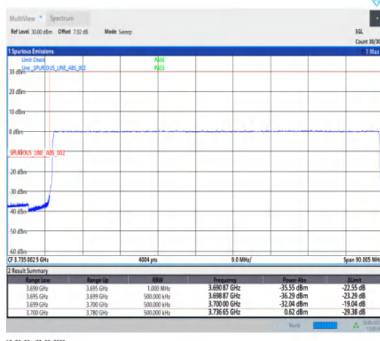
1-N78-3700-3800-30-80-L-6-CP-QPSK-Outer_Full_-217@0-Ant1-1--PASS-see graph
