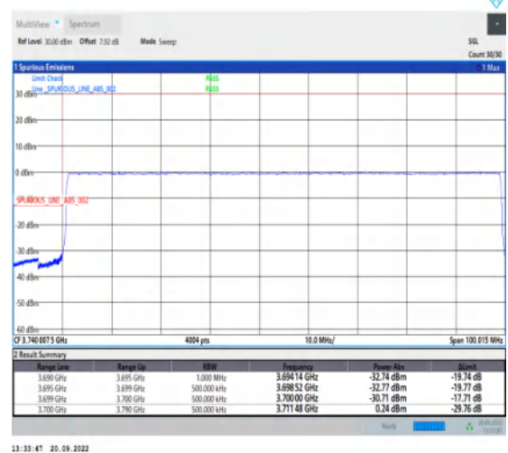
1-N78-3700-3800-30-90-L-6-CP-QPSK-Outer_Full -245@0-Ant1-1--PASS-see graph
