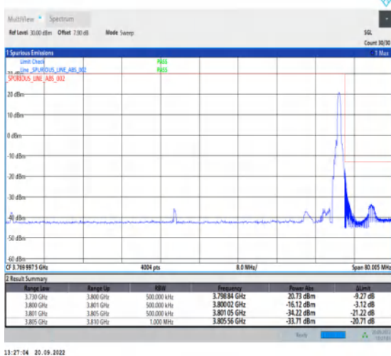
1-N78-3700-3800-30-70-H-5-CP-QPSK-Edge_1RB_Ri ght-1@188-Ant1-1--PASS-see graph
