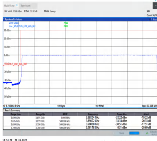
1-N78-3700-3800-PC2-30-80-L-6-CP-QPSK-Outer _Full-217@0-Ant1-1--PASS-see graph
