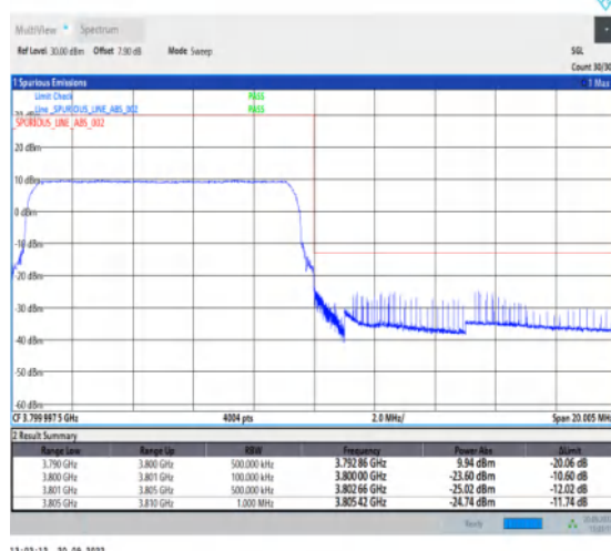
1-N78-3700-3800-30-10-H-6-CP-QPSK-Outer_Full-24@0-Ant1-1--PASS-see graph
