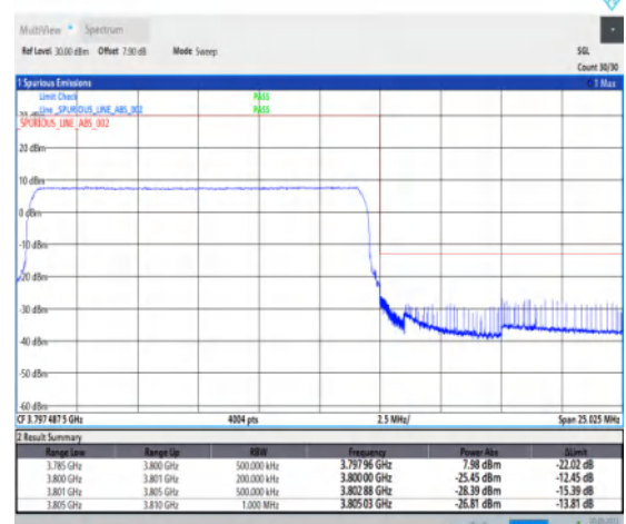
1-N78-3700-3800-30-15-H-6-CP-QPSK-Outer_Full-38@0-Ant1-1--PASS-see graph
