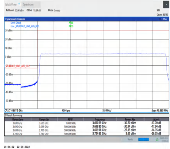
1-N78-3700-3800-PC2-30-40-L-6-CP-QPSK-Outer _Full-106@0-Ant1-1--PASS-see graph
