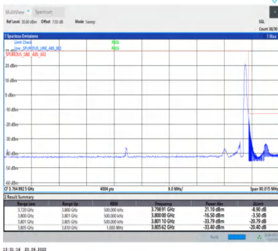
1-N78-3700-3800-30-80-H-5-CP-QPSK-Edge_1RB_Ri ght-1@216-Ant1-1--PASS-see graph
