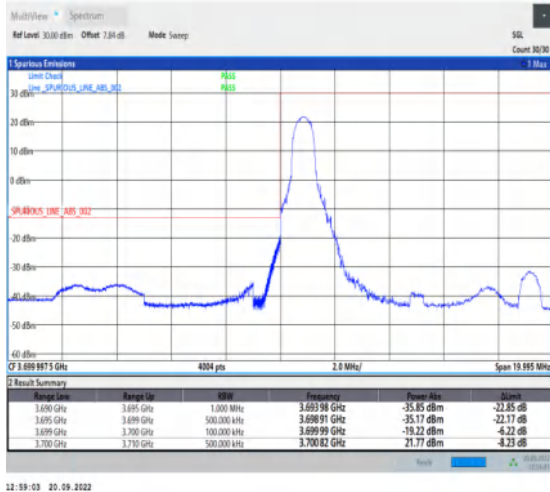
1-N78-3700-3800-30-10-L-1-DFT-PI2BPSK-Edge_1RB _Left-1@0-Ant1-1--PASS-see graph
