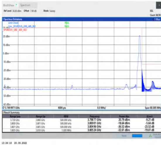
1-N78-3700-3800-30-70-H-2-DFT-PI2BPSK-Edge_1R B_Right-1@188-Ant1-1--PASS-see graph
