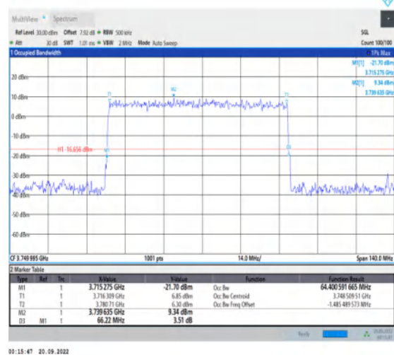
1-N78-3700-3800-30-70-M-5-DFT-256QAM-Outer_Full-180@0-Ant1-64.401-66.220-≤70-PASS
