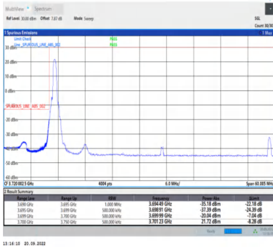
1-N78-3700-3800-30-50-L-1-DFT-PI2BPSK-Edge_1RB _Left-1@0-Ant1-1--PASS-see graph
