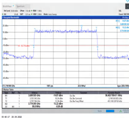
1-N78-3700-3800-30-100-H-2-DFT-PI2BPSK-Outer_F ull-270@0-Ant1-96.404-99.800-≤100-PASS
