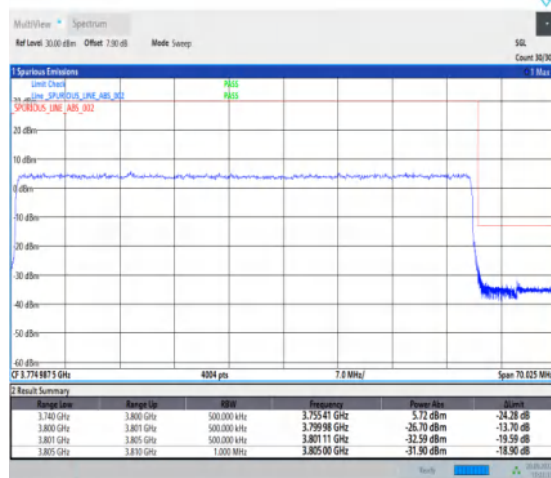
1-N78-3700-3800-30-60-H-3-DFT-PI2BPSK-Outer _Full-162@0-Ant1-1--PASS-see graph
