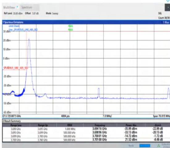
1-N78-3700-3800-30-60-L-4-CP-QPSK-Edge_1RB_Lef t-1@0-Ant1-1--PASS-see graph
