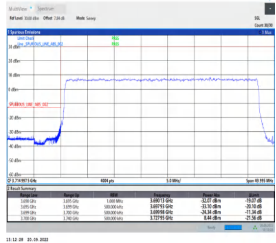
1-N78-3700-3800-30-40-L-3-DFT-PI2BPSK-Outer_Full-100@0-Ant1-1--PASS-see graph
