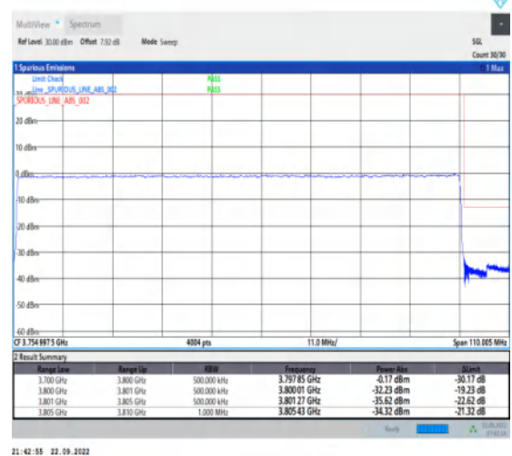
1-N78-3700-3800-30-100-H-6-CP-QPSK-Outer_Full-273@0-Ant1-1--PASS-see graph
