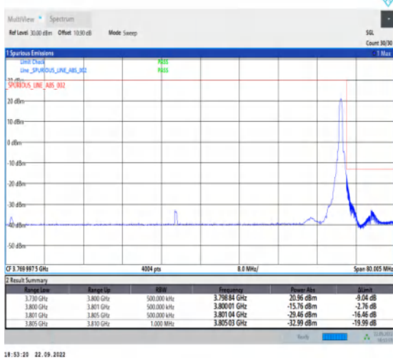
1-N78-3700-3800-PC2-30-70-H-5-CP-QPSK-Edge_1R B_Right-1@188-Ant1-1--PASS-see graph
