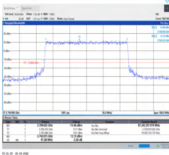
1-N78-3700-3800-30-90-M-6-CP-QPSK-Outer_Full-2 45@0-Ant1-87.342-91.080≤90-PASS
