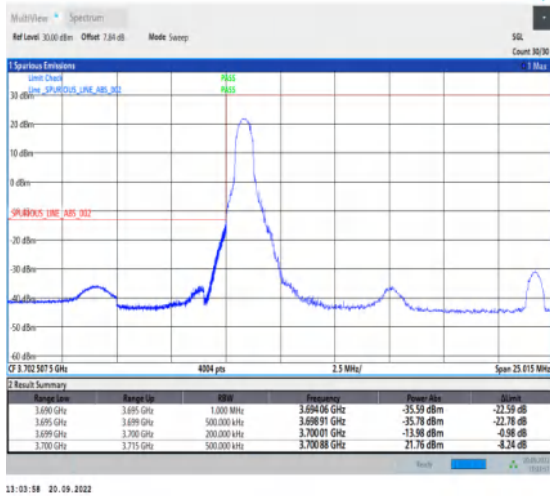
1-N78-3700-3800-30-15-L-1-DFT-PI2BPSK-Edge_1RB_Left-1@0-Ant1-1--PASS-see graph
