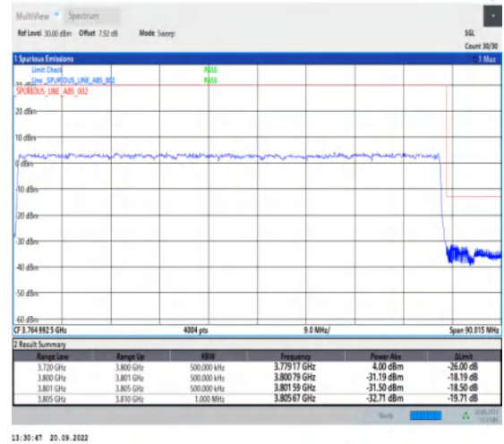
1-N78-3700-3800-30-80-H-3-DFT-PI2BPSK-Outer _Full-216@0-Ant1-1--PASS-see graph
