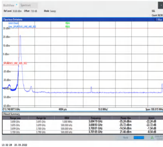
1-N78-3700-3800-30-90-L-1-DFT-PI2BPSK-Edge_1RB_Left-1@0-Ant1-1--PASS-see graph
