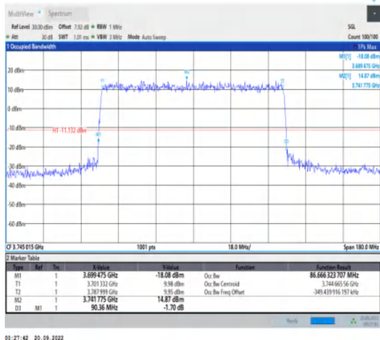
1-N78-3700-3800-30-90-L-1-DFT-QPSK-Outer_Full-243@0-Ant1-86.666-90.360-≤90-PASS
