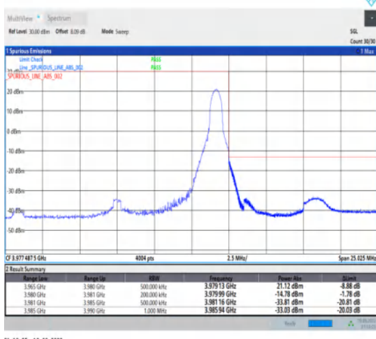
1-N77-3700-3980--30-15-H-5-CP-QPSK-Edge_1RB_R ight-1@37-Ant1-1--PASS-see graph
