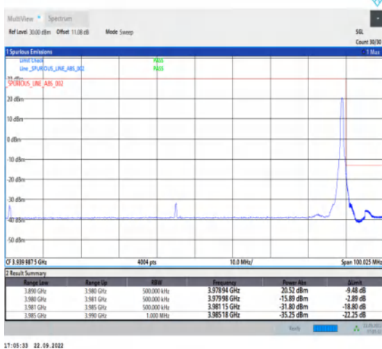
1-N77-3700-3980-PC2-30-90-H-5-CP-QPSK-Edge_1R B_Right-1@244-Ant1-1--PASS-see graph
