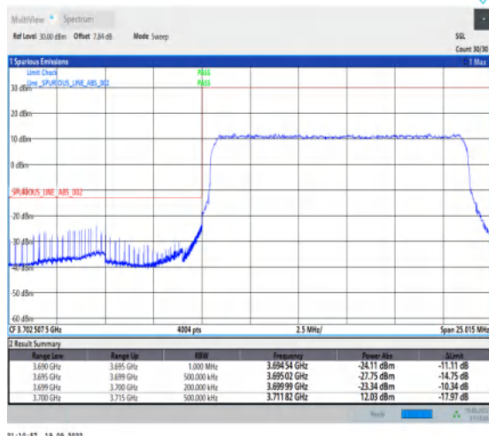
1-N77-3700-3980--30-15-L-3-DFT-PI2BPSK-Outer_Full-36@0-Ant1-1--PASS-see graph
