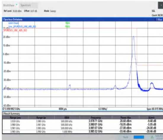
1-N77-3700-3980--30-50-H-2-DFT-PI2BPSK-Edge_1R B_Right-1@132-Ant1-1--PASS-see graph
