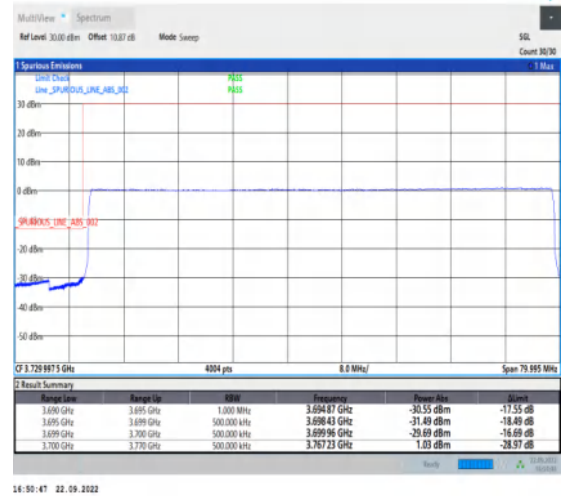
1-N77-3700-3980-PC2-30-70-L-6-CP-QPSK-Outer _Full-189@0-Ant1-1--PASS-see graph
