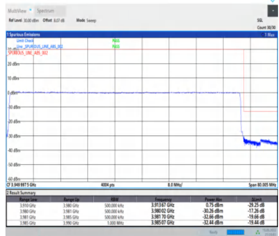
1-N77-3700-3980--30-70-H-6-CP-QPSK-Outer_Ful l-189@0-Ant1-1--PASS-see graph
