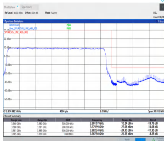
1-N77-3700-3980--30-20-H-3-DFT-PI2BPSK-Outer_Full-50@0-Ant1-1--PASS-see graph
