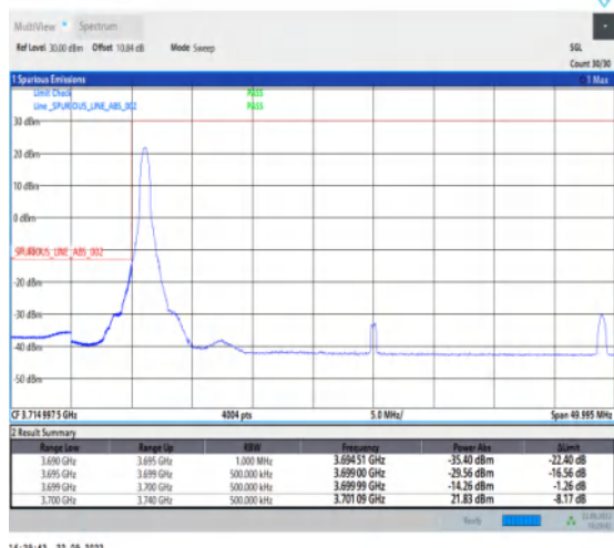
1-N77-3700-3980-PC2-30-40-L-4-CP-QPSK-Edge_1R B_Left-1@0-Ant1-1--PASS-see graph
