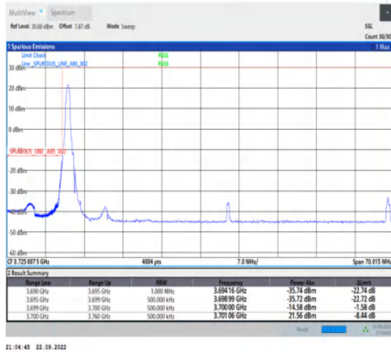
1-N77-3700-3980--30-60-L-1-DFT-PI2BPSK-Edge_1R_B_Left-1@0-Ant1-1--PASS-see graph
