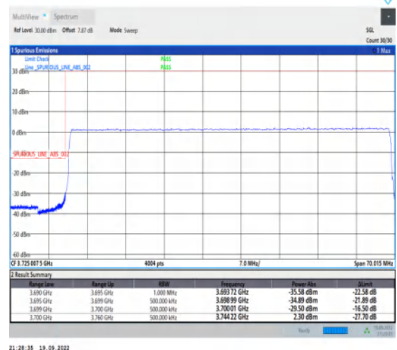
1-N77-3700-3980--30-60-L-6-CP-QPSK-Outer_Full-162@0-Ant1-1--PASS-see graph
