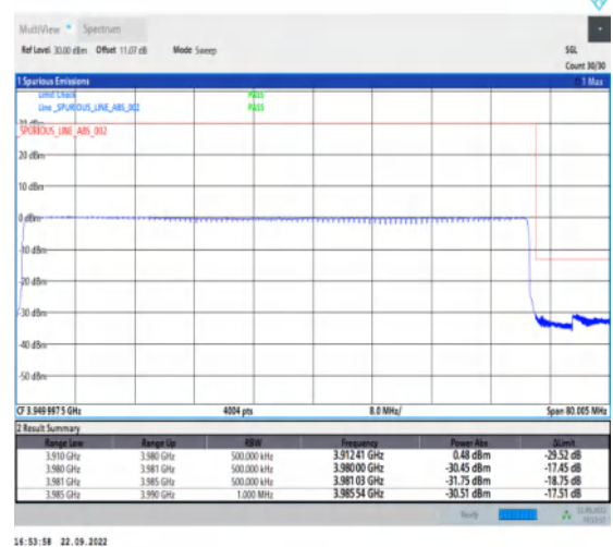
1-N77-3700-3980-PC2-30-70-H-6-CP-QPSK-Outer _Full-189@0-Ant1-1--PASS-see graph
