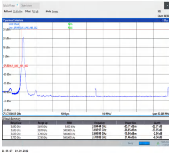
1-N77-3700-3980--30-80-L-1-DFT-PI2BPSK-Edge_1R_B_Left-1@0-Ant1-1--PASS-see graph
