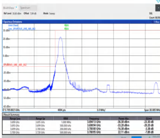
1-N77-3700-3980--30-20-L-4-CP-QPSK-Edge_1RB_Left-1@0-Ant1-1--PASS-see graph
