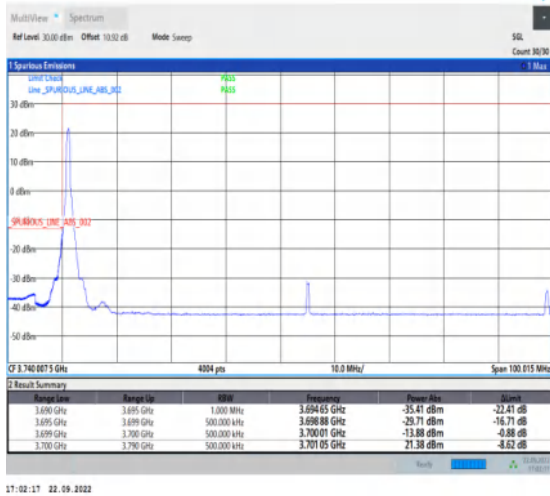
1-N77-3700-3980-PC2-30-90-L-4-CP-QPSK-Edge_1R B_Left-1@0-Ant1-1--PASS-see graph
