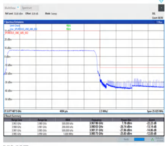
1-N77-3700-3980--30-15-H-6-CP-QPSK-Outer_Ful l-38@0-Ant1-1--PASS-see graph
