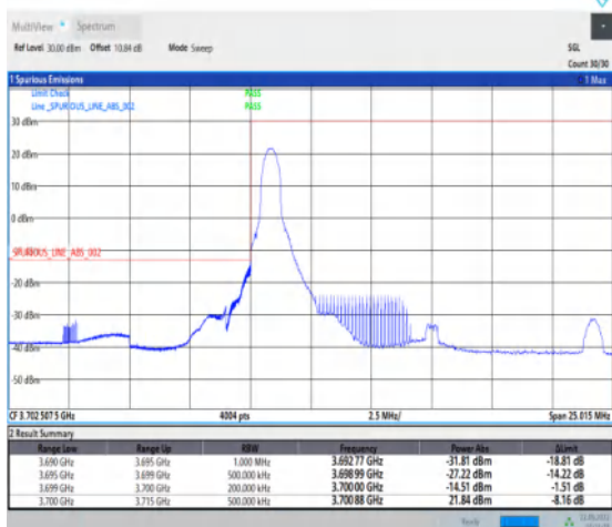
1-N77-3700-3980-PC2-30-15-L-4-CP-QPSK-Edge_1R B_Left-1@0-Ant1-1--PASS-see graph
