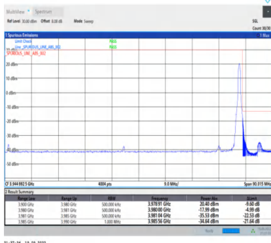
1-N77-3700-3980--30-80-H-2-DFT-PI2BPSK-Edge_1R B_Right-1@216-Ant1-1--PASS-see graph
