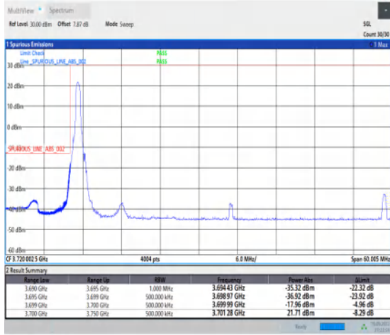
1-N77-3700-3980--30-50-L-1-DFT-PI2BPSK-Edge_1R_B_Left-1@0-Ant1-1--PASS-see graph
