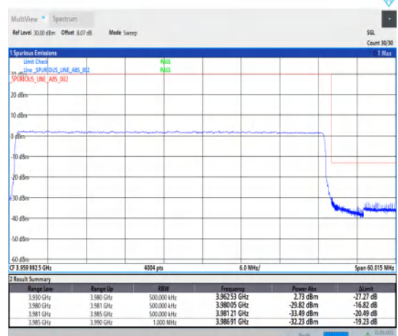
1-N77-3700-3980--30-50-H-6-CP-QPSK-Outer_Ful l-133@0-Ant1-1--PASS-see graph
