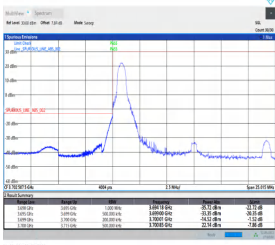
1-N77-3700-3980--30-15-L-4-CP-QPSK-Edge_1RB_Left-1@0-Ant1-1--PASS-see graph
