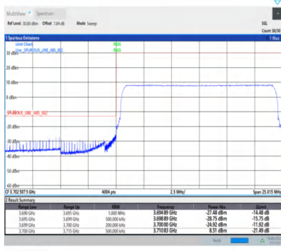
1-N77-3700-3980--30-15-L-6-CP-QPSK-Outer_Full-38@0-Ant1-1--PASS-see graph
