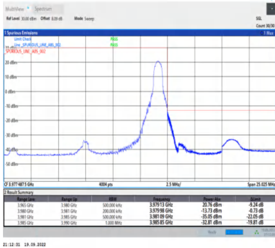
1-N77-3700-3980--30-15-H-2-DFT-PI2BPSK-Edge_1R_B_Right-1@37-Ant1-1--PASS-see graph
