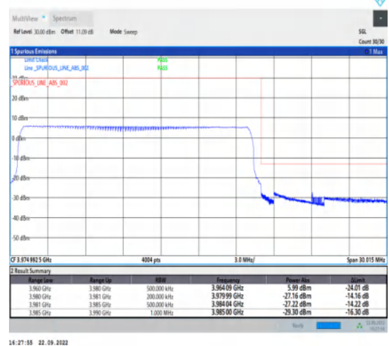
1-N77-3700-3980-PC2-30-20-H-6-CP-QPSK-Outer _Full-51@0-Ant1-1--PASS-see graph
