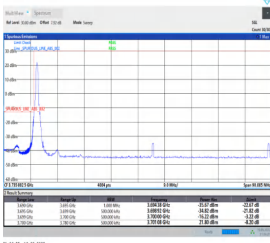
1-N77-3700-3980--30-80-L-4-CP-QPSK-Edge_1RB_Left-1@0-Ant1-1--PASS-see graph
