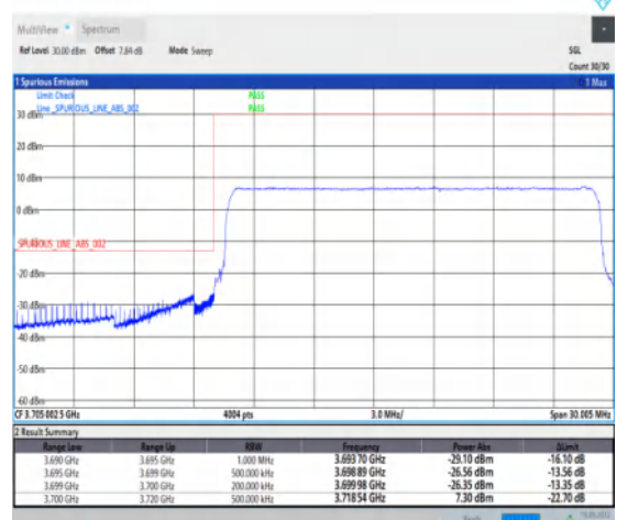
1-N77-3700-3980--30-20-L-6-CP-QPSK-Outer_Full-51@0-Ant1-1--PASS-see graph
