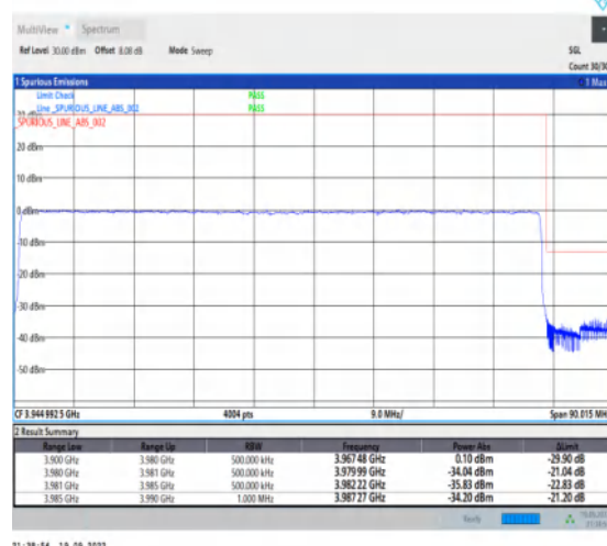
1-N77-3700-3980--30-80-H-6-CP-QPSK-Outer_Ful I-217@0-Ant1-1--PASS-see graph
