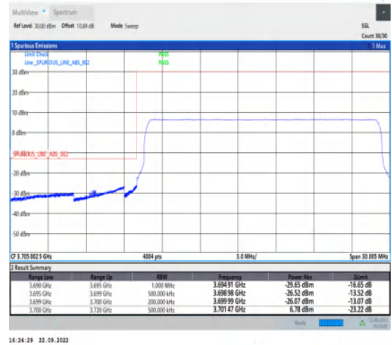
1-N77-3700-3980-PC2-30-20-L-6-CP-QPSK-Outer _Full-51@0-Ant1-1--PASS-see graph
