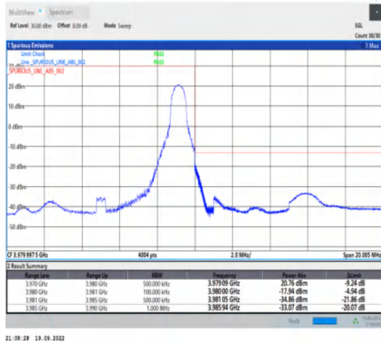
1-N77-3700-3980--30-10-H-2-DFT-PI2BPSK-Edge_1R_B_Right-1@23-Ant1-1--PASS-see graph
