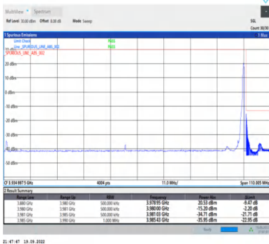
1-N77-3700-3980--30-100-H-5-CP-QPSK-Edge_1RB Right-1@272-Ant1-1--PASS-see graph
