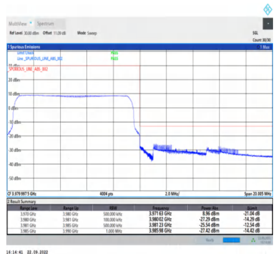
1-N77-3700-3980-PC2-30-10-H-6-CP-QPSK-Outer _Full-24@0-Ant1-1--PASS-see graph
