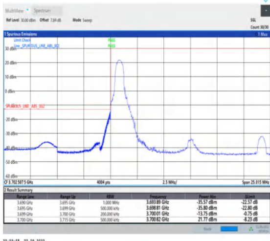
1-N77-3700-3980--30-15-L-1-DFT-PI2BPSK-Edge_1R_B_Left-1@0-Ant1-1--PASS-see graph
