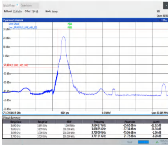
1-N77-3700-3980--30-20-L-1-DFT-PI2BPSK-Edge_1R_B_Left-1@0-Ant1-1--PASS-see graph
