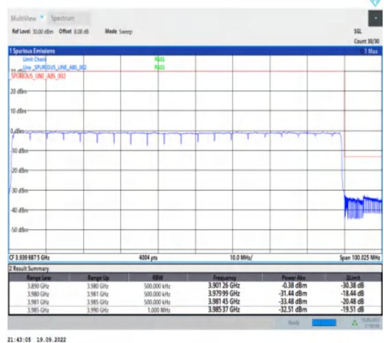
1-N77-3700-3980--30-90-H-6-CP-QPSK-Outer_Ful l-245@0-Ant1-1--PASS-see graph
