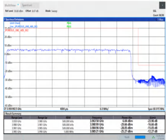
1-N77-3700-3980--30-50-H-3-DFT-PI2BPSK-Outer _Full-128@0-Ant1-1--PASS-see graph
