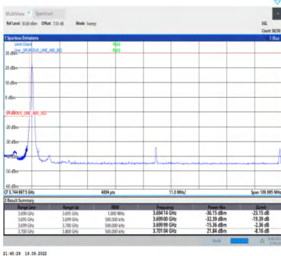
1-N77-3700-3980--30-100-L-4-CP-QPSK-Edge_1RB_Left-1@0-Ant1-1--PASS-see graph
