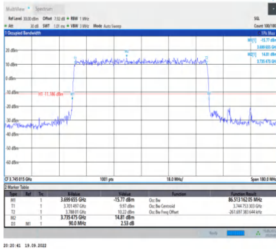
1-N77-3700-3980--30-90-L-1-DFT-QPSK-Outer_Full -243@0-Ant1-86.513-90.000-≤90-PASS
