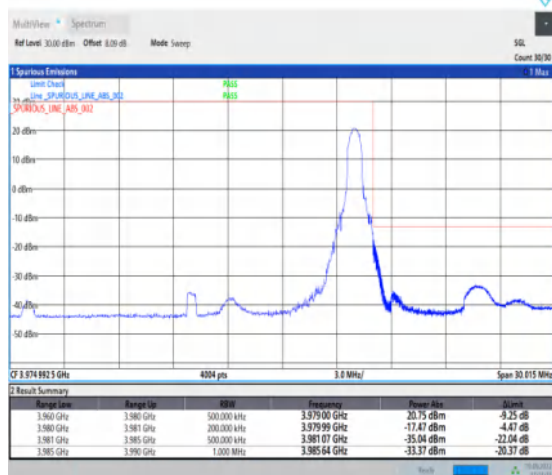
1-N77-3700-3980--30-20-H-2-DFT-PI2BPSK-Edge_1R_B_Right-1@50-Ant1-1--PASS-see graph
