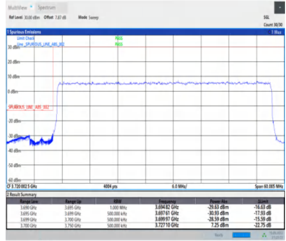
1-N77-3700-3980--30-50-L-3-DFT-PI2BPSK-Outer_Full-128@0-Ant1-1--PASS-see graph
