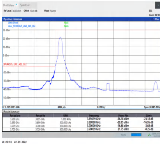
1-N77-3700-3980-PC2-30-20-L-4-CP-QPSK-Edge_1R B_Left-1@0-Ant1-1--PASS-see graph
