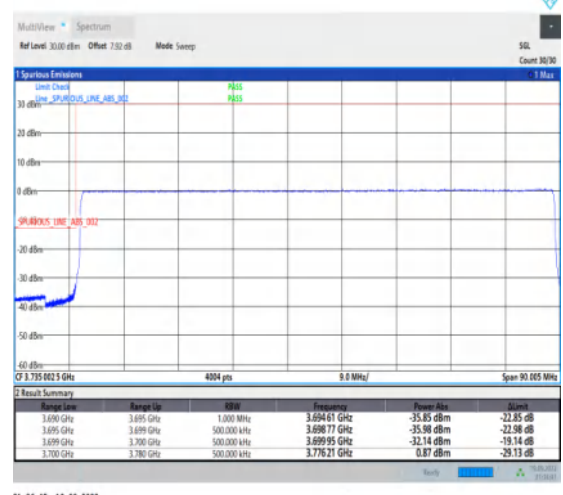
1-N77-3700-3980--30-80-L-6-CP-QPSK-Outer_Full-217@0-Ant1-1--PASS-see graph
