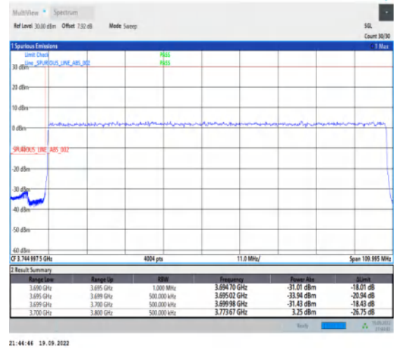
1-N77-3700-3980--30-100-L-3-DFT-PI2BPSK-Outer_Full-270@0-Ant1-1--PASS-see graph
