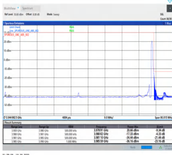
1-N77-3700-3980--30-80-H-5-CP-QPSK-Edge_1RB_R ight-1@216-Ant1-1--PASS-see graph
