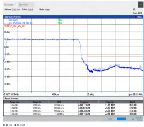
1-N77-3700-3980--30-15-H-3-DFT-PI2BPSK-Outer_Full-36@0-Ant1-1--PASS-see graph
