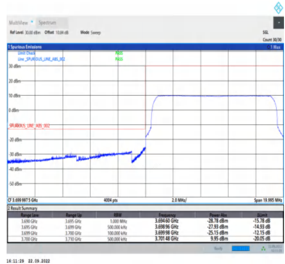
1-N77-3700-3980-PC2-30-10-L-6-CP-QPSK-Outer _Full-24@0-Ant1-1--PASS-see graph
