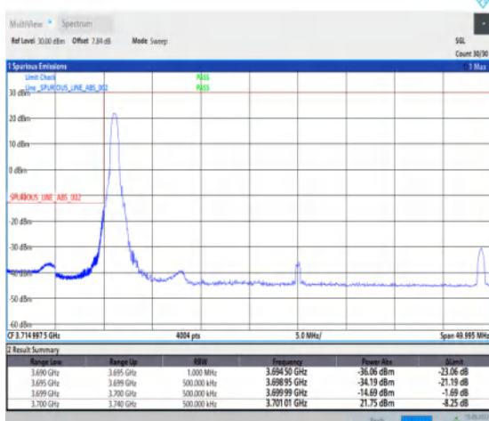
1-N77-3700-3980--30-40-L-4-CP-QPSK-Edge_1RB_Left-1@0-Ant1-1--PASS-see graph
