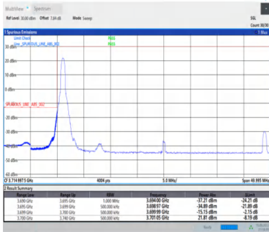
1-N77-3700-3980--30-40-L-1-DFT-PI2BPSK-Edge_1R_B_Left-1@0-Ant1-1--PASS-see graph
