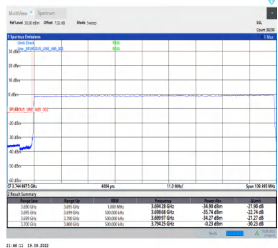
1-N77-3700-3980--30-100-L-6-CP-QPSK-Outer_Full-273@0-Ant1-1--PASS-see graph
