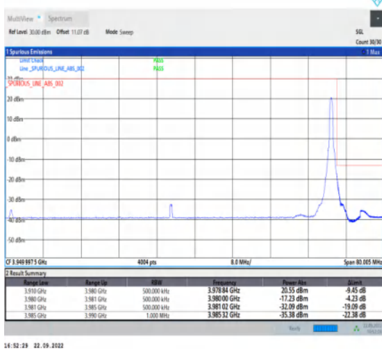
1-N77-3700-3980-PC2-30-70-H-5-CP-QPSK-Edge_1R B_Right-1@188-Ant1-1--PASS-see graph
