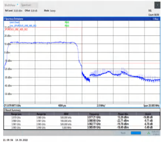
1-N77-3700-3980--30-10-H-3-DFT-PI2BPSK-Outer_Full-24@0-Ant1-1--PASS-see graph
