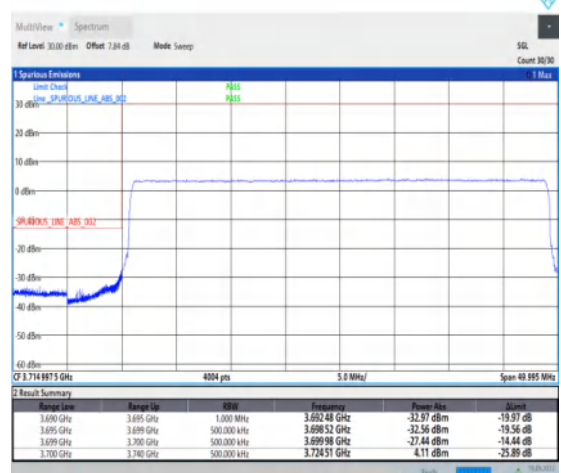
1-N77-3700-3980--30-40-L-6-CP-QPSK-Outer_Full-106@0-Ant1-1--PASS-see graph
