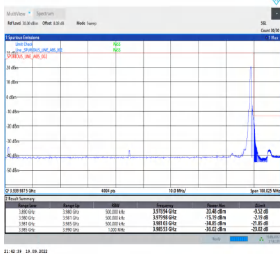
1-N77-3700-3980--30-90-H-5-CP-QPSK-Edge_1RB_R ight-1@244-Ant1-1--PASS-see graph
