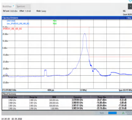
1-N77-3700-3980-PC2-30-20-H-5-CP-QPSK-Edge_1R B_Right-1@50-Ant1-1--PASS-see graph
