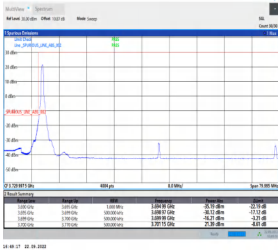
1-N77-3700-3980-PC2-30-70-L-4-CP-QPSK-Edge_1R B_Left-1@0-Ant1-1--PASS-see graph
