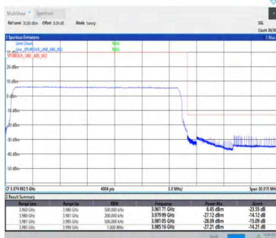
1-N77-3700-3980--30-20-H-6-CP-QPSK-Outer_Ful l-51@0-Ant1-1--PASS-see graph
