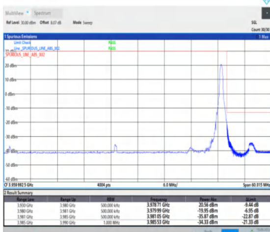
1-N77-3700-3980--30-50-H-5-CP-QPSK-Edge_1RB_R ight-1@132-Ant1-1--PASS-see graph
