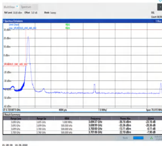
1-N77-3700-3980--30-60-L-4-CP-QPSK-Edge_1RB_Left-1@0-Ant1-1--PASS-see graph
