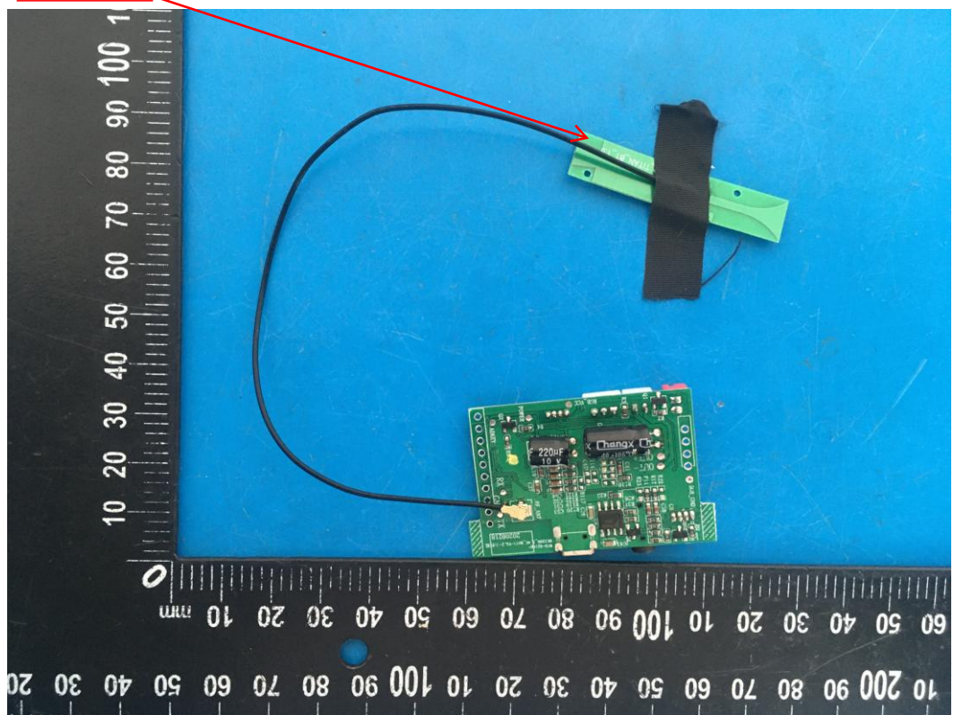
BT antenna
