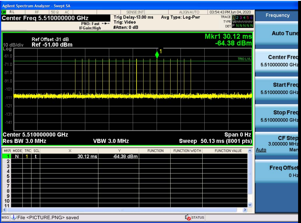
Radar Type 0 Calibration Plot (5510MHz)
