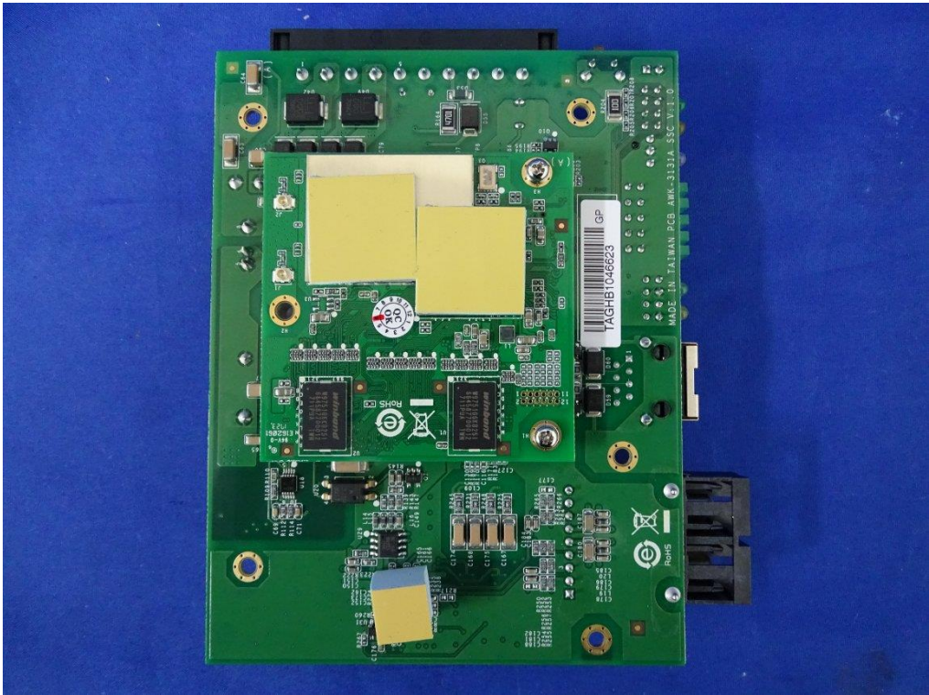
(55) EUT Photo
