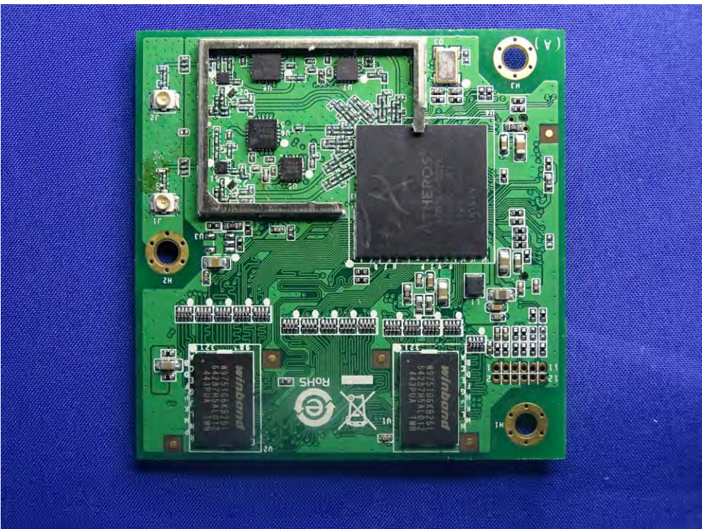
(38) EUT Photo
