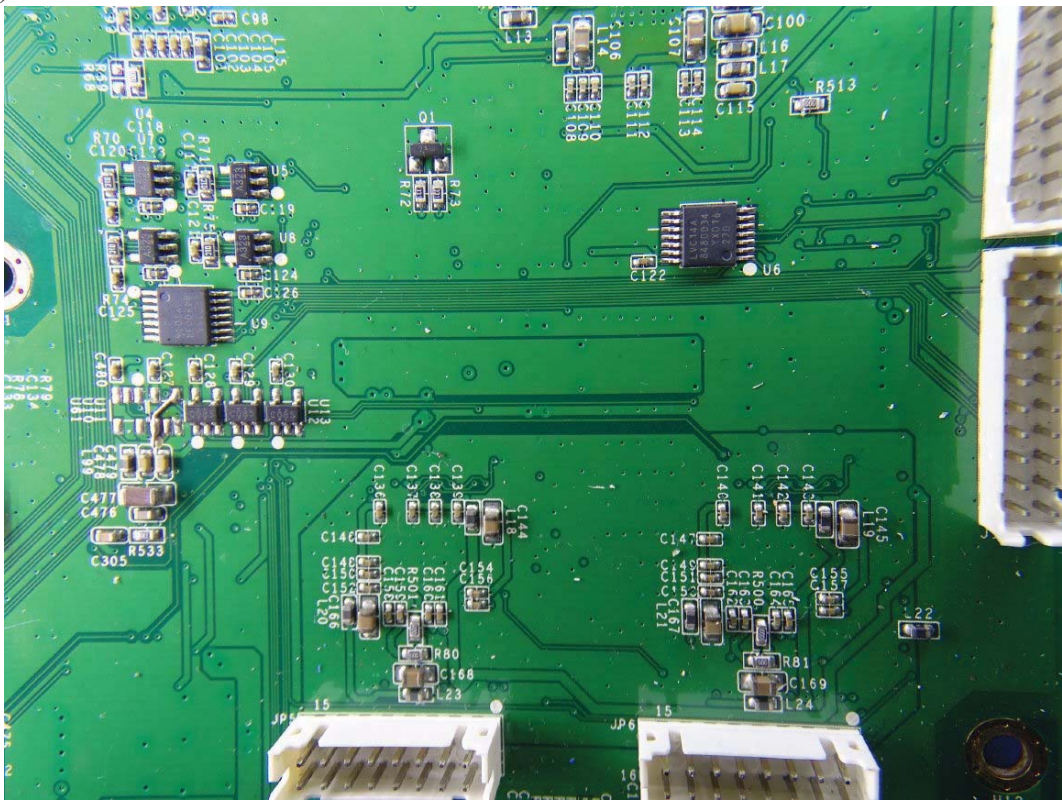
(42) EUT Photo
