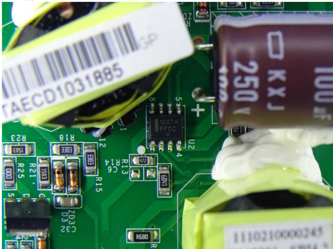
(42) EUT Photo
