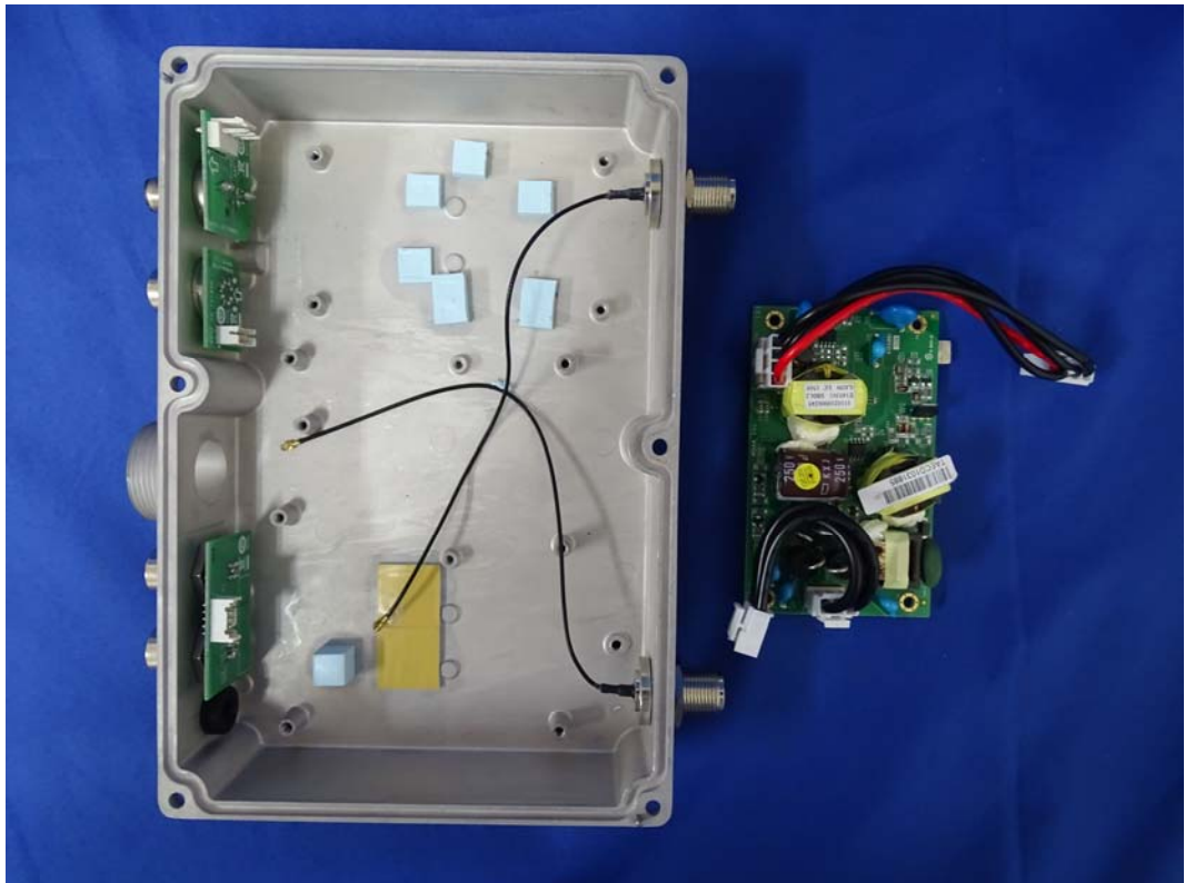
(38) EUT Photo
