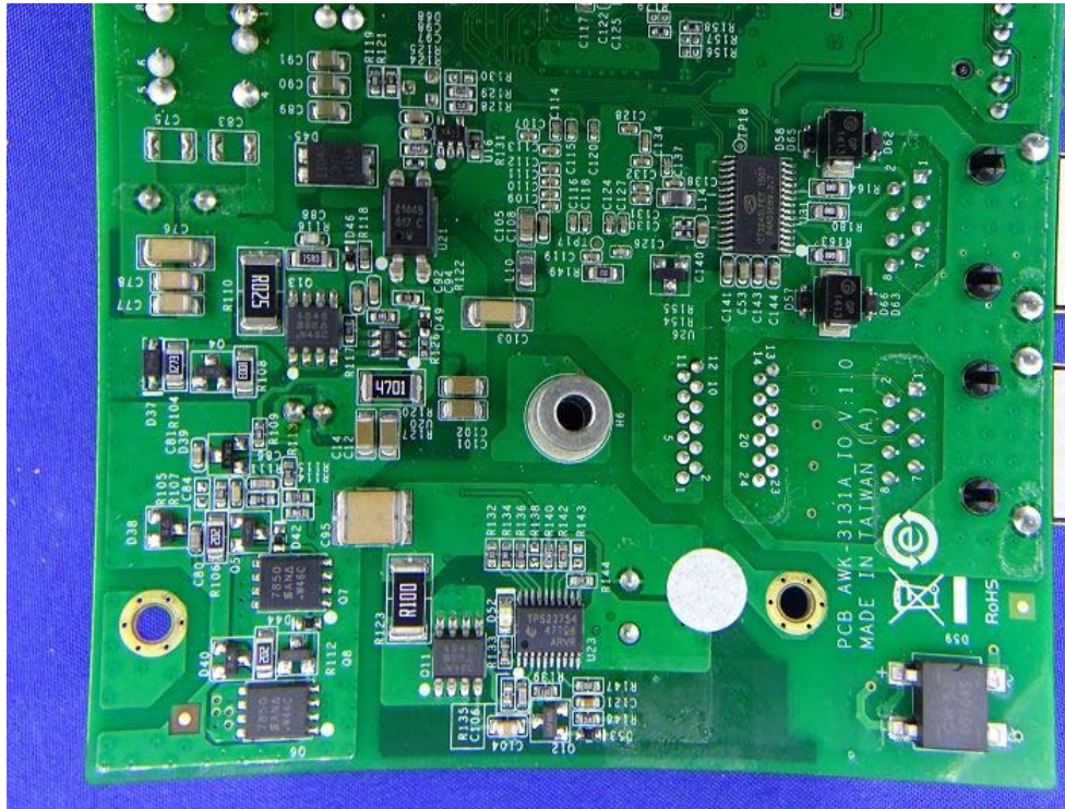
(25) EUT Photo
