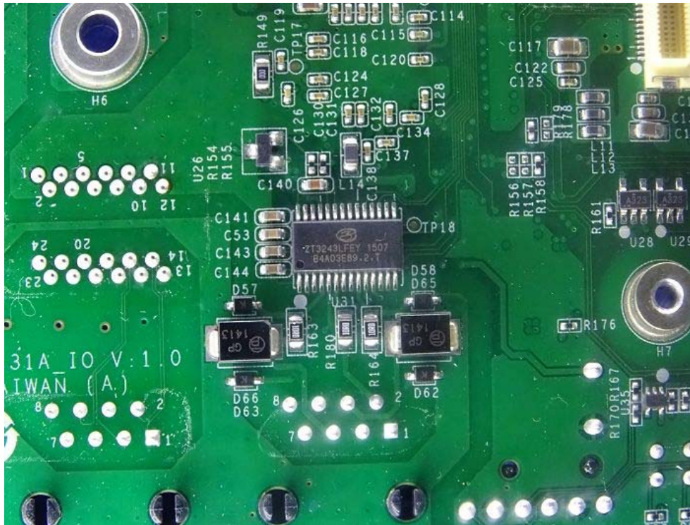
(23) EUT Photo
