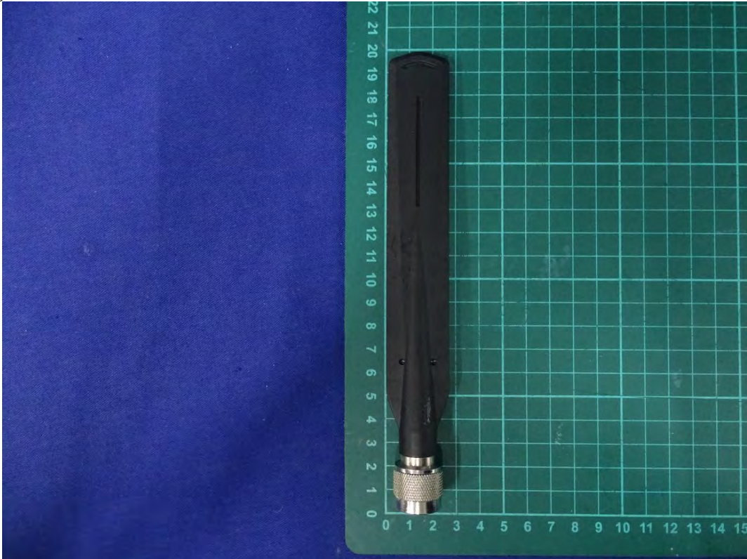
(20) EUT Photo _ Antenna: MOXA / ANT-WDB-ANM-0502
