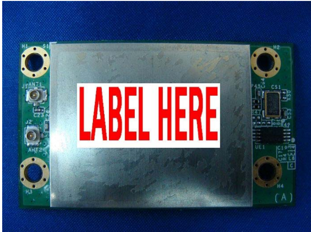
(7) EUT Photo
