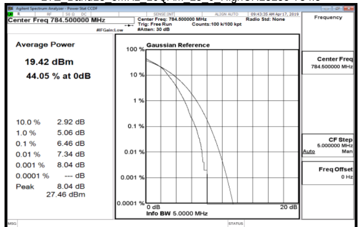
LTE Band13 5MHz 16QAM 25 0 HighCH23255-784.5
