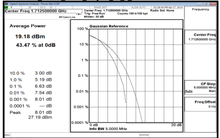
LTE Band4 5MHz 16QAM 25 0 LowCH19975-1712.5
