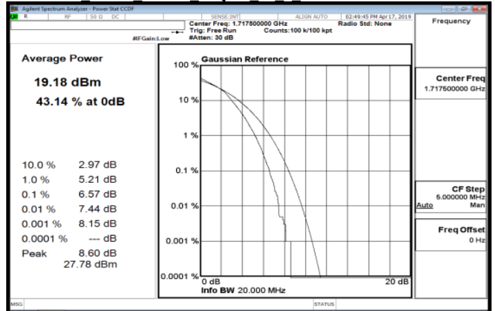
LTE Band4 15MHz 16QAM 75 0 LowCH20025-1717.5
