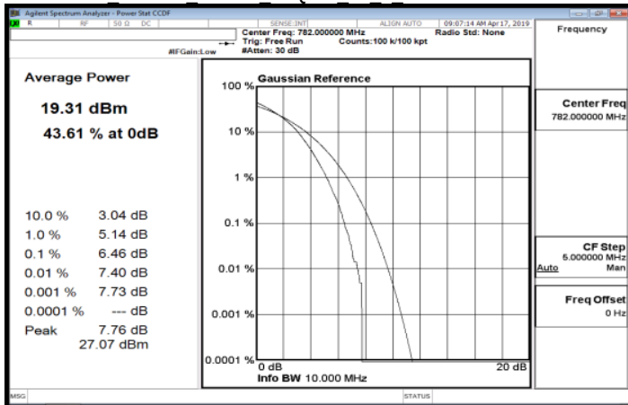
LTE Band13 10MHz 16QAM 50 0 Low CH23230-782
