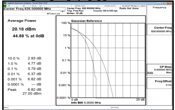
LTE Band5 5MHz 16QAM 25 0 LowCH20425-826.5
