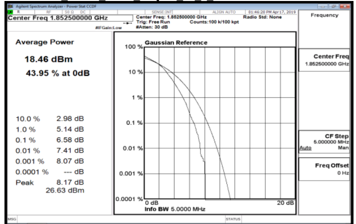
LTE Band2 5MHz 16QAM 25 0 LowCH18625-1852.5
