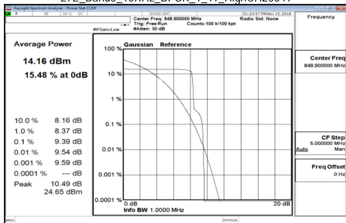
LTE_Band5_15KHz_BPSK_1_11_HighCH20649
