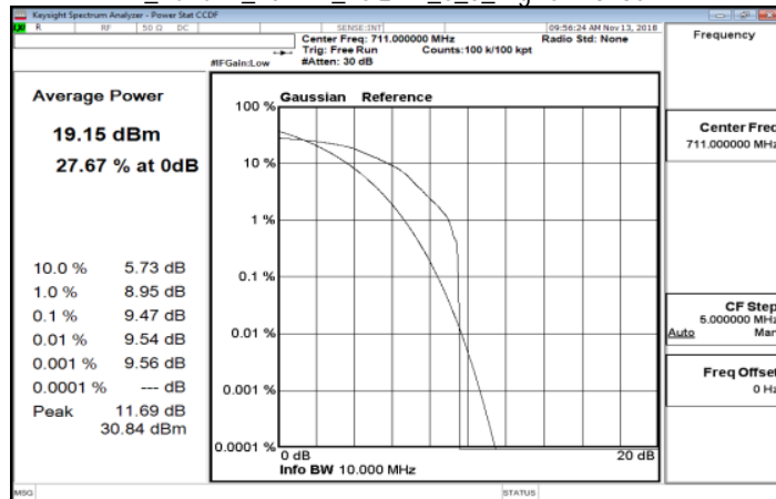
LTE_Band12_10MHz_16QAM_6_0_HighCH23130-711
