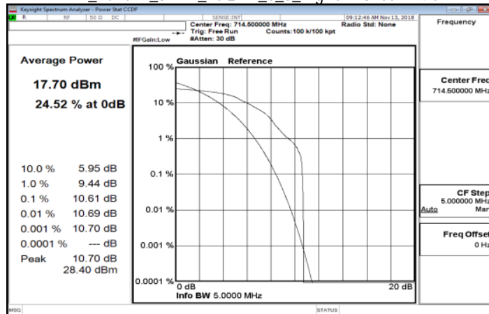
LTE_Band12_3MHz_16QAM_6_0_HighCH23165-714.5
