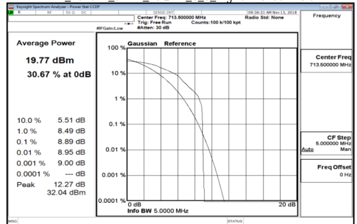
LTE_Band12_5MHz_16QAM_6_0_HighCH23155-713.5
