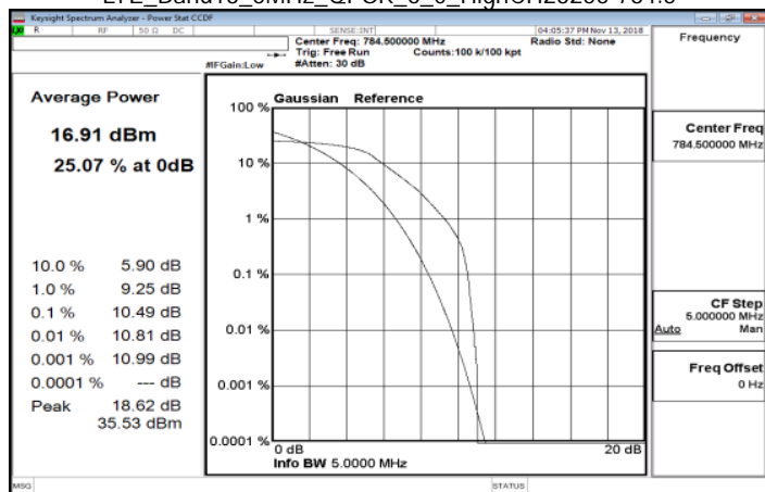
LTE_Band13_5MHz_QPSK_6_0_HighCH23255-784.5
