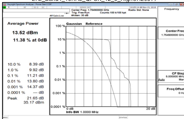
LTE_Band4_15KHz_QPSK_12_0_HighCH20399
