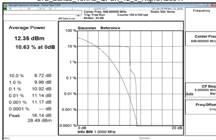
LTE_Band5_15KHz_QPSK_12_0_HighCH20649
