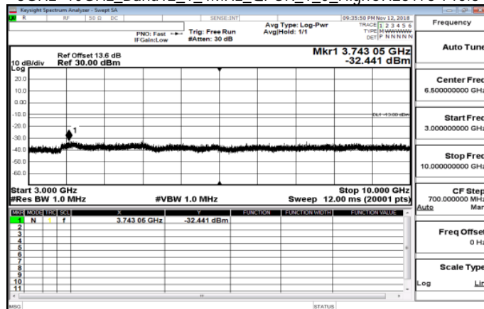
3GHz~10GHz_Band12_1_4MHz_QPSK_1_0_HighCH23173-715.3
