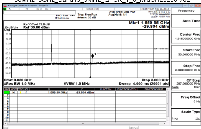
30MHz~3GHz_Band13_5MHz_QPSK_1_0_MidCH23230-782
