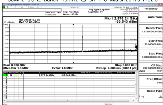
30MHz~3GHz_Band4_15MHz_QPSK_1_0_MidCH20175-1732.5
