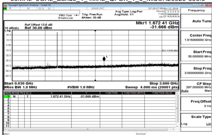
30MHz~3GHz_Band5_1_4MHz_QPSK_1_0_MidCH20525-836.5
