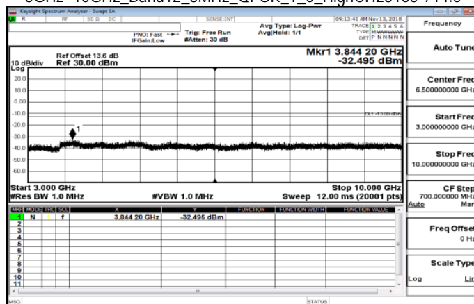
3GHz~10GHz_Band12_3MHz_QPSK_1_0_HighCH23165-714.5
