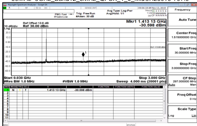
30MHz~3GHz_Band12_3MHz_QPSK_1_0_MidCH23095-707.5
