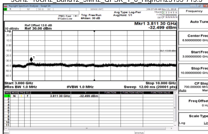
3GHz~10GHz_Band12_5MHz_QPSK_1_0_HighCH23155-713.5
