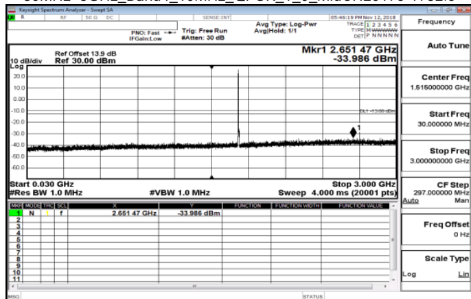
30MHz~3GHz_Band4_10MHz_QPSK_1_0_MidCH20175-1732.5
