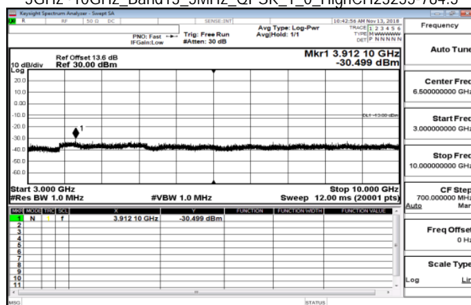
3GHz~10GHz_Band13_5MHz_QPSK_1_0_HighCH23255-784.5
