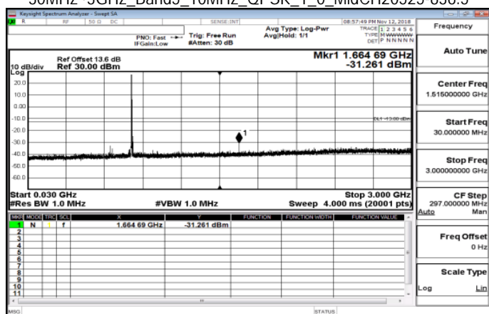
30MHz~3GHz_Band5_10MHz_QPSK_1_0_MidCH20525-836.5
