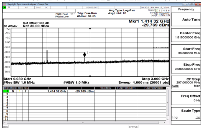
30MHz~3GHz_Band12_1_4MHz_QPSK_1_0_MidCH23095-707.5
