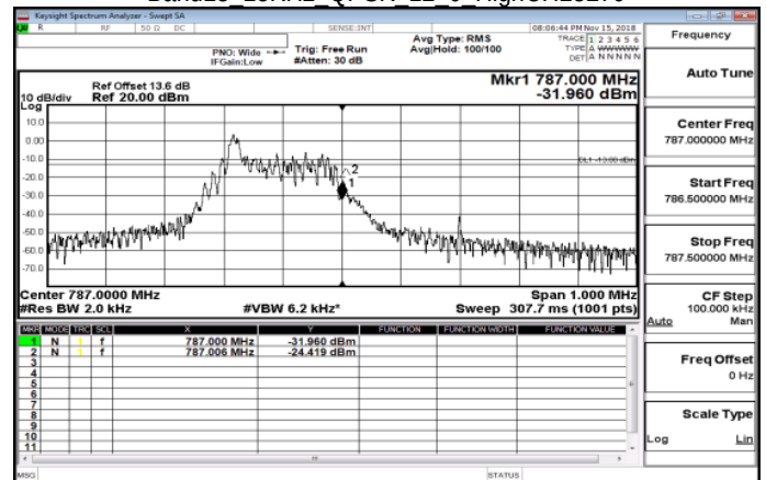
Band13 15KHz QPSK 12 0 HighCH23279
