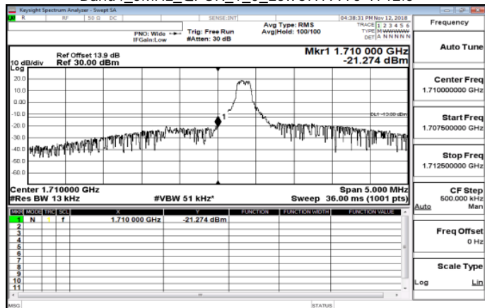
Band4_5MHz_QPSK_1_0_LowCH19975-1712.5
