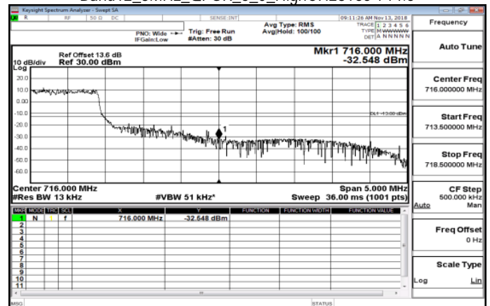
Band12_3MHz_QPSK_6_0_HighCH23165-714.5
