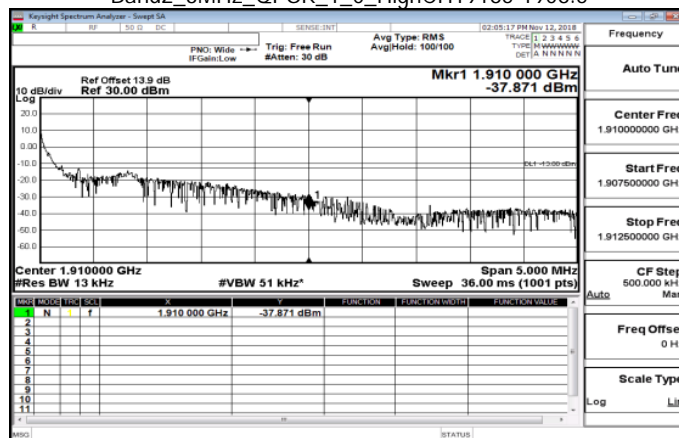
Band2_3MHz_QPSK_1_0_HighCH19185-1908.5
