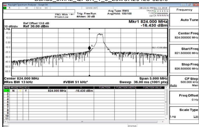
Band5_5MHz_QPSK_1_0_LowCH20425-826.5
