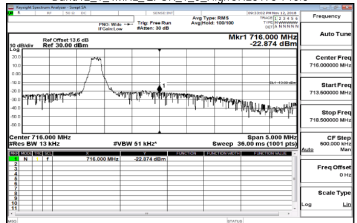
Band12_1_4MHz_QPSK_1_0_HighCH23173-715.3
