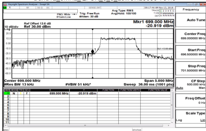
Band12_5MHz_QPSK_6_0_LowCH23035-701.5
