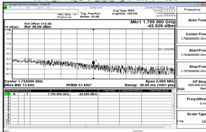
Band4_5MHz_QPSK_6_0_HighCH20375-1752.5
