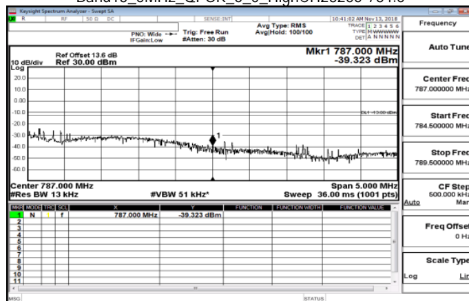
Band13_5MHz_QPSK_6_0_HighCH23255-784.5
