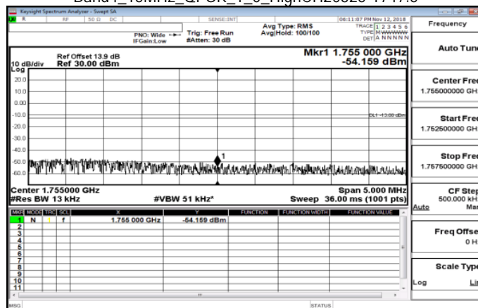
Band4_15MHz_QPSK_1_0_HighCH20325-1747.5
