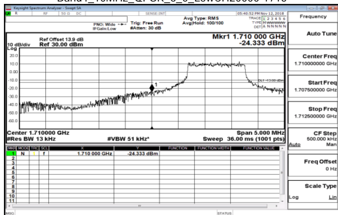
Band4_10MHz_QPSK_6_0_LowCH20000-1715
