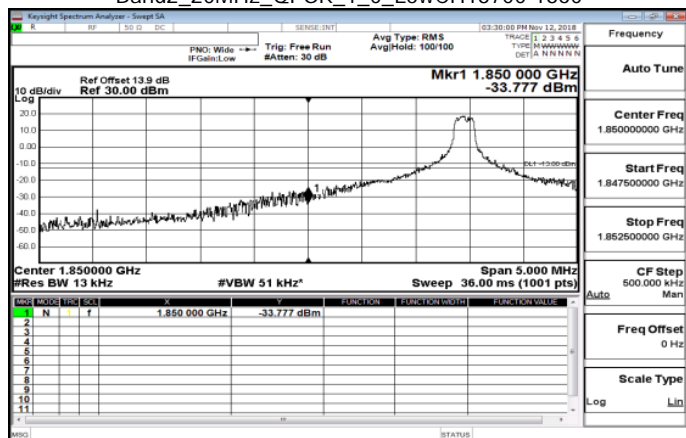
Band2_20MHz_QPSK_1_0_LowCH18700-1860
