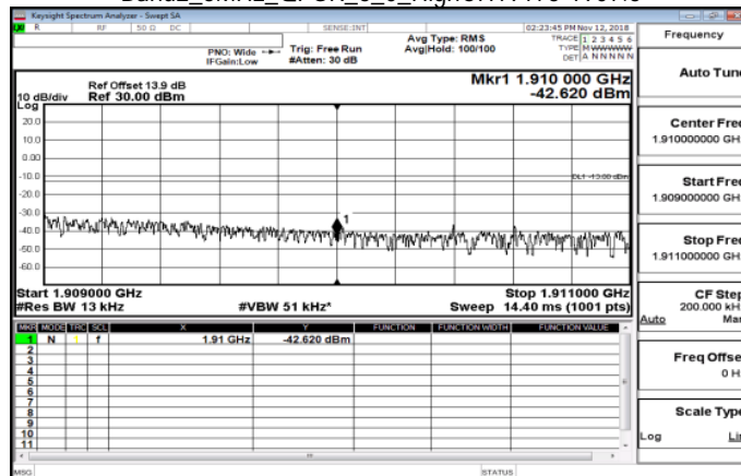
Band2_5MHz_QPSK_6_0_HighCH19175-1907.5
