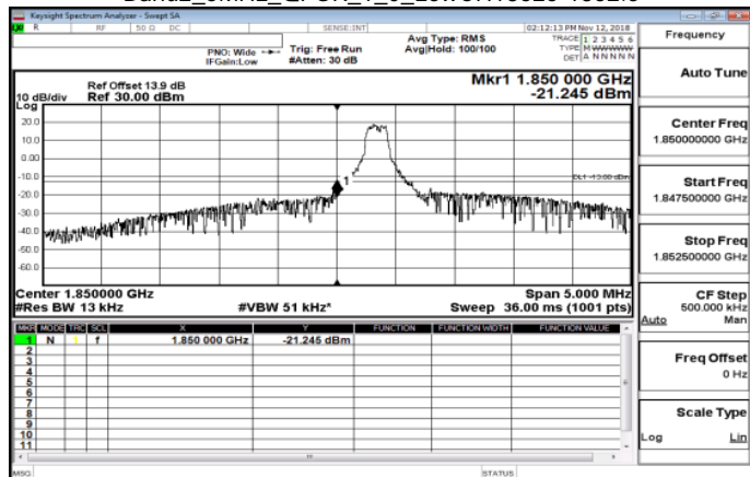
Band2_5MHz_QPSK_1_0_LowCH18625-1852.5
