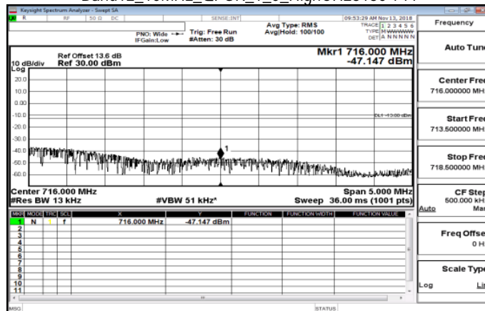
Band12_10MHz_QPSK_1_0_HighCH23130-711
