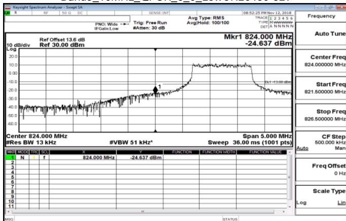
Band5_10MHz_QPSK_6_0_LowCH20450-829
