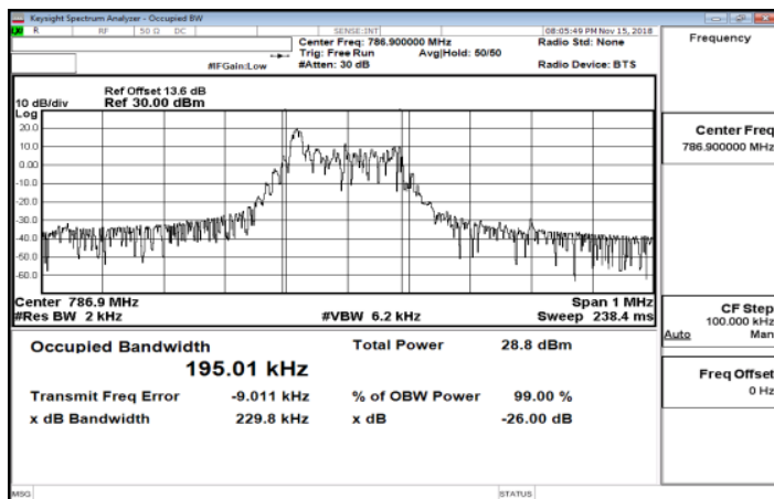
Band13_15KHz_QPSK_12_0_HighCH23279
