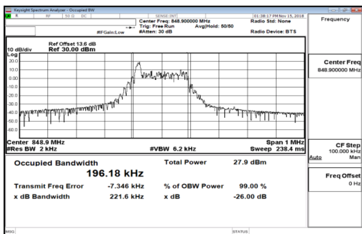
Band5_15KHz_QPSK_12_0_HighCH20649
