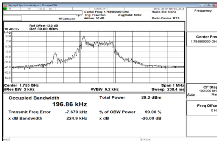
Band4_15KHz_QPSK_12_0_HighCH20399
