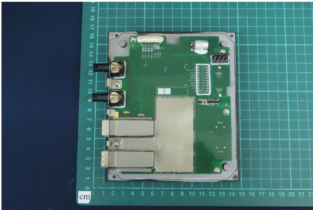
(32) EUT Photo
