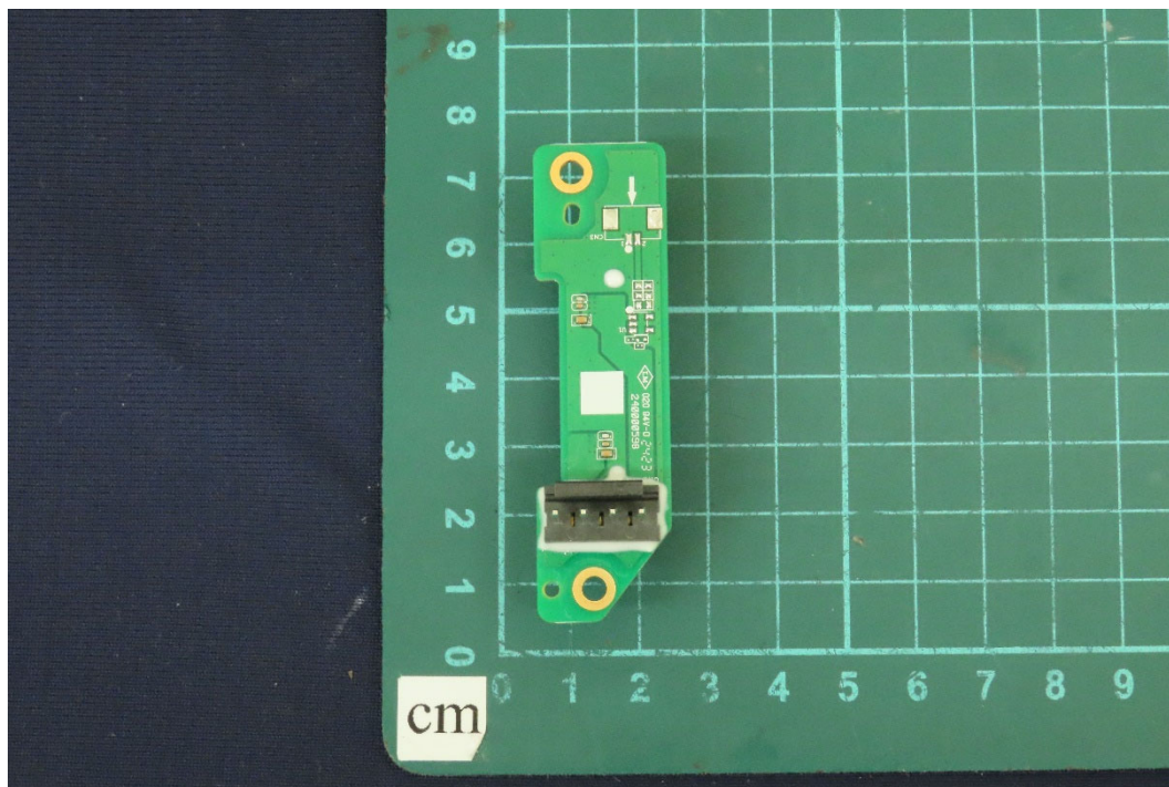
(42) EUT Photo
