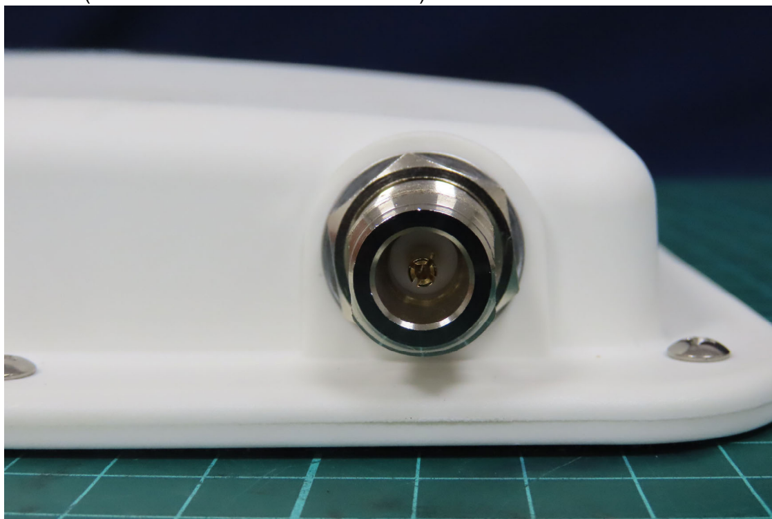
(17) EUT Photo (Antenna: MOXA / ANT-WDB-PNF-1011)
