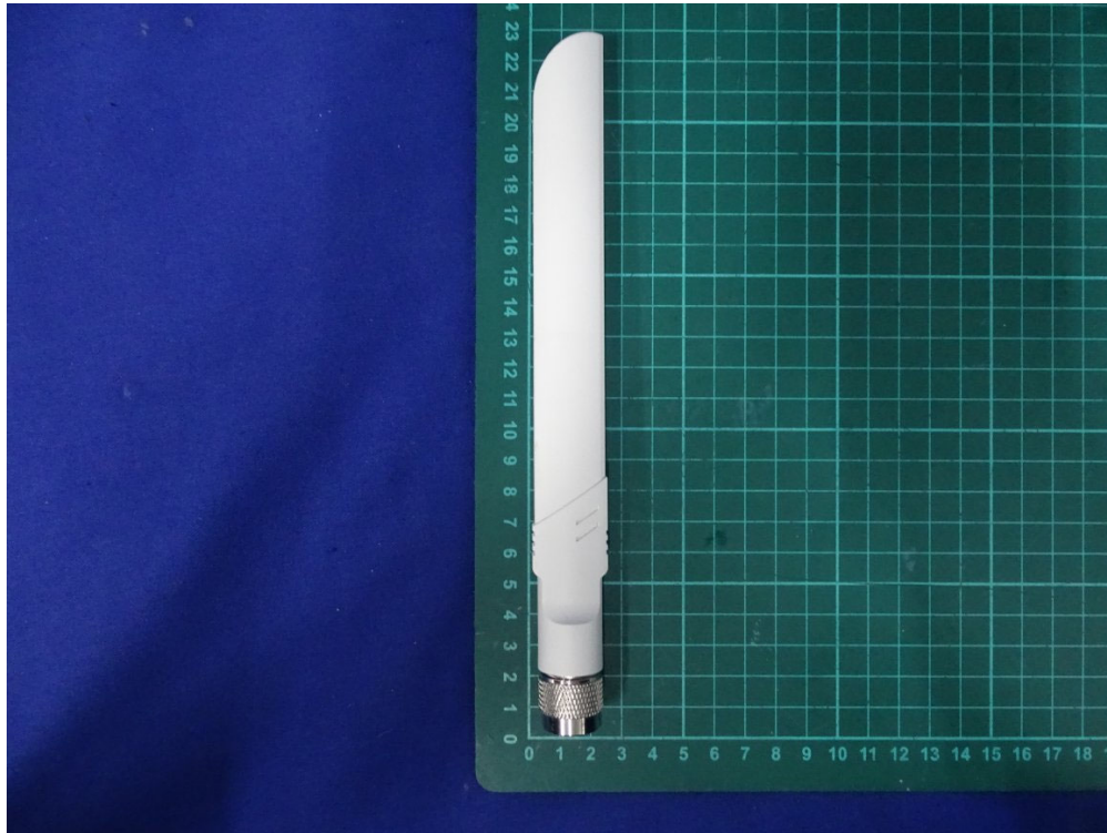
(7) EUT Photo_ Antenna: MOXA / ANT-WDB-ANM-0306
