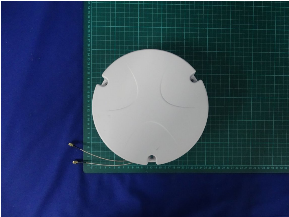
(22) EUT Photo_ Antenna: MOXA / MAT-WDB-CA-RM-2-0205
