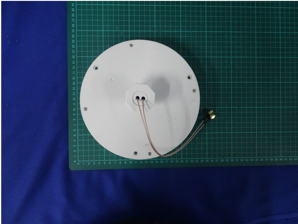
(23) EUT Photo_ Antenna: MOXA / MAT-WDB-CA-RM-2-0205
