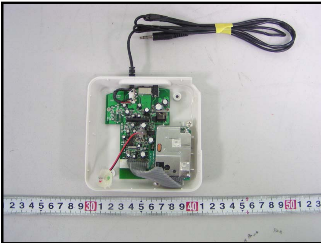
EUT –Board Top View
