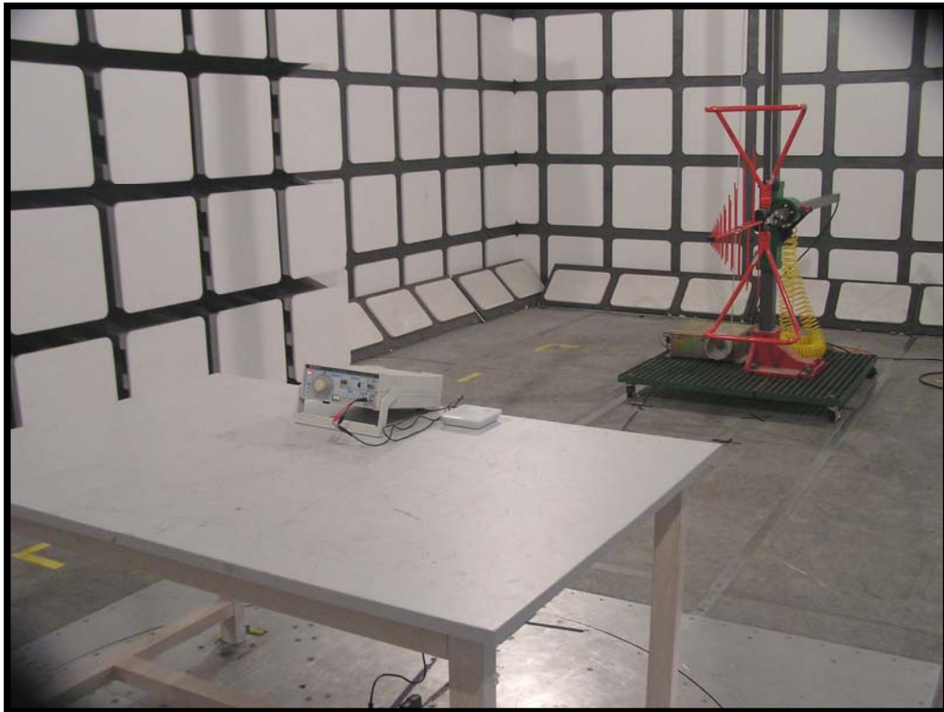
Radiated Emissions - Front View, 30MHz-1000MHz
