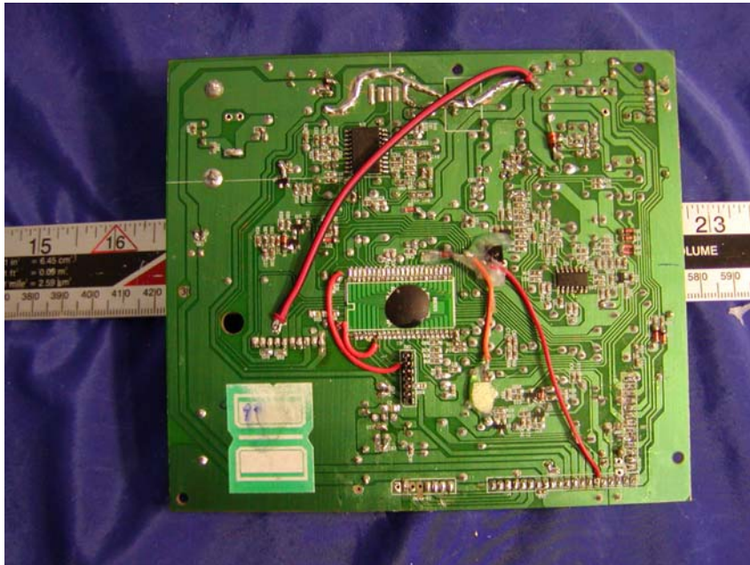
Base Board 2 – Solder View
