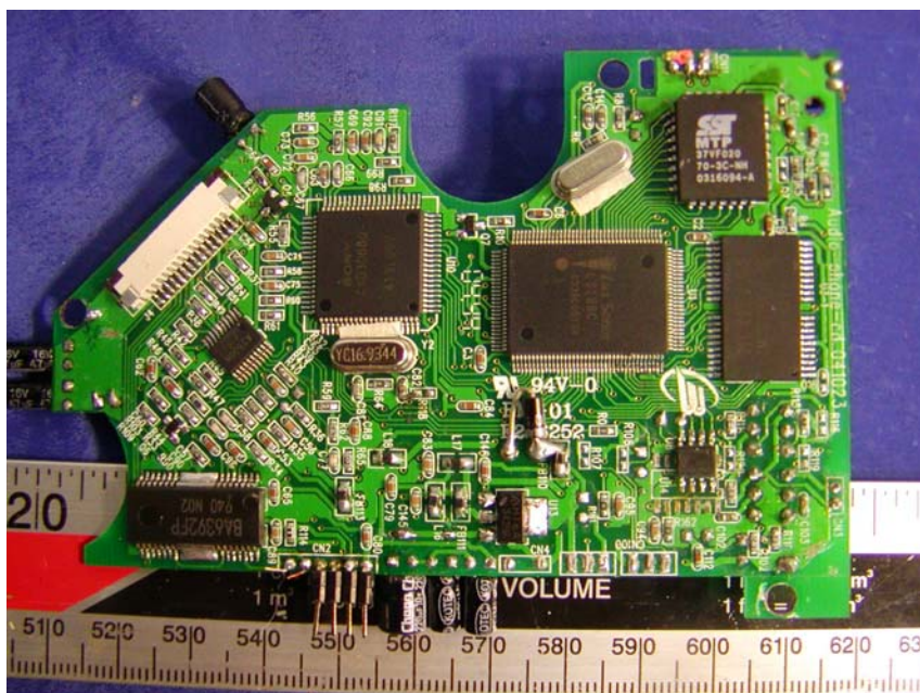
CD Player Board – Solder View
