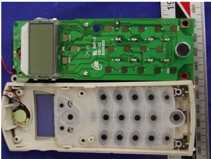
Handset – Component View
