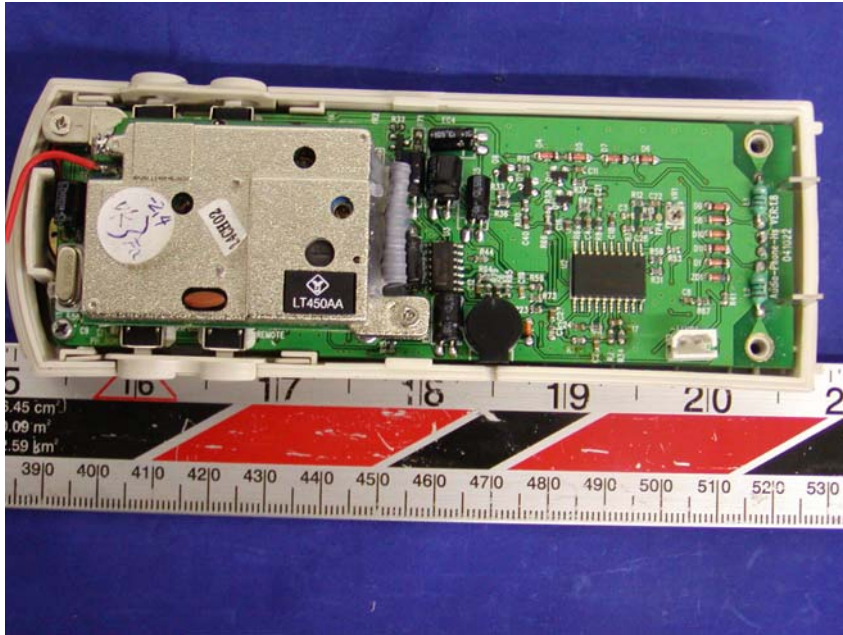
Handset – Chassis Cover Off View
