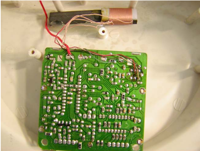
Base Board 1 – Solder View
