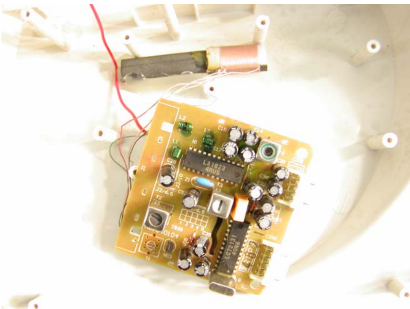
Base Board 1 – Component View
