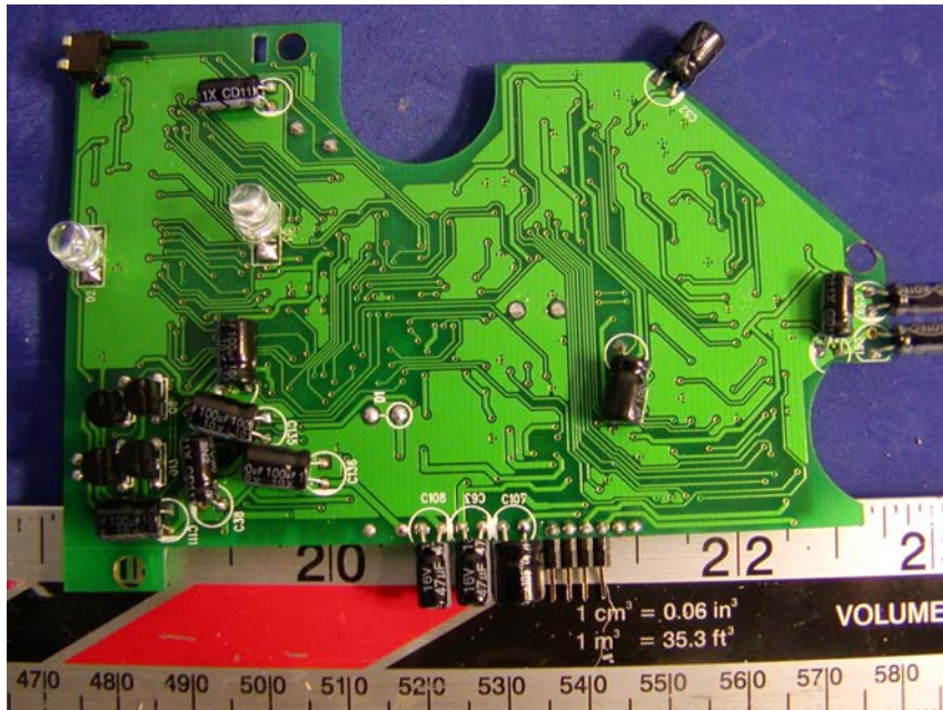
CD Player Board – Component View
