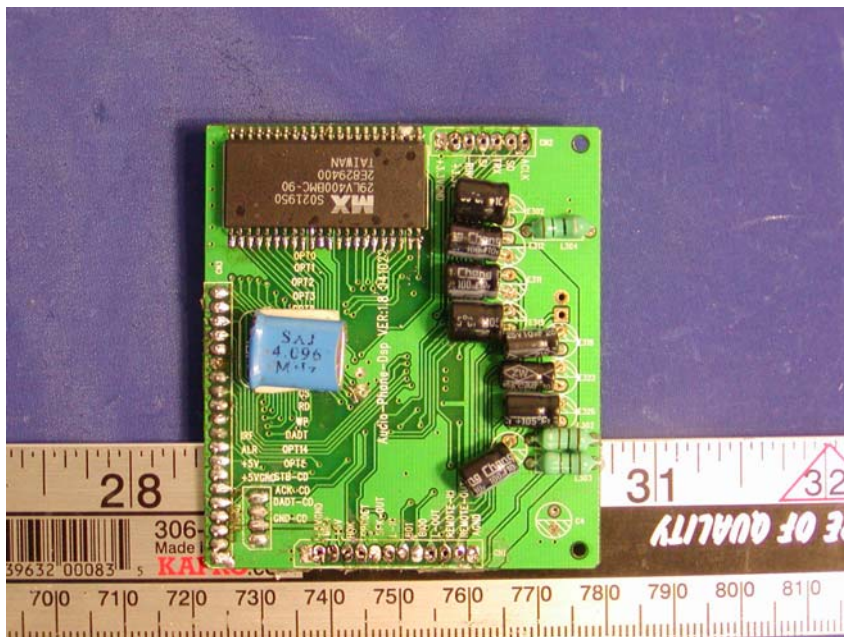
Base Board 3 – Solder View
