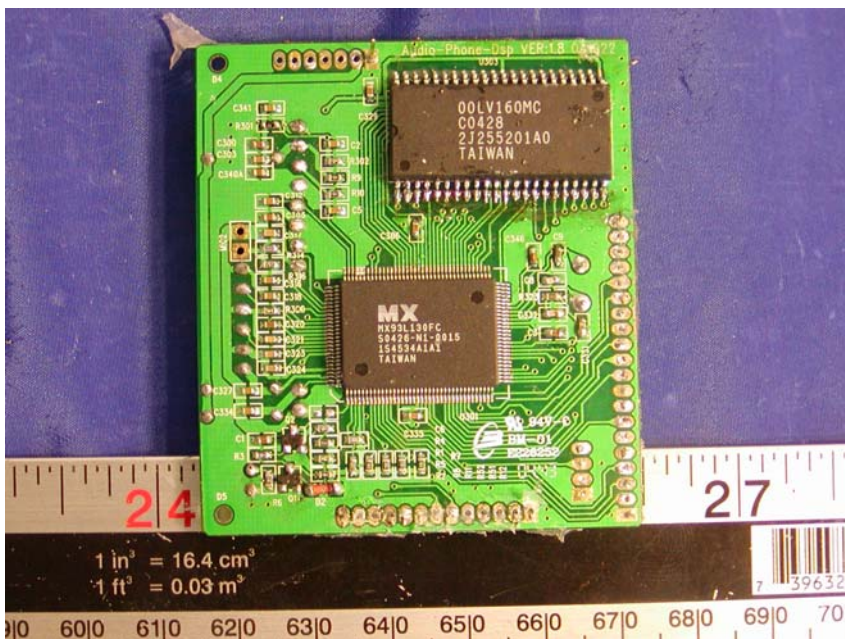
Base Board 3 – Component View
