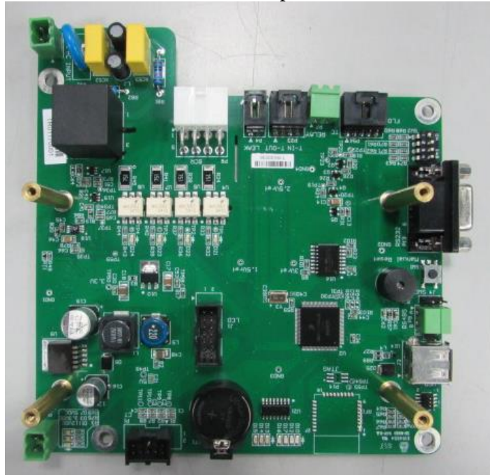
PCB view of main power board
