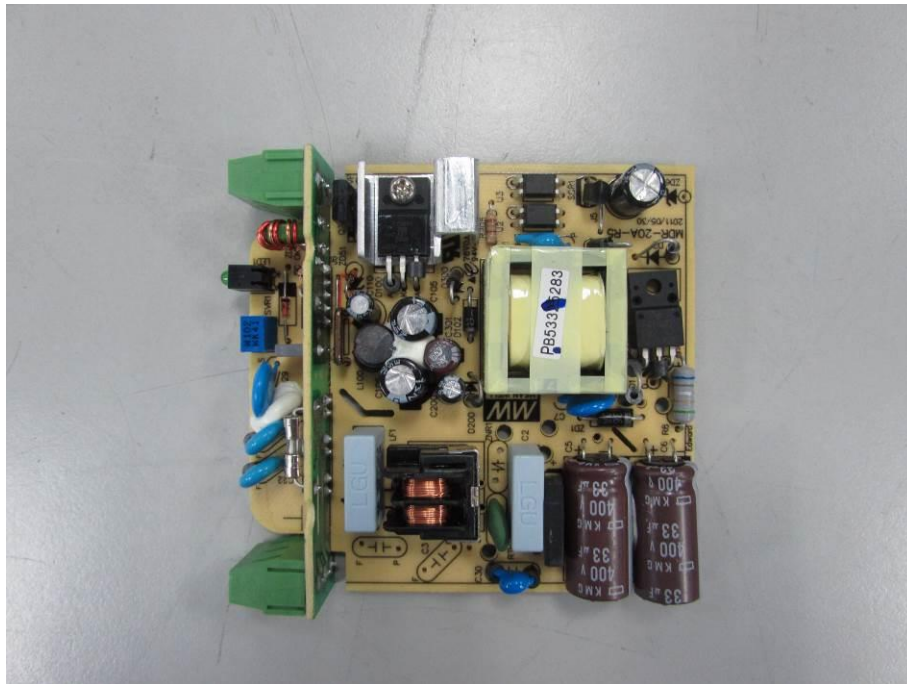
PCB view of adaptor
