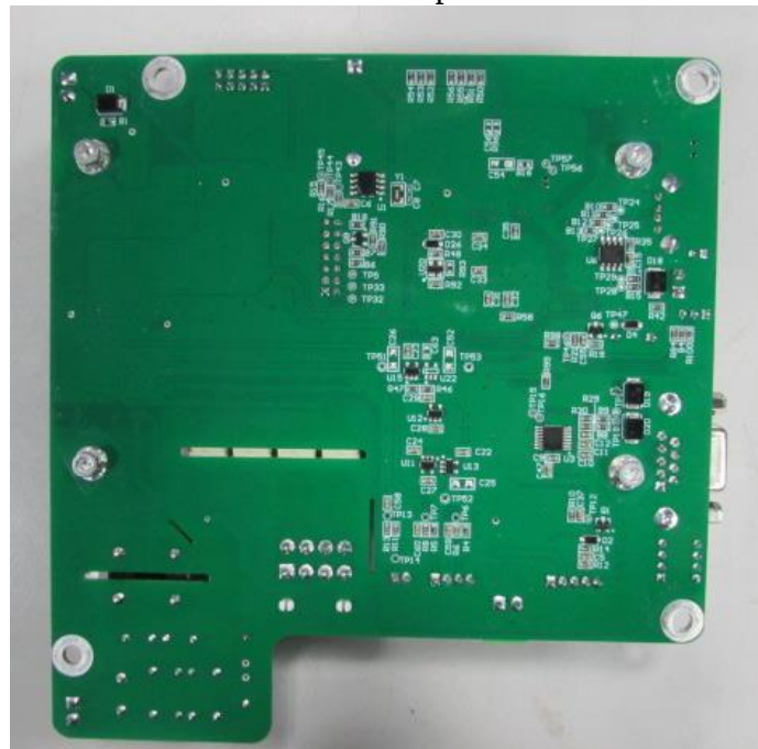
PCB view of main power board
