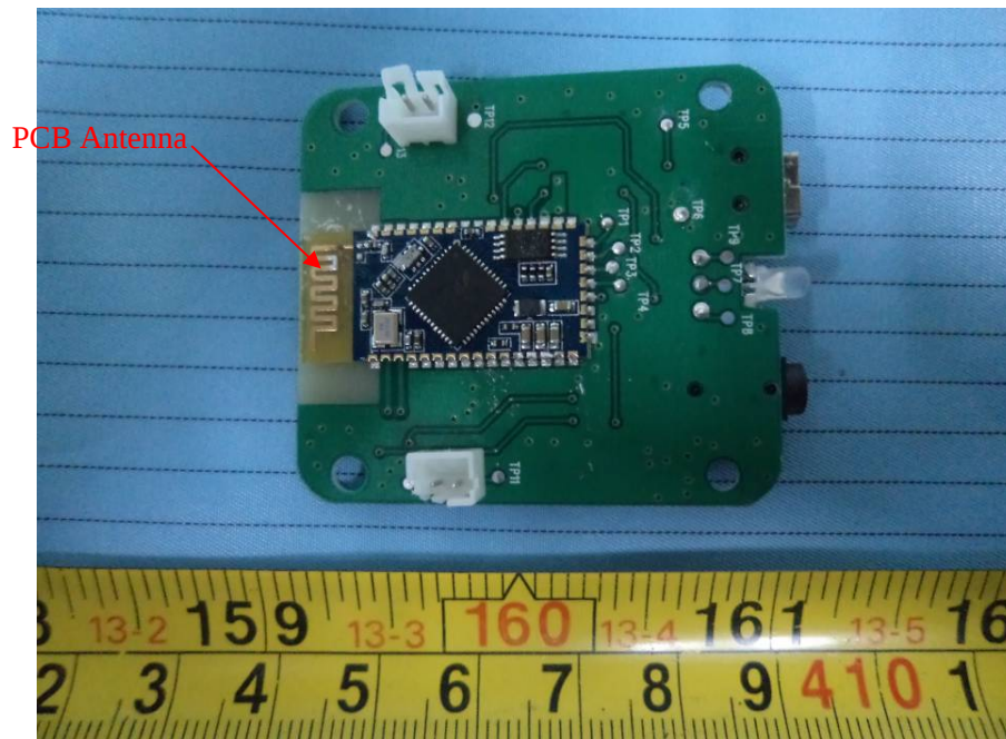
EUT – Main Board Bottom View (with RF Board)
