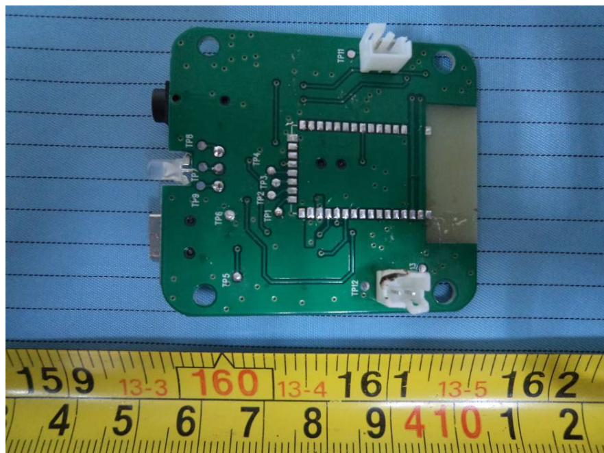
EUT – Main Board Bottom View (without RF Board)
