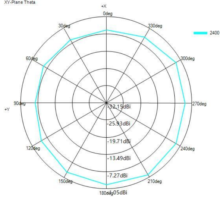
XY-Plane Theta
