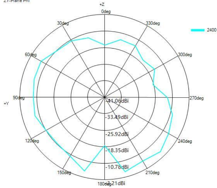
ZY-Plane Phi
