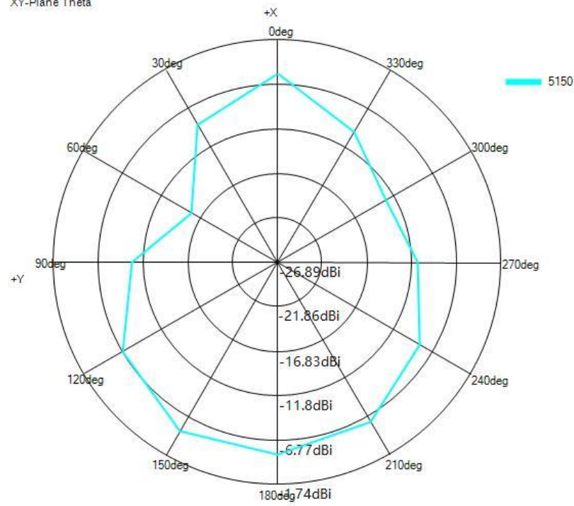
XY-Plane Theta
