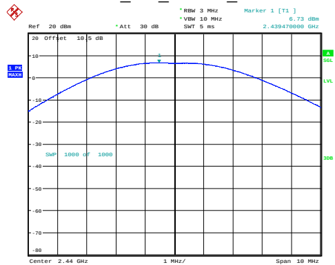
BLE_2M_Middle_Channel
