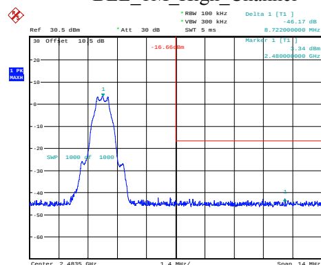
BLE_1M_High_Channel
