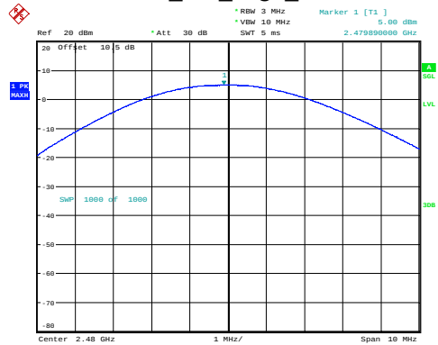
BLE_1M_High_Channel
