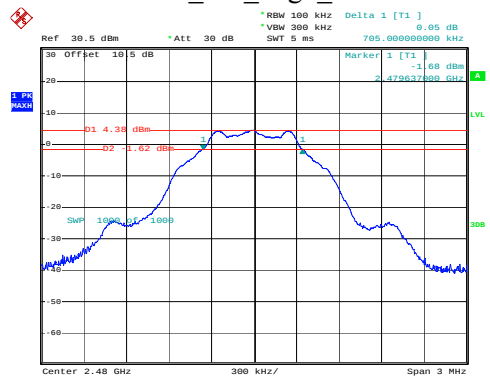
BLE_1M_High_Channel
