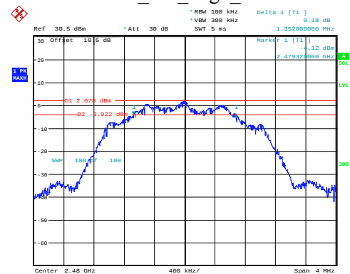
BLE_2M_High_Channel
