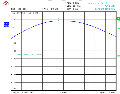
BLE_2M_Low_Channel
