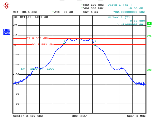
BLE_1M_Low_Channel
