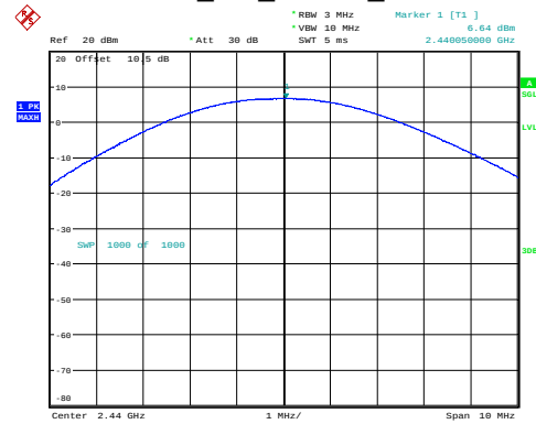
BLE_1M_Middle_Channel
