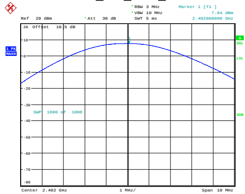
BLE_1M_Low_Channel
