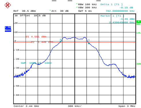
BLE_1M_Middle_Channel
