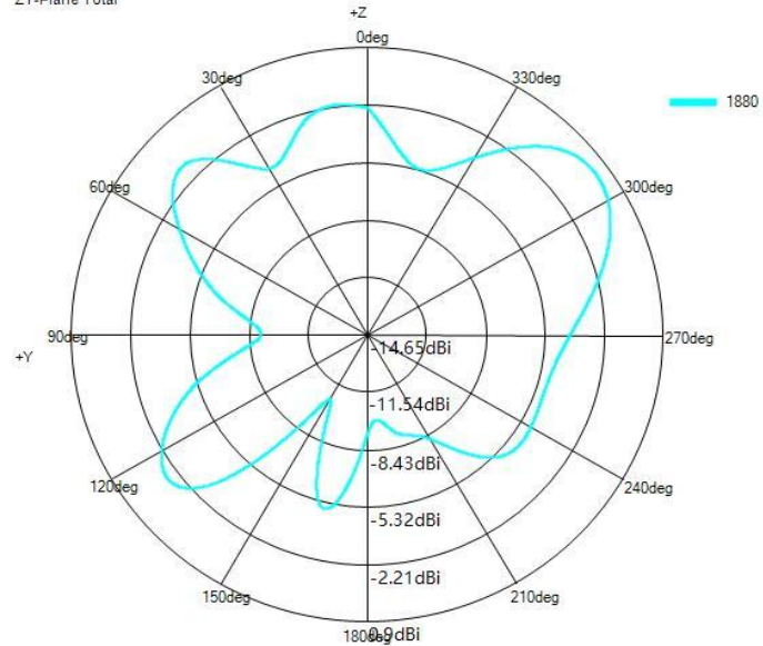
ZY-Plane Total
