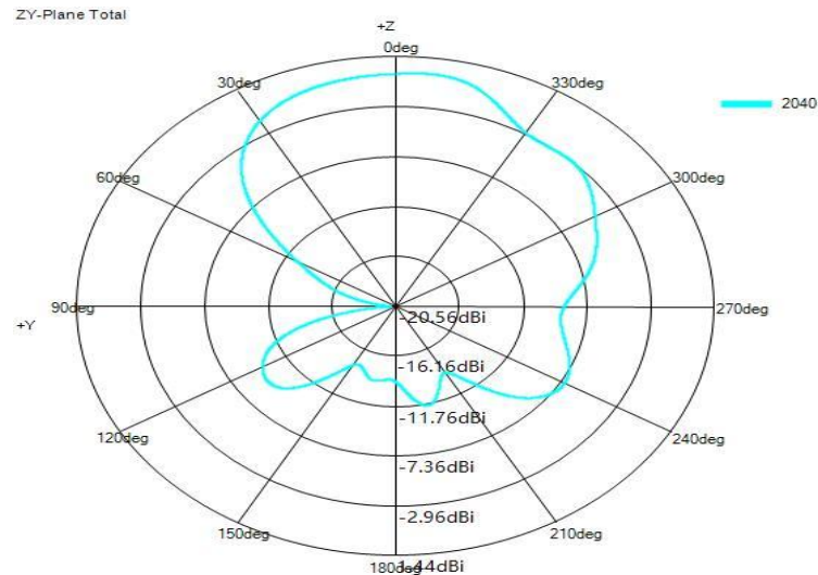
ZY-Plane Total
