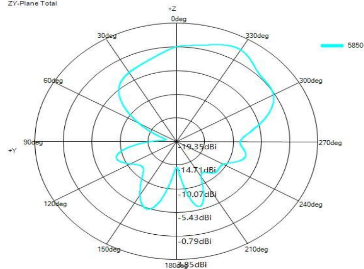
ZY-Plane Total
