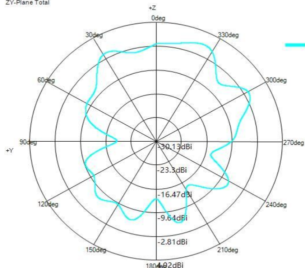
ZY-Plane Total
