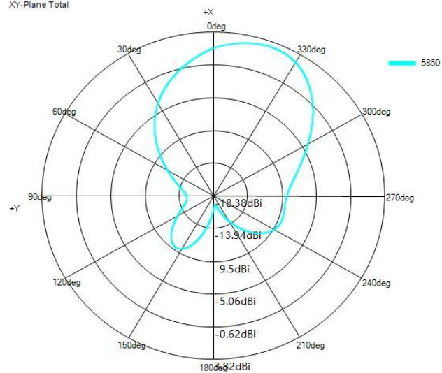
XY-Plane Total
