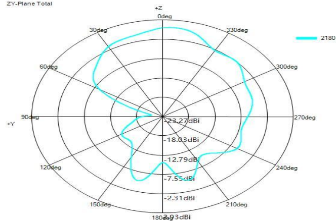
ZY-Plane Total
