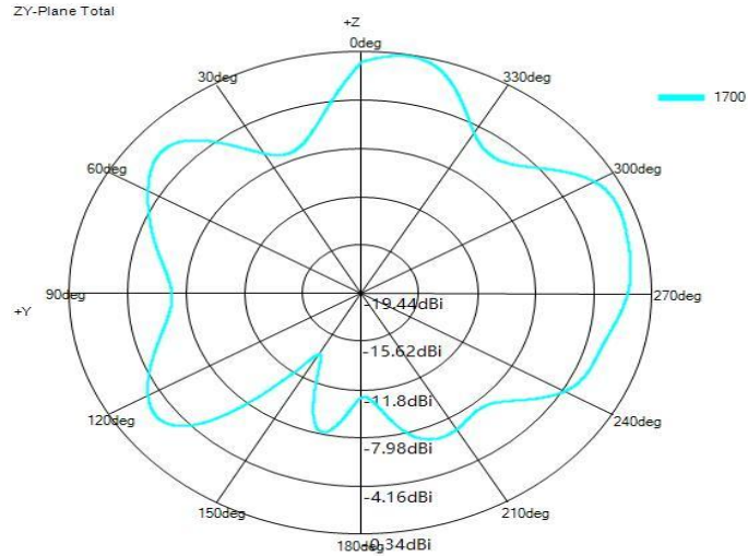
ZY-Plane Total
