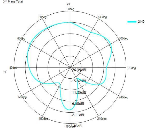
XY-Plane Total
