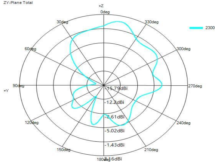
ZY-Plane Total
