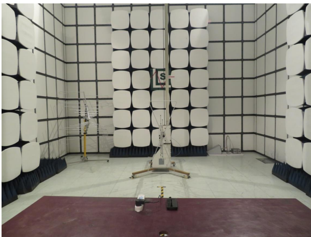
Radiated emission below 1GHz-charging from adapter
