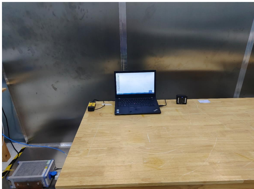
Photograph 4: Set-up photo for Part 15.207, conducted Emission
