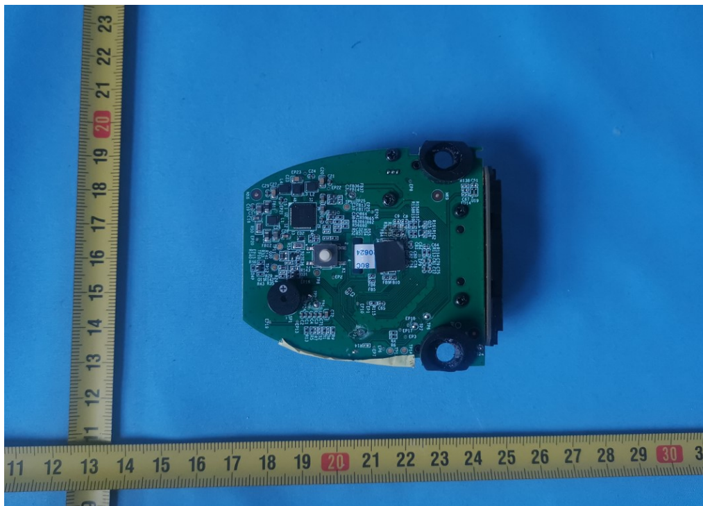
Figure 10 PCB view
