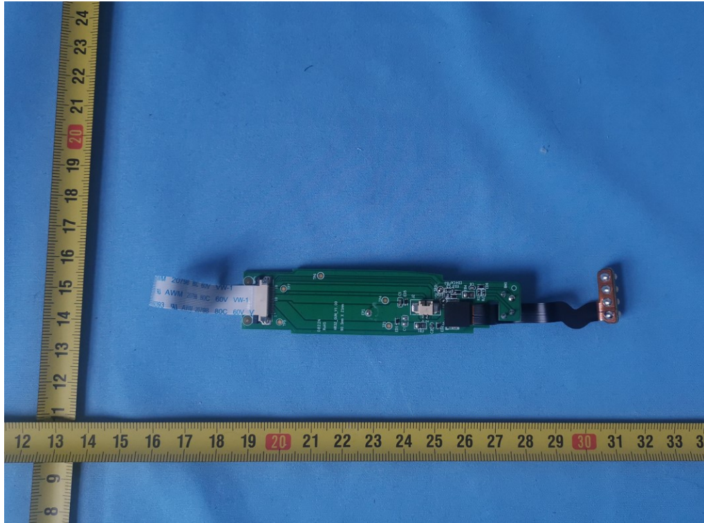
Figure 11 PCB view
