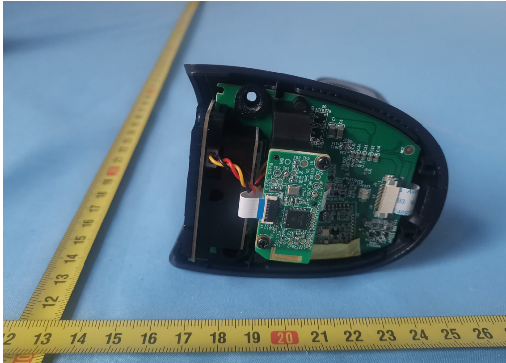
Figure 7 Internal view
