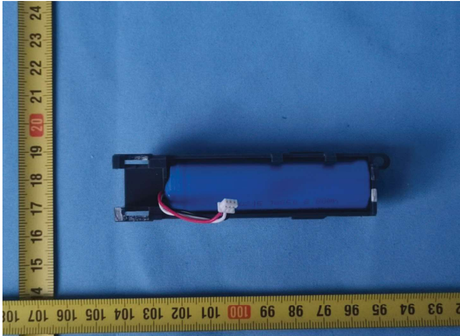
Figure 5. Internal view
