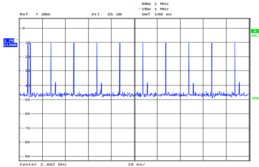
Plot 1: Transmit bursts (within 100ms): 11
