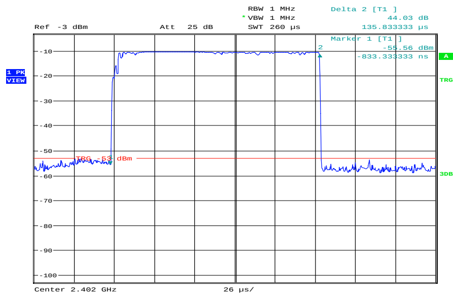
Plot 2: Transmit burst in detail: Burst length 135.83 \mu s
