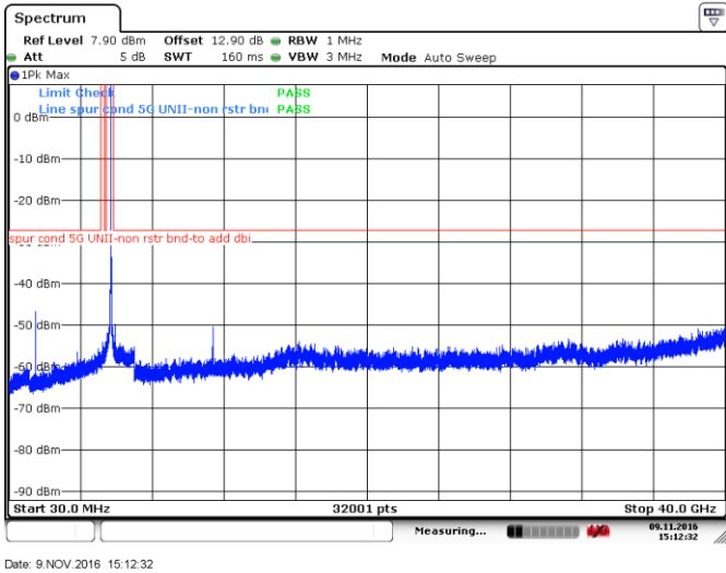
Figure 8.4-29: Peak spurious emissions outside restricted bands at high channel, 802.11ac-VHT20, ch140
