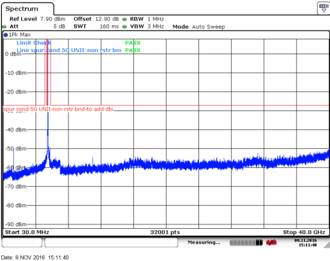
Figure 8.4-27: Peak spurious emissions outside restricted bands at low channel, 802.11ac-VHT20, ch100
