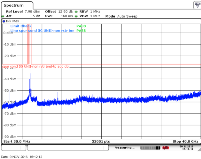
Figure 8.4-28: Peak spurious emissions outside restricted bands at mid channel, 802.11ac-VHT20, ch120
