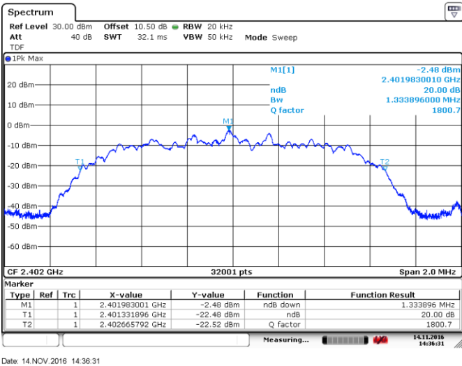
Figure 8.2-5: 20 dB bandwidth on low channel- Modulation 2
