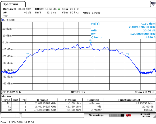
Figure 8.2-9: 20 dB bandwidth on low channel- Modulation 3
