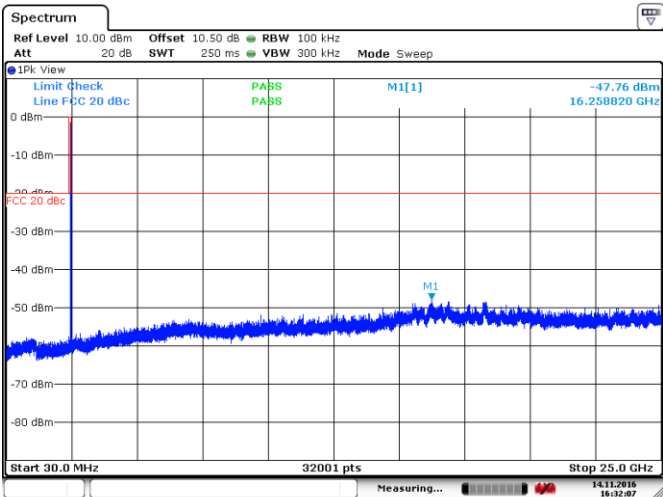
Figure 8.4-3: Conducted spurious emissions for high channel, Modulation 1
