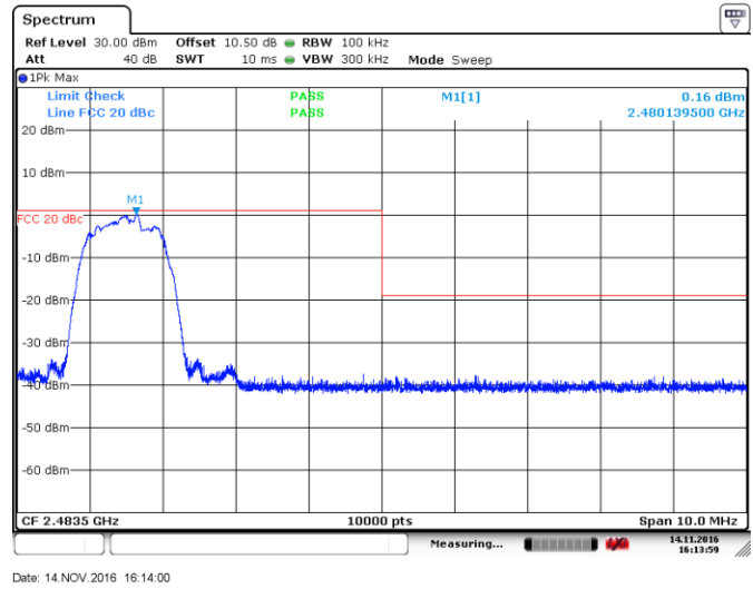
Figure 8.4-19: Conducted spurious emissions at the upper band edge, Modulation 3
