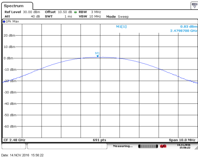
Figure 8.3-3: Output power on high channel, Modulation 1
