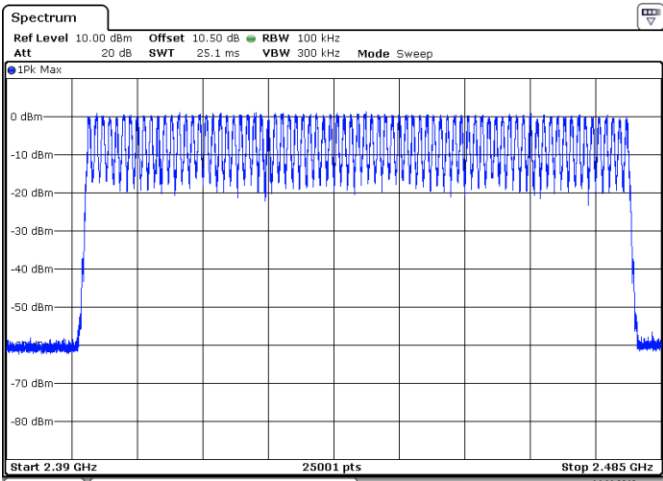
Figure 8.2-13: Number of hopping channels
