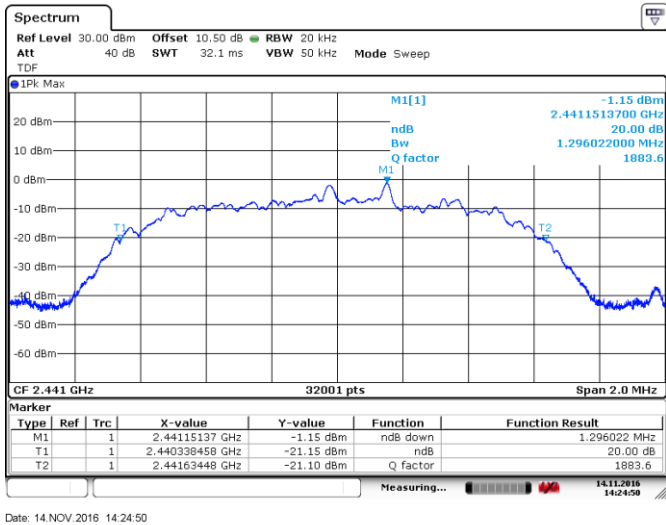
Figure 8.2-10: 20 dB bandwidth on mid channel Modulation 3
