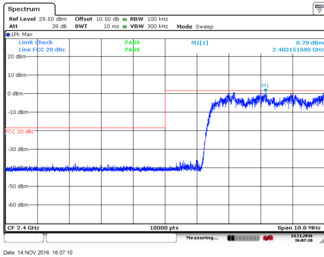
Figure 8.4-20: Conducted spurious emissions at the lower band edge hopping, Modulation 3
