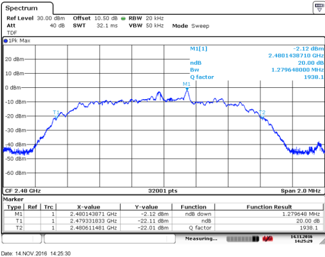
Figure 8.2-11: 20 dB bandwidth on high channel Modulation 3
