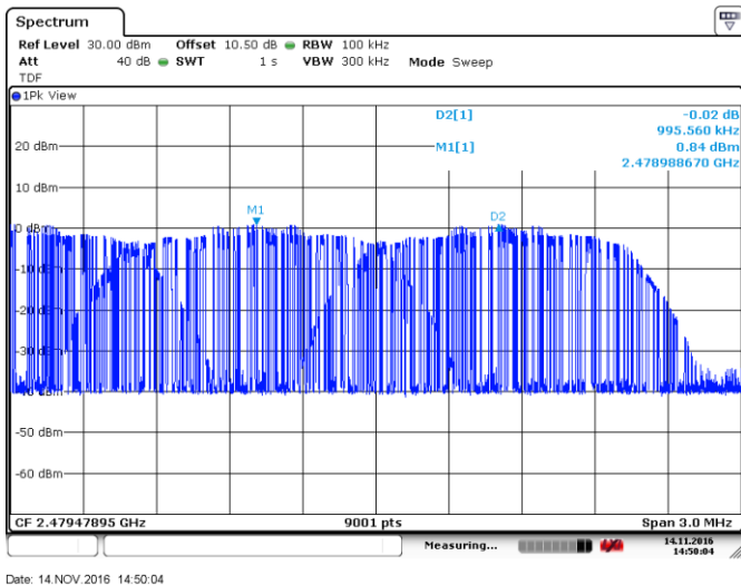
Figure 8.2-8: Carrier frequency separation Modulation 2
