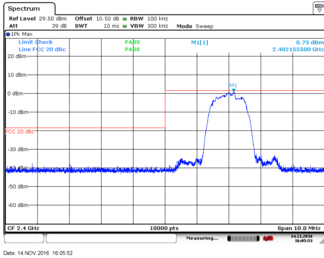
Figure 8.4-18: Conducted spurious emissions at the lower band edge, Modulation 3
