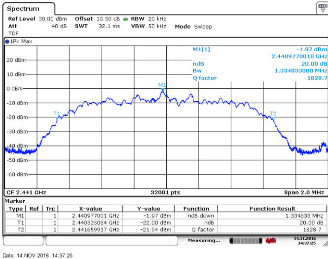
Figure 8.2-6: 20 dB bandwidth on mid channel Modulation 2
