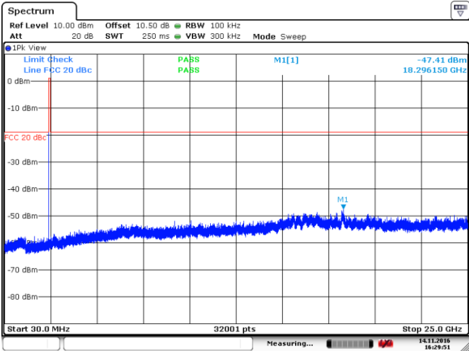
Figure 8.4-1: Conducted spurious emissions for low channel, Modulation 1
