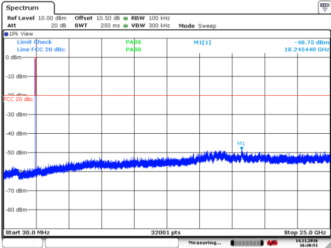
Figure 8.4-2: Conducted spurious emissions for mid channel, Modulation 1
