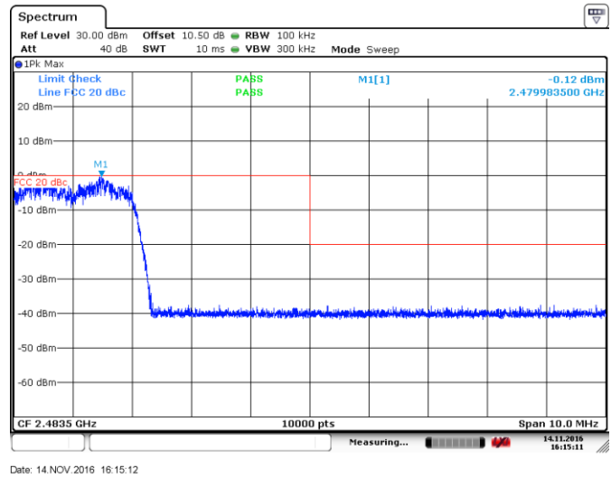
Figure 8.4-21: Conducted spurious emissions for high channel hopping, Modulation 3
