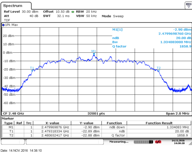
Figure 8.2-7: 20 dB bandwidth on high channel Modulation 2
