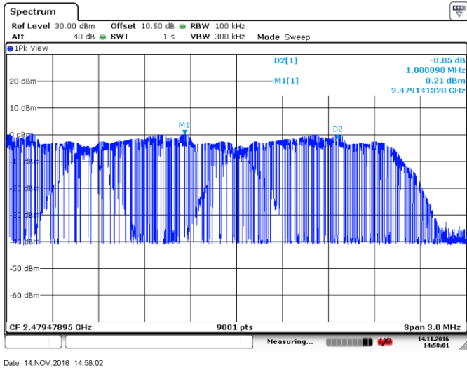
Figure 8.2-12: Carrier frequency separation Modulation 3
