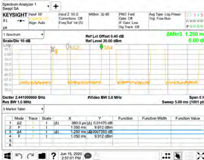
Dwell Time_GFSK_1M_DH1_2441MHz
