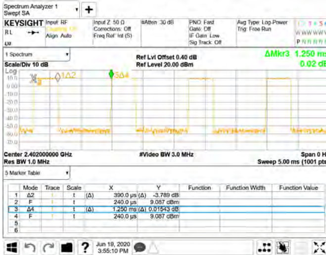
Dwell Time_8DPSK_3M_DH1_2402MHz
