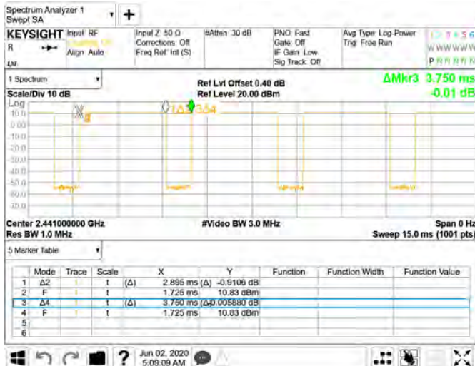
Dwell Time_GFSK_1M_DH5_2441MHz
