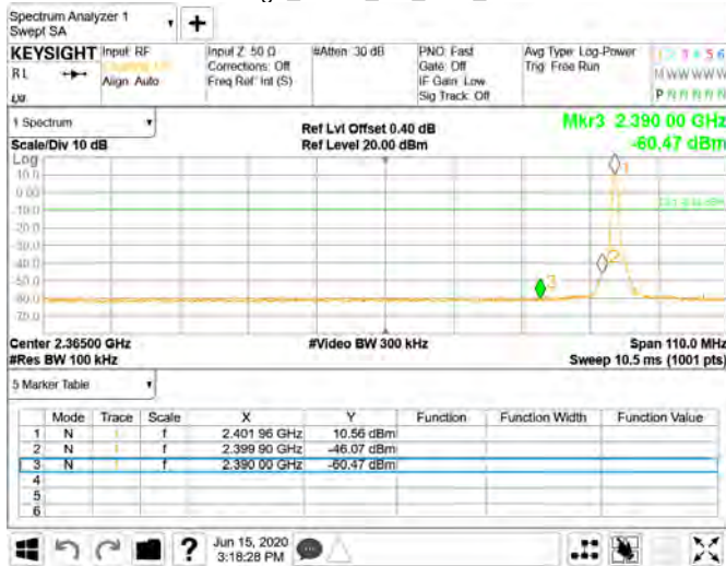
Band Edge_GFSK_1M_DH5_2402MHz
