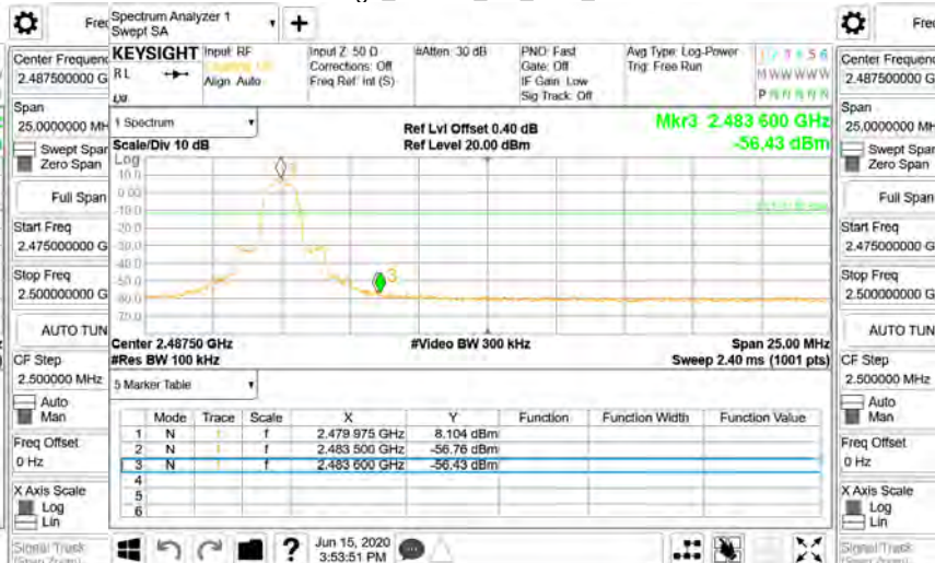
Band Edge_8DPSK_3M_DH5_2480MHz
