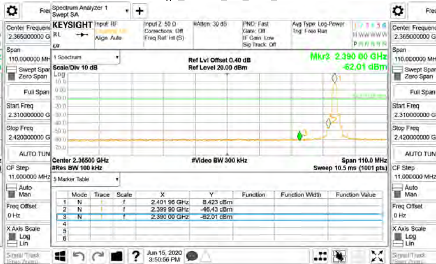
Band Edge_8DPSK_3M_DH5_2402MHz
