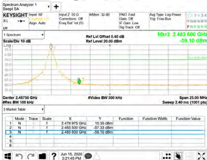
Band Edge_GFSK_1M_DH5_2480MHz
