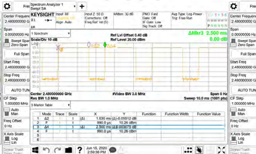
Dwell Time_GFSK_1M_DH3_2480MHz
