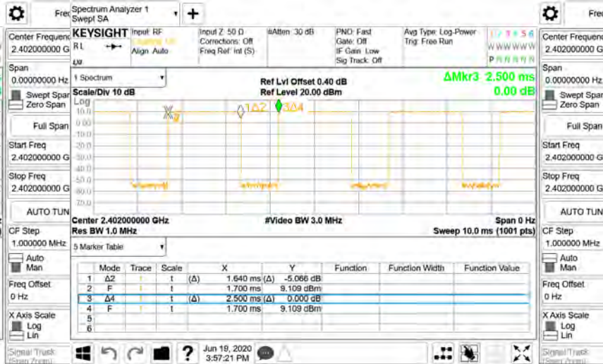
Dwell Time_8DPSK_3M_DH3_2402MHz
