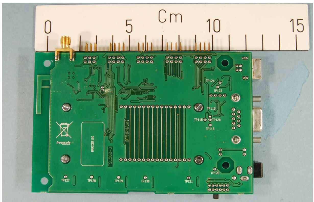
13213-NCB - rear view
