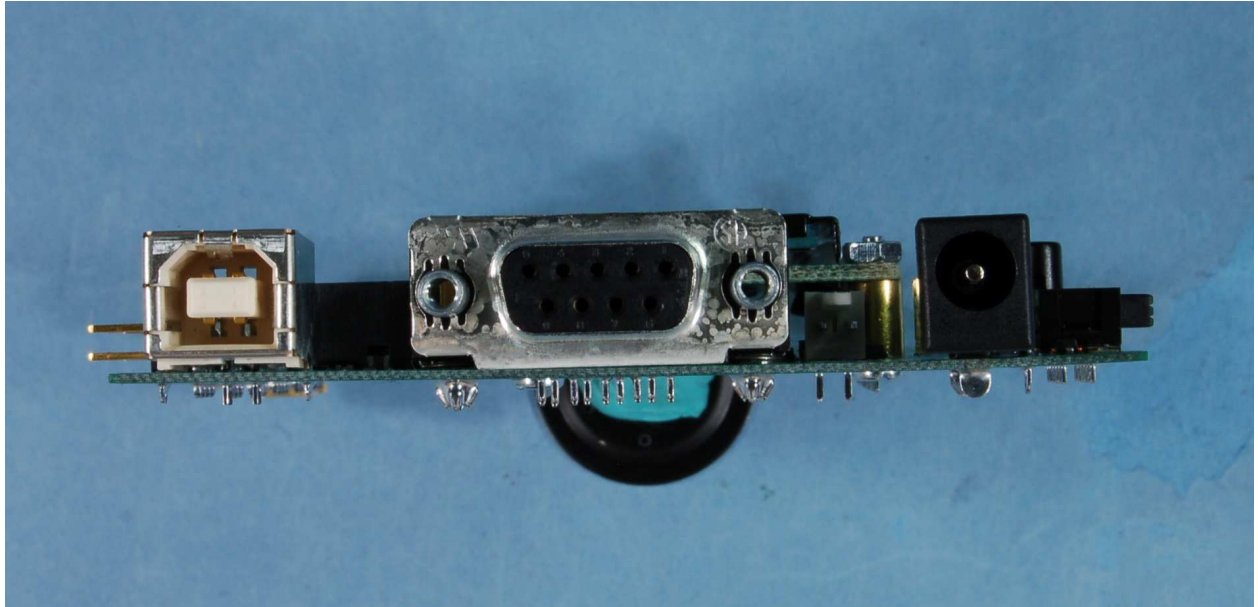
13213-NCB view of USB, RS232 DC adapter ports
