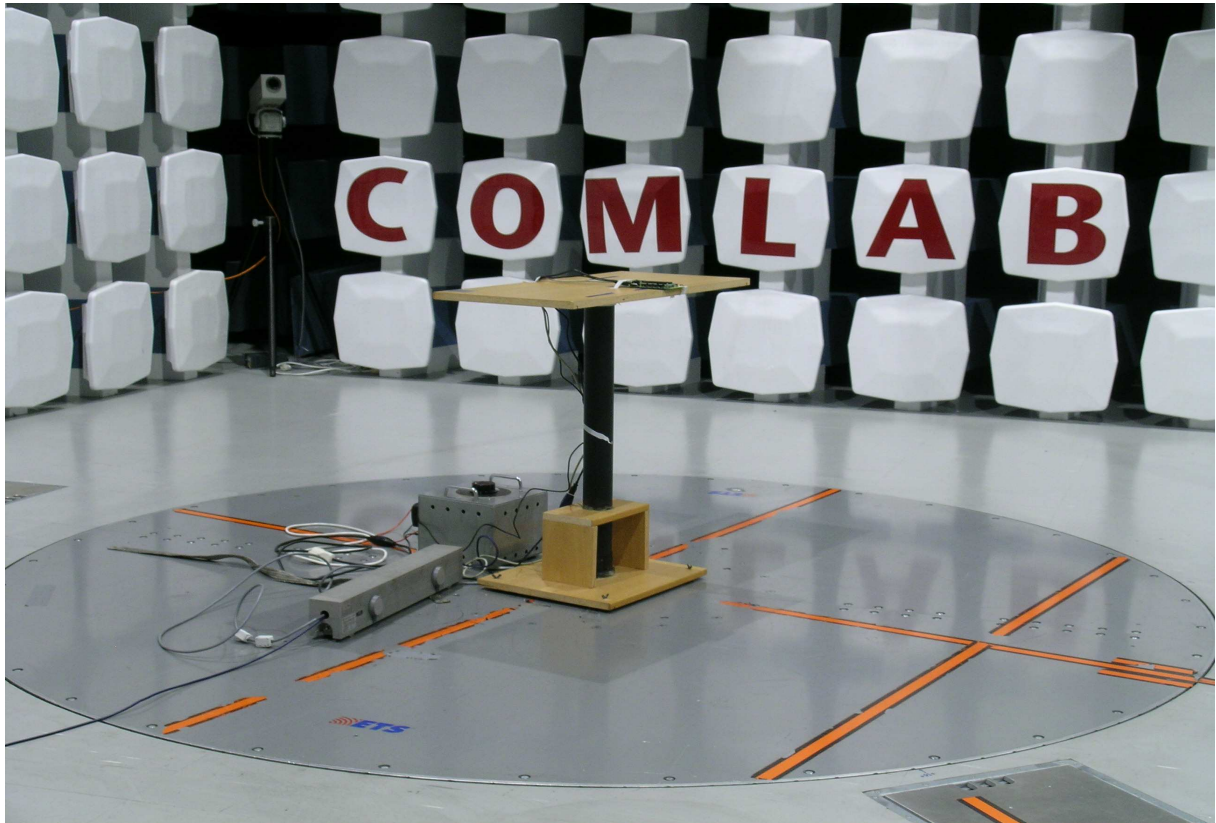
13213-NCB - Radiated emission with integral antenna 9 kHz – 25 GHz
