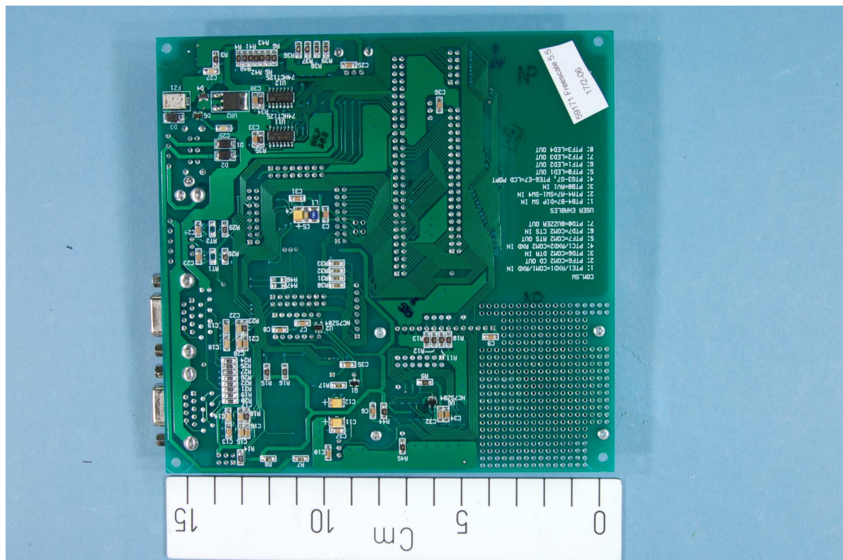
Fig 6 - M68EVB908GB60 – Microcontroller board –Rear view
