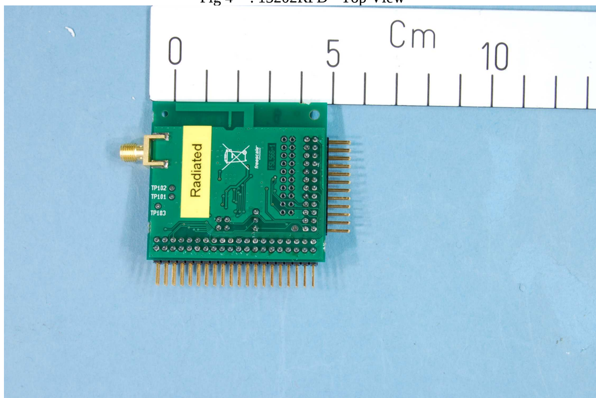
Fig 4 - . 13202RFD- Top View
