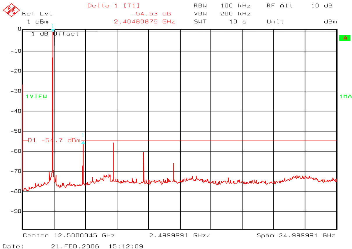
Fig. 11– 13202RFD - Ch11 – Conducted Spurious – 9kHz – 25GHz
