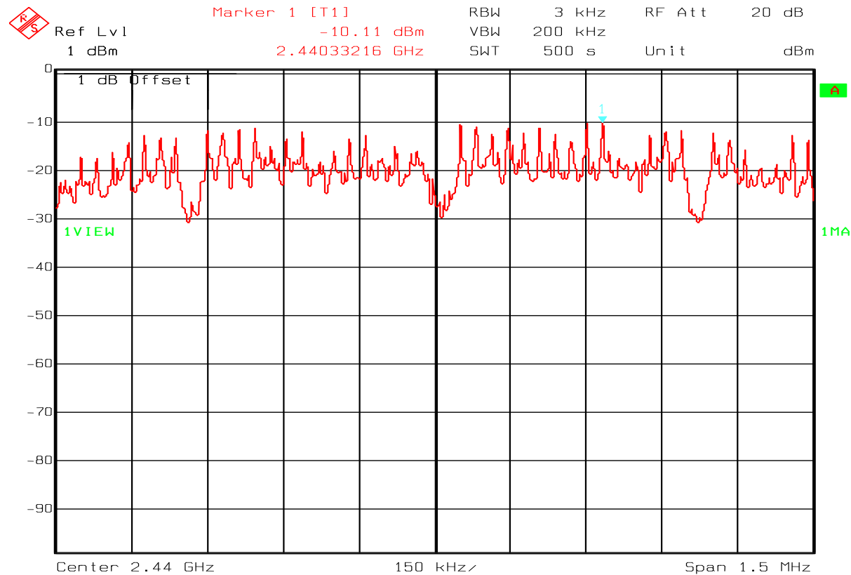
Fig 24- 13202RFD- Ch11 – Power Density – Conducted measurement
