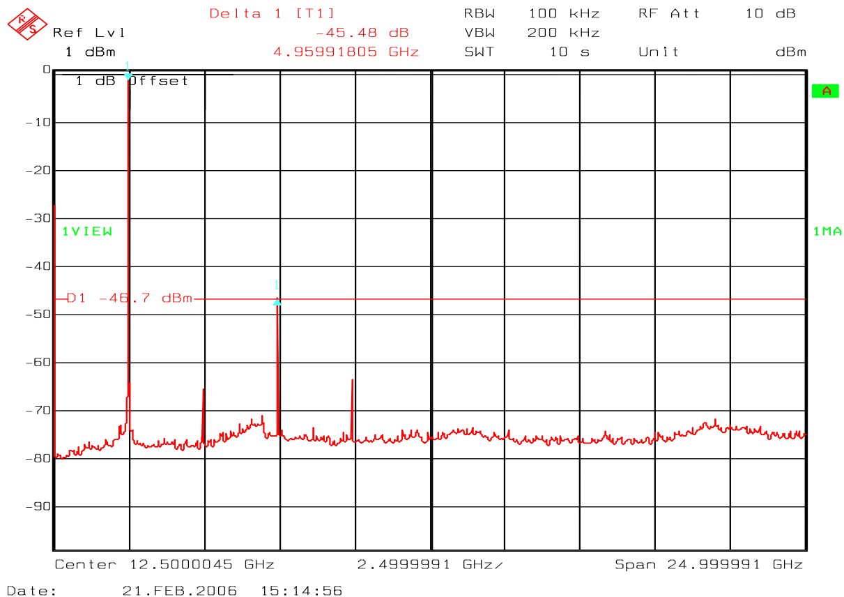
Fig. 13 – 13202RFD - Ch26 – Conducted Spurious – 9kHz – 25GHz
