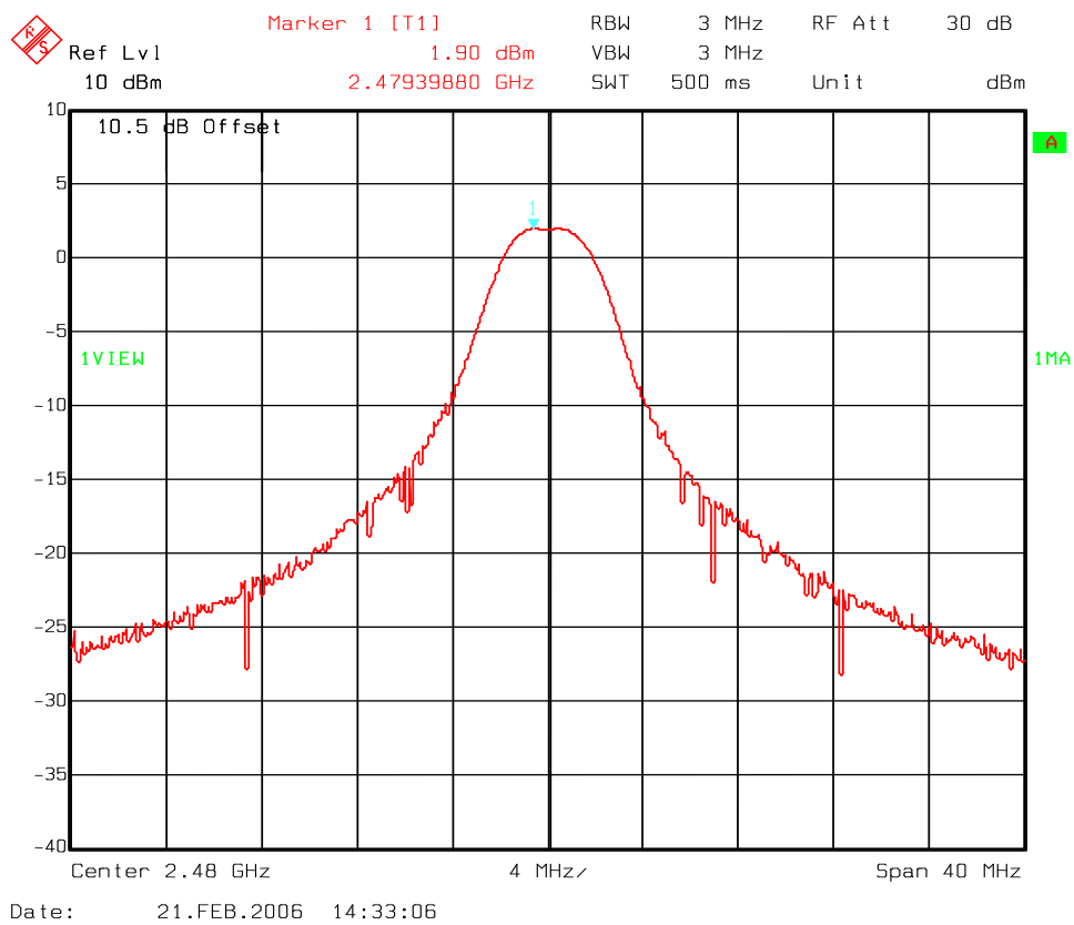
Fig 8 – 13202RFD – Ch26 – Conducted Peak Output Power
