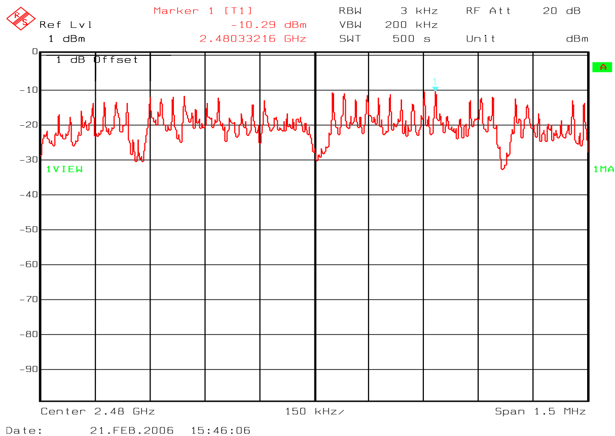
Fig 26- 13202RFD – Ch26 – Power Density – Conducted measurement
