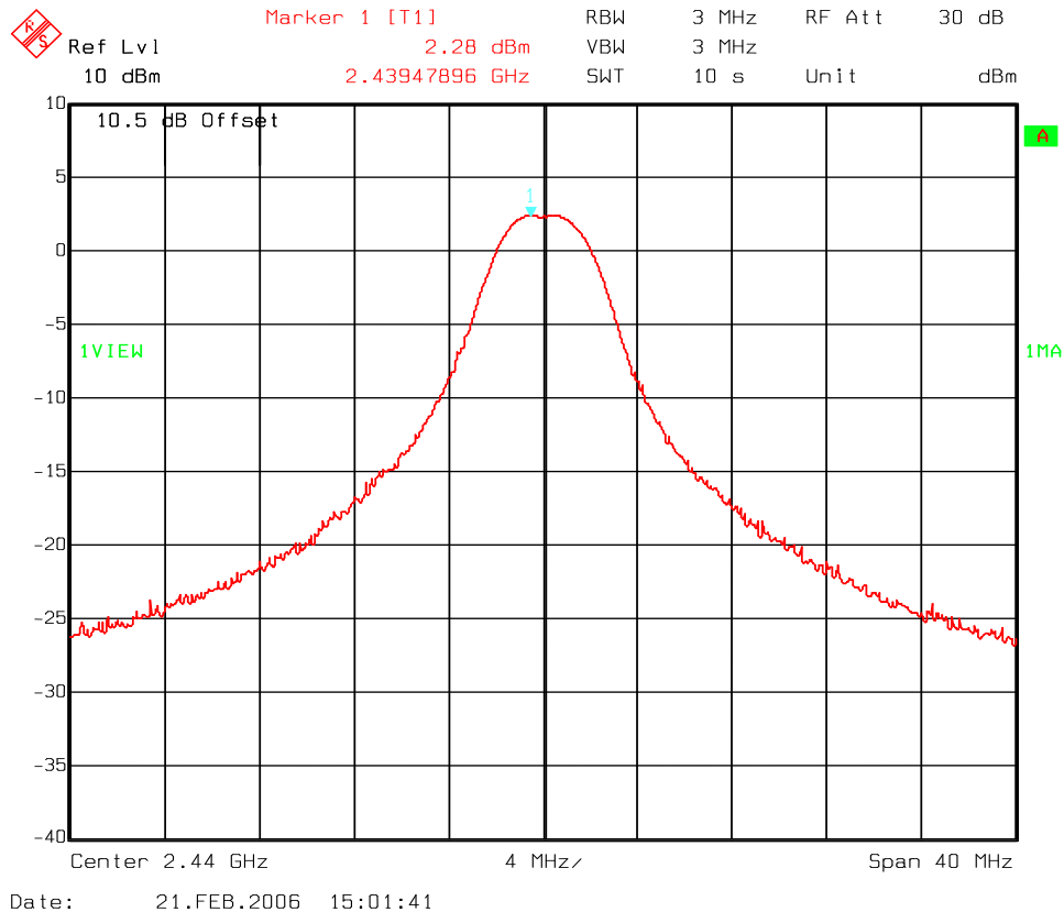
Fig 7– 13202RFD – Ch18 – Conducted Peak Output Power
