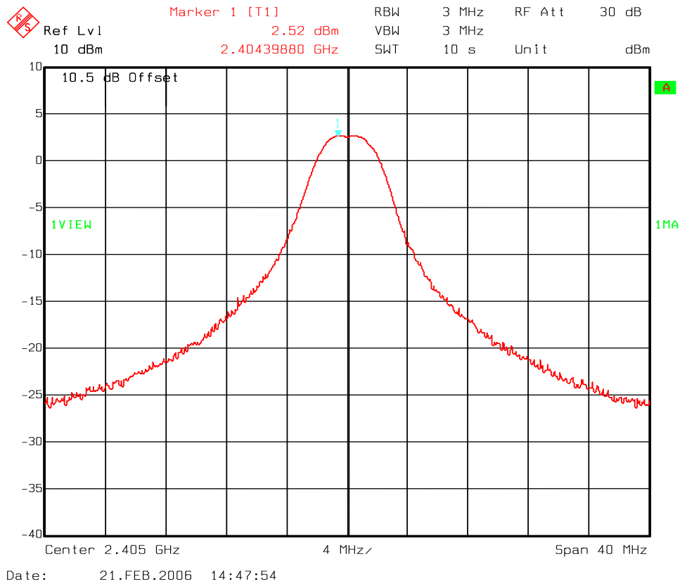
Fig 6 – 13202RFD – Ch11 – Conducted Peak Output Power
