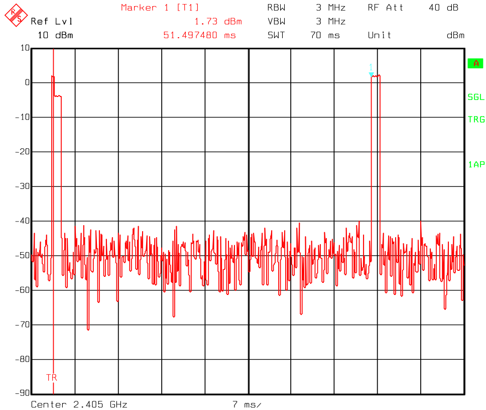
Fig 14 – 13202RFD – Duty Cycle – ON-time
