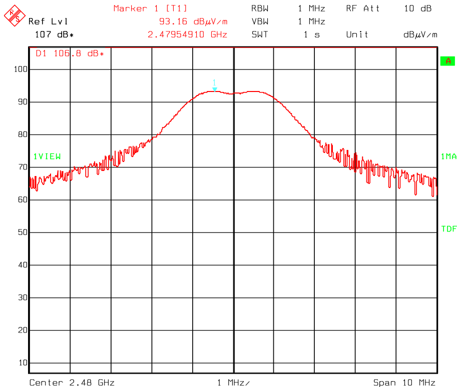
Fig. 9 –13202RFD - Ch26 – upper-band –field strength
