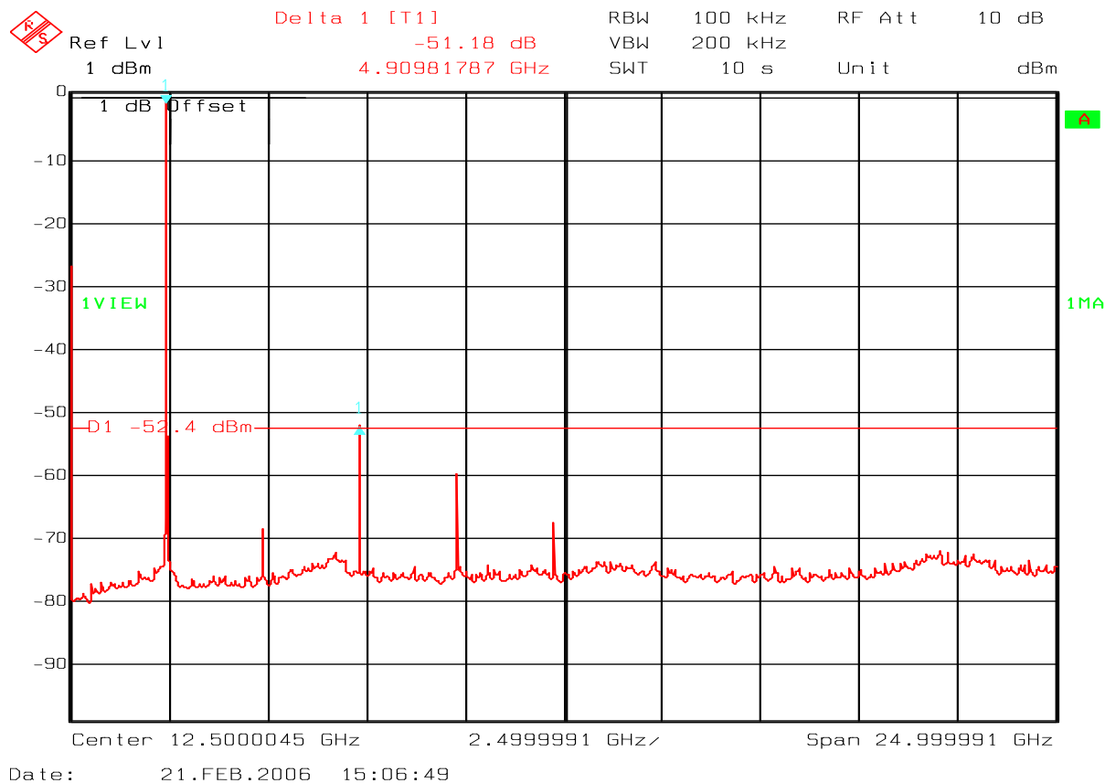
Fig. 12 –13202RFD- Ch18 – Conducted Spurious – 9kHz – 25GHz
