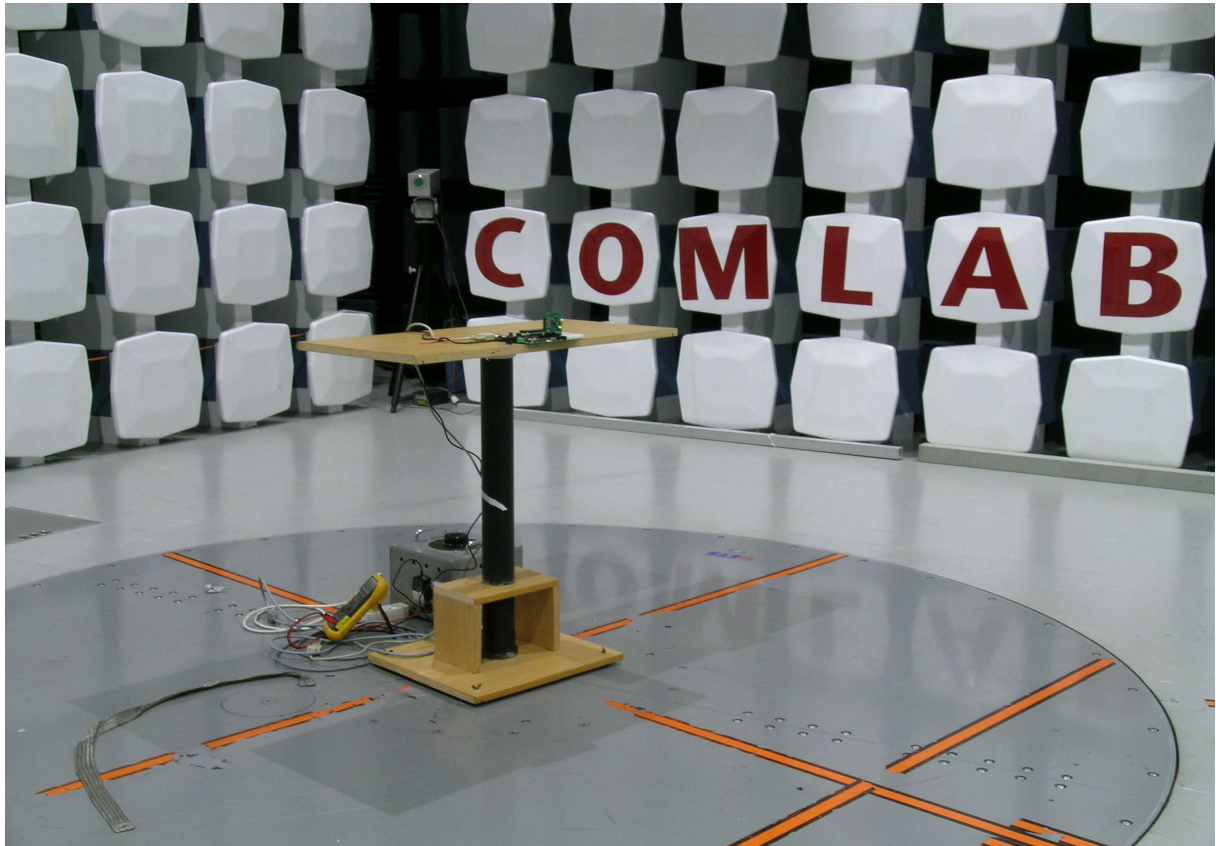
13202-RFD - Radiated emission 9 kHz – 25 GHz
