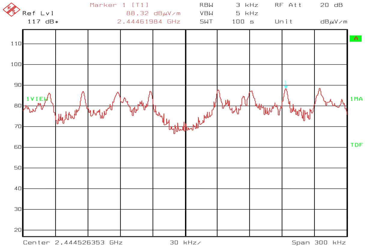
Ch11 Peak level for PSD
