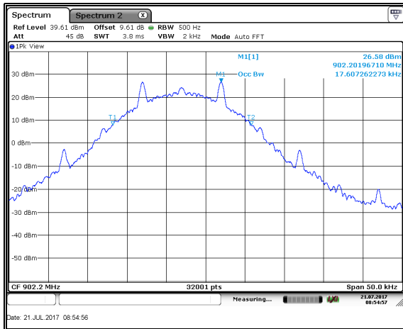
Figure 7.4.3.2-4: 99% BW Low Ch – FSK – 10kbps
