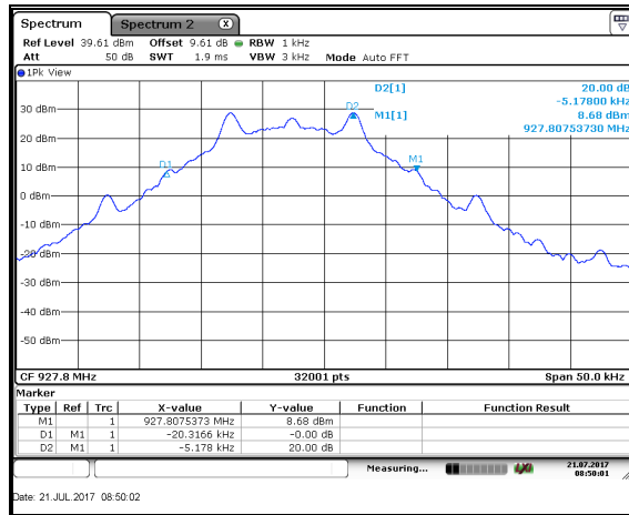
Figure 7.3.4.2-3: 20dB BW High Ch – FSK – 10kbps
