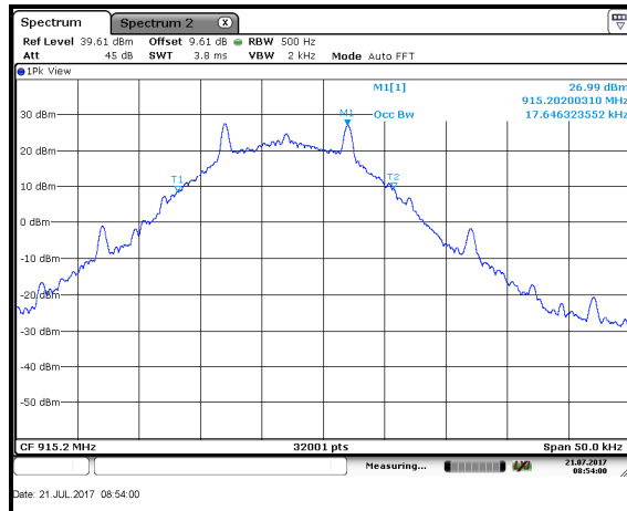
Figure 7.3.4.2-5: 99% BW Mid Ch – FSK – 10kbps
