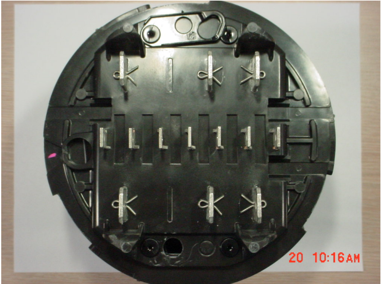
Figure 2: Rear View
