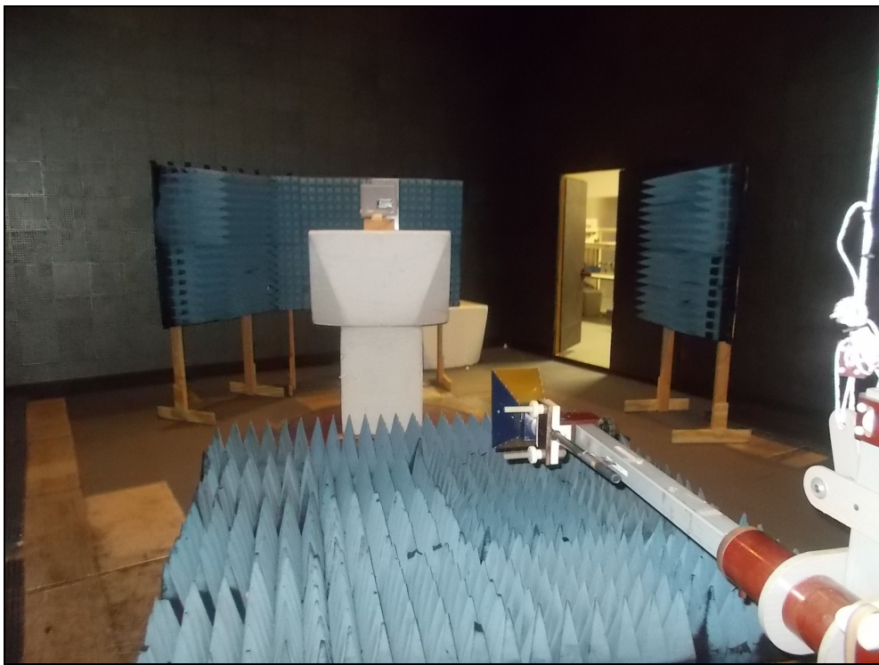
Figure 1: Test Setup – Front View
